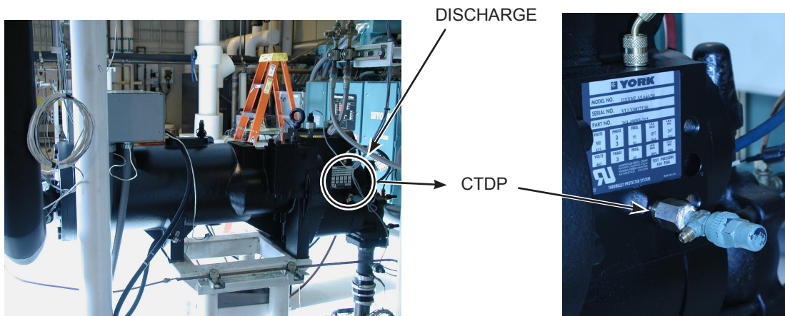
FIGURE 2 - SUCTION
