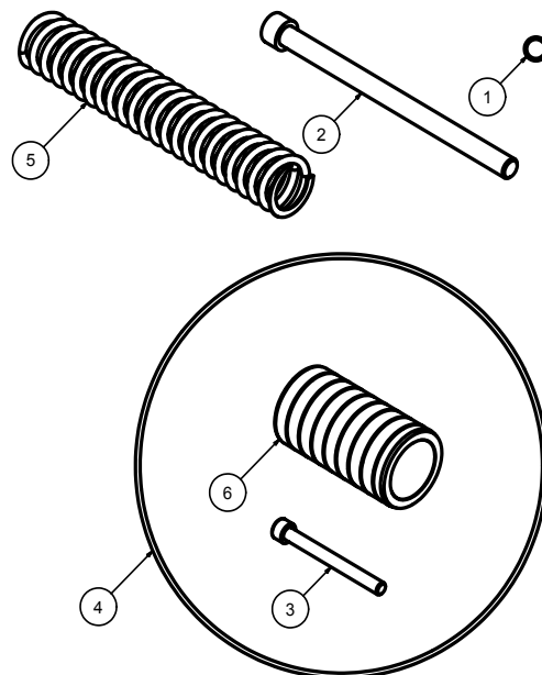
FIGURE 1 - SLIDE VALVE RETURN SPRING KIT
