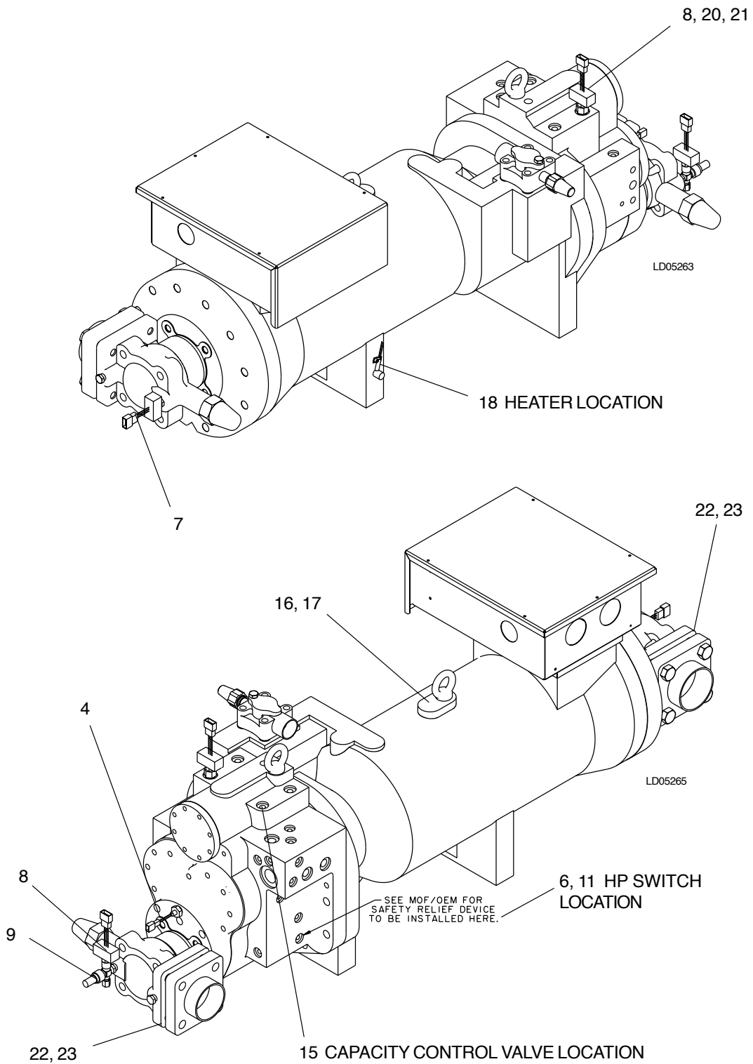
FIG. 12 – DXS COMPRESSOR OUTLINE (REF. TABLES 8 AND 9, PAGE 25)
