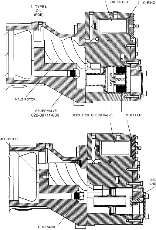
FIG. 11 – COMPRESSOR FILTER AND MUFFLER
