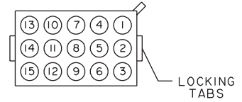
HOUSING - CONNECTOR (J4) WIRING END
