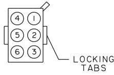
HOUSING - CONNECTOR (J1, J2, J5, & J6) WIRING END
