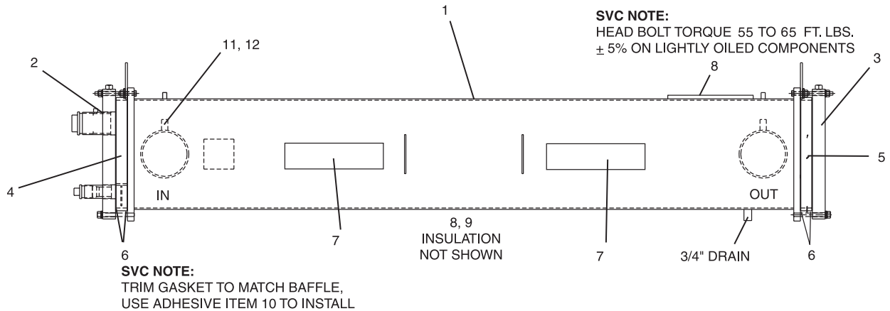
FIG. 1 – EVAPORATOR COMPONENTS
