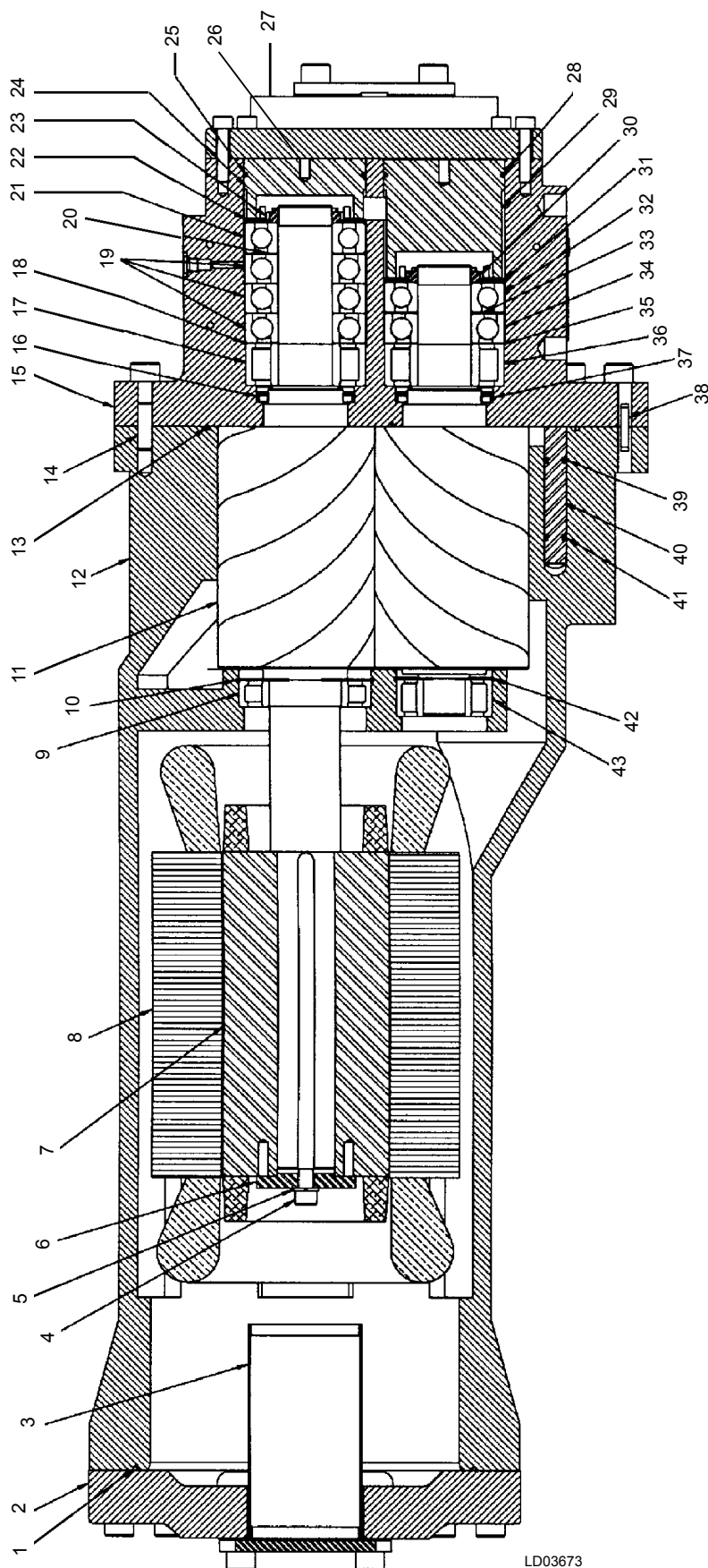
FIG. 43 – COMPRESSOR COMPONENTS
