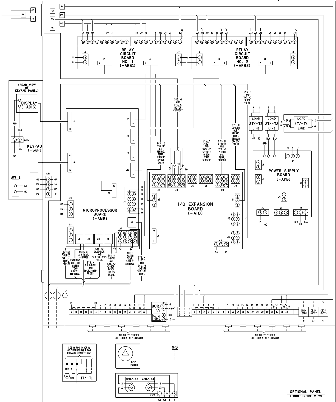
FIG. 22B – POWER PANEL COMPONENT LOCATION
