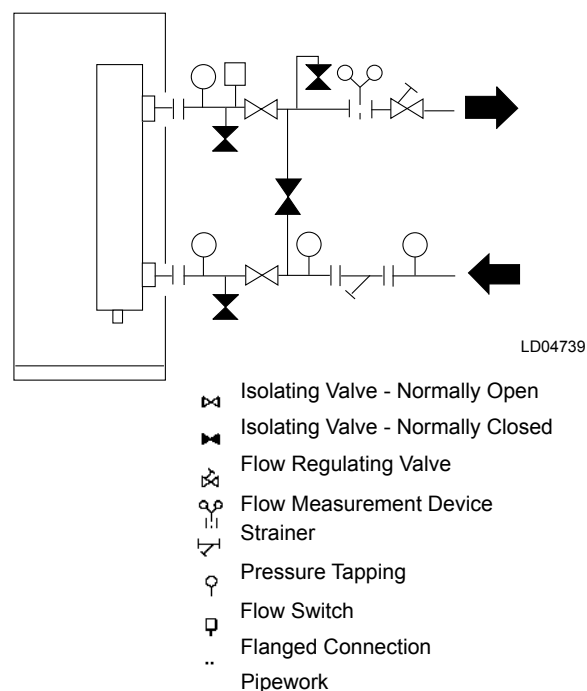
FIG. 5 – PIPEWORK ARRANGEMENT
