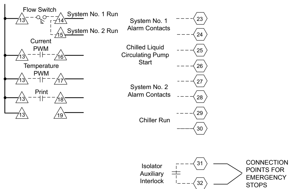
FIG. 12 – CUSTOMER CONNECTIONS
