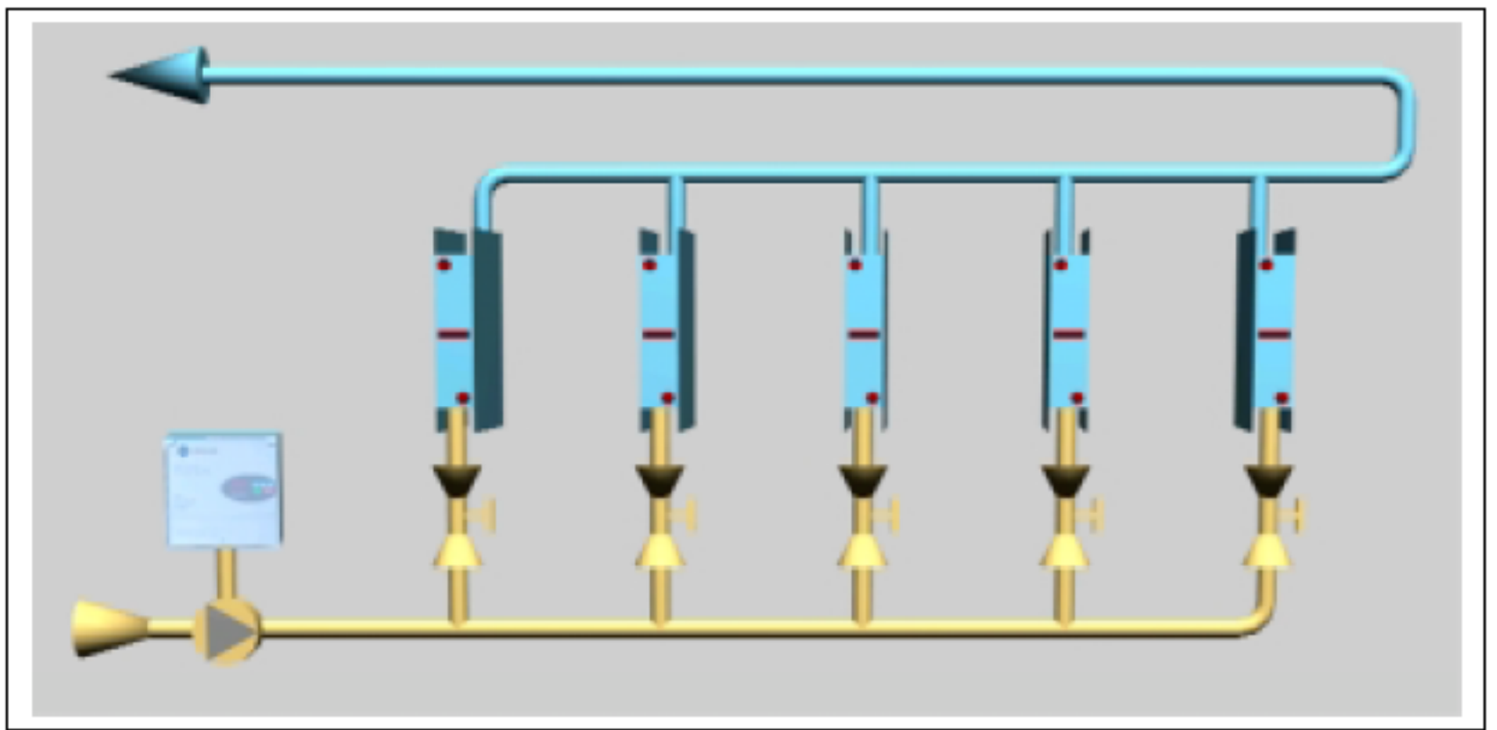
Figure 6 - Reverse Return Piping
