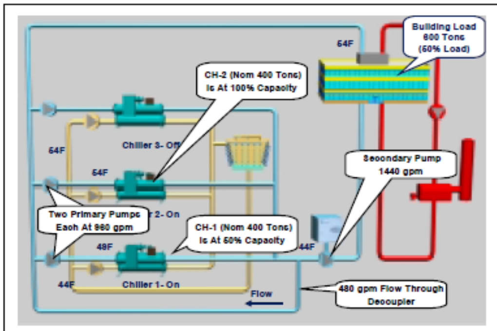
Figure 49 - Backloaded Primary Loop Layout
