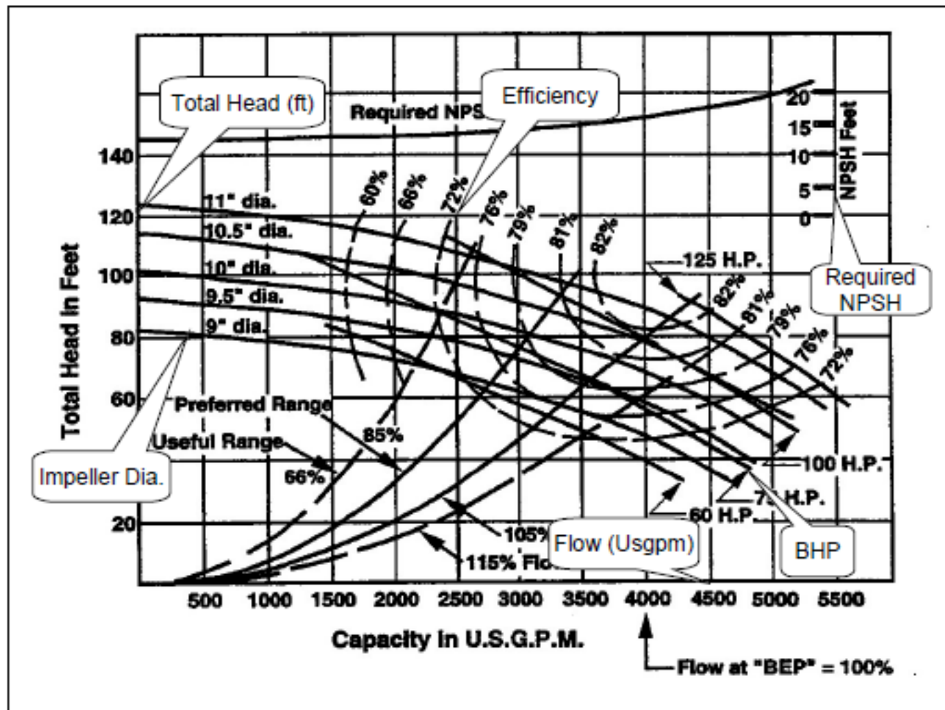
Figure 11 - Typical Centrifugal Pump Curve
