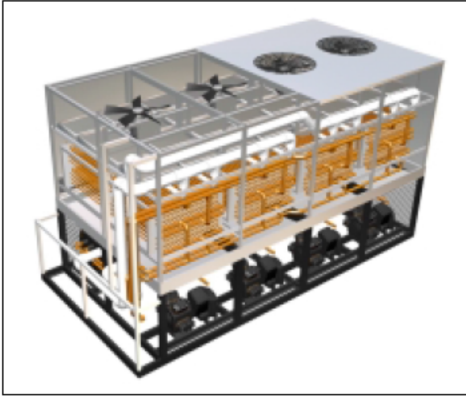
Figure 29 - McQuay EGR Evaporatively Cooled Chiller
