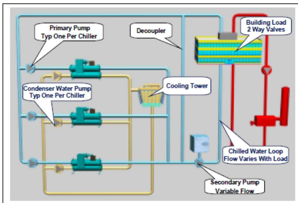
Figure 43 - Typical Primary/Secondary System
