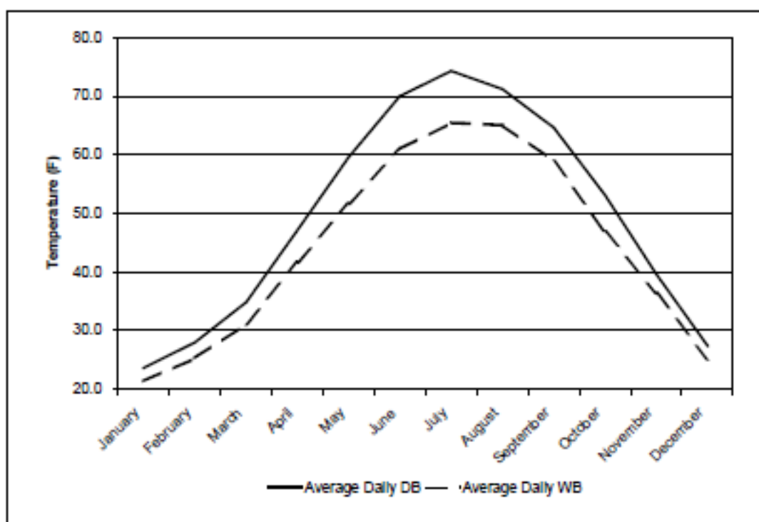
Figure 28 - Annual Ambient Drybulb Vs. Wetbulb
