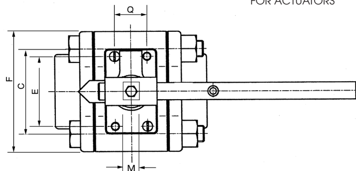
1/4" - 4" STEM ARRANGEMENT FOR ACTUATORS
