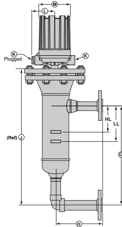
Figure 16 Flanged Side/Side
