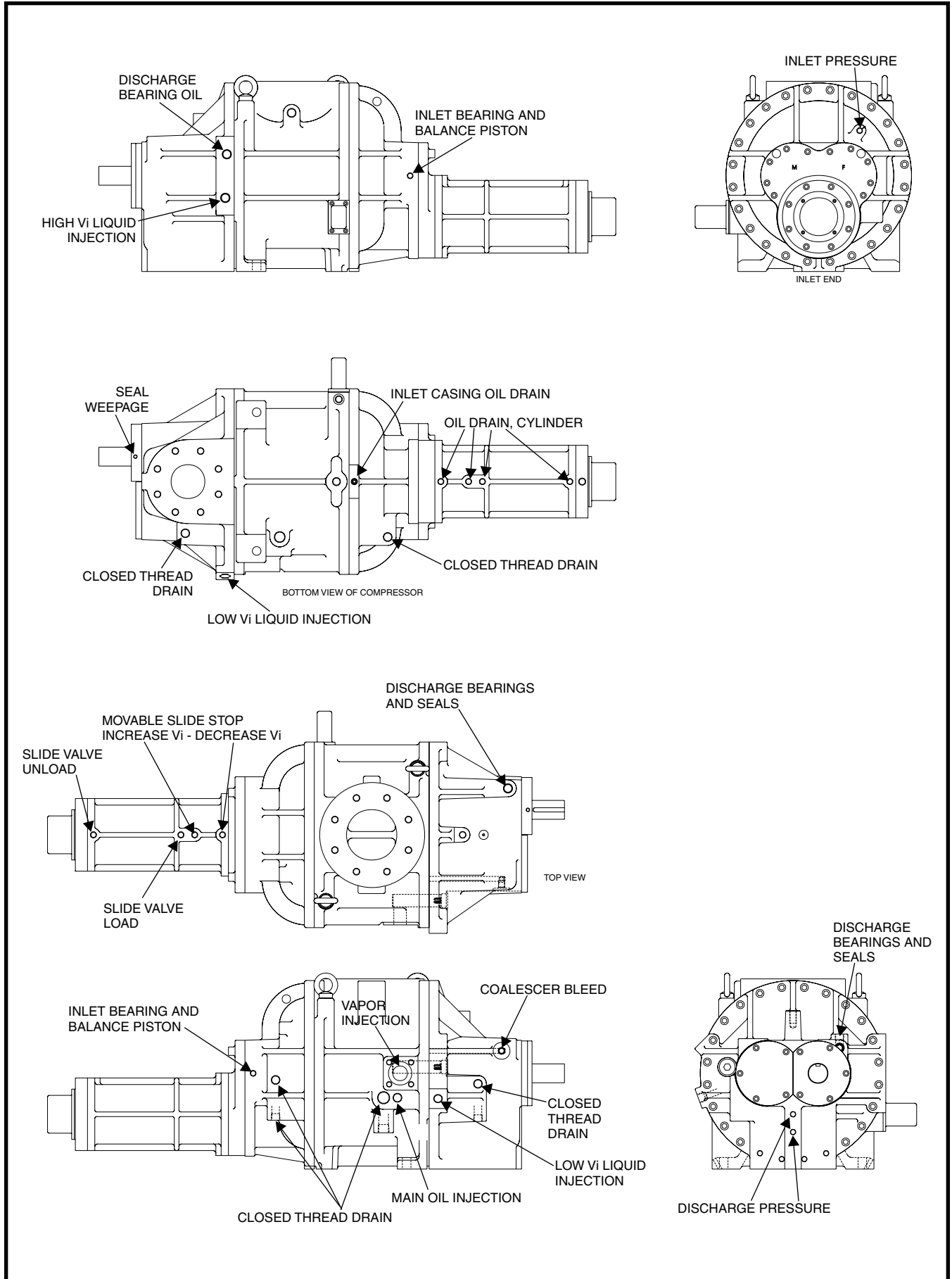
Figure 31. 163/193mm Compressor Ports Locations
