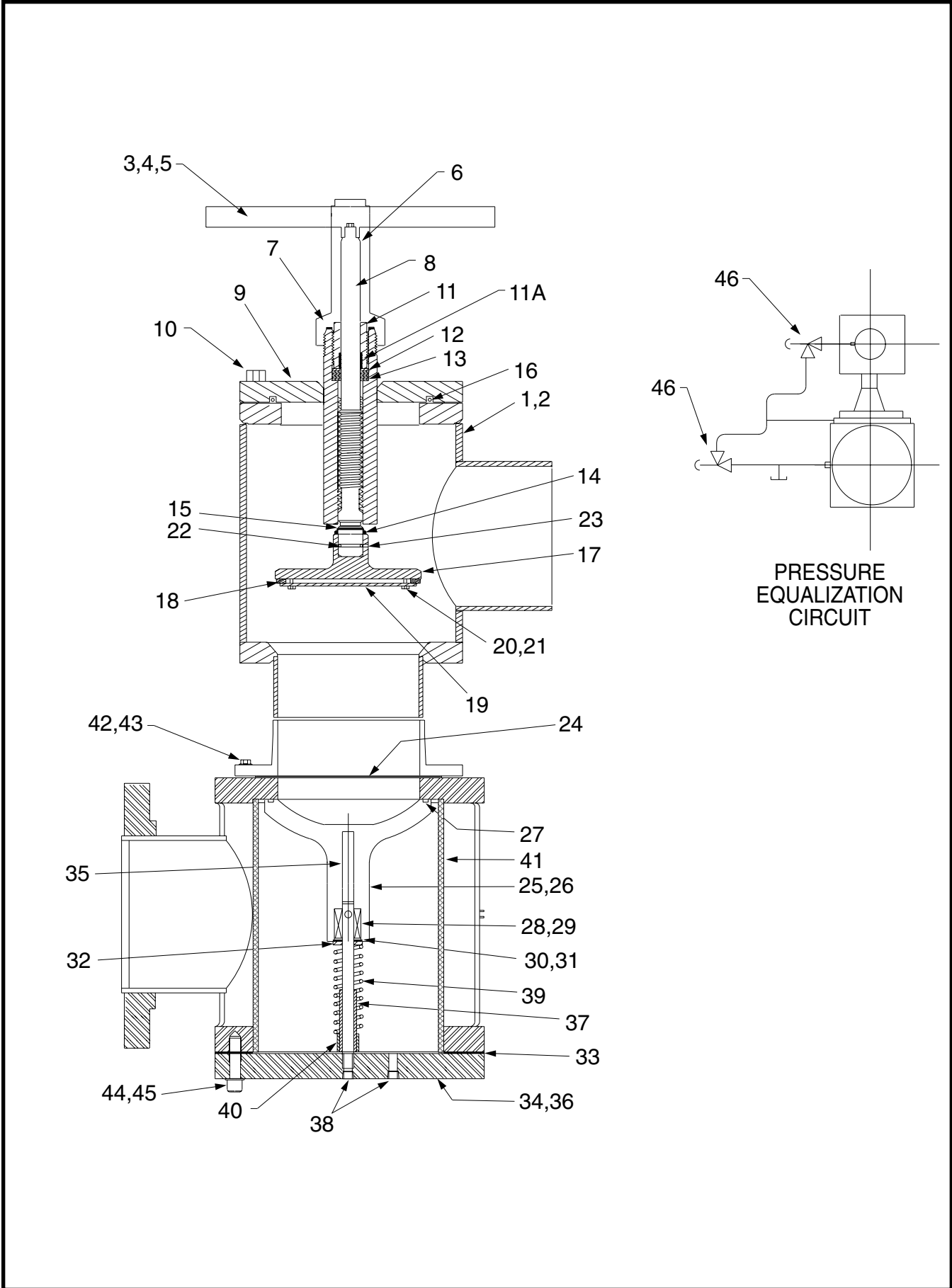
Figure 17. 10" and 14" Multivalve, Frick®
