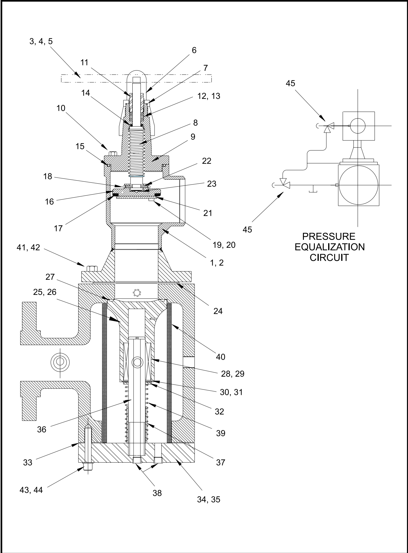
Figure 16. 5"—8" Multivalve, Frick®
