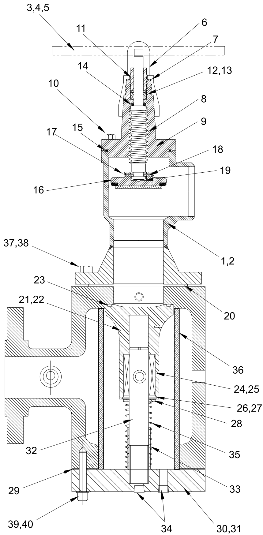
Figure 15. 4" Multivalve, Frick®
