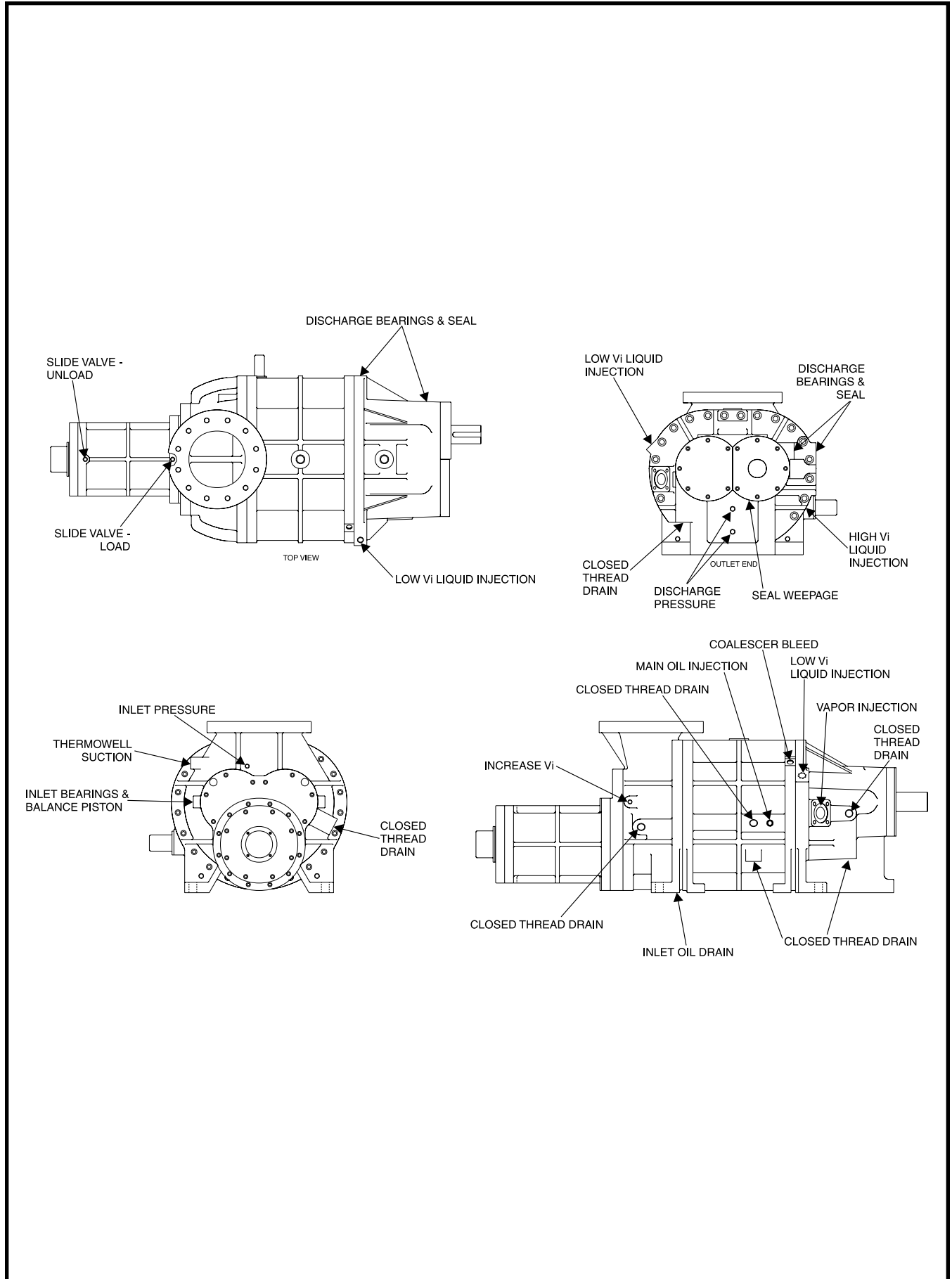
Figure 33. 283mm Compressor Ports Locations
