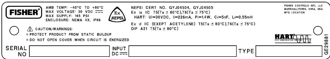
TYPE DVC6010, DVC6020, AND DVC6030
