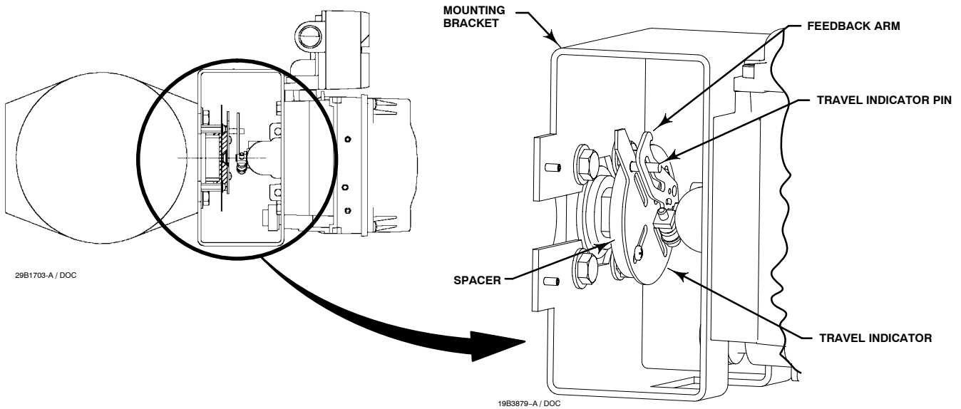
Figure 2-5. Mounting a DVC6030 Digital Valve Controller on a Rotary Actuator (Type 1032 Size 425A Shown)
