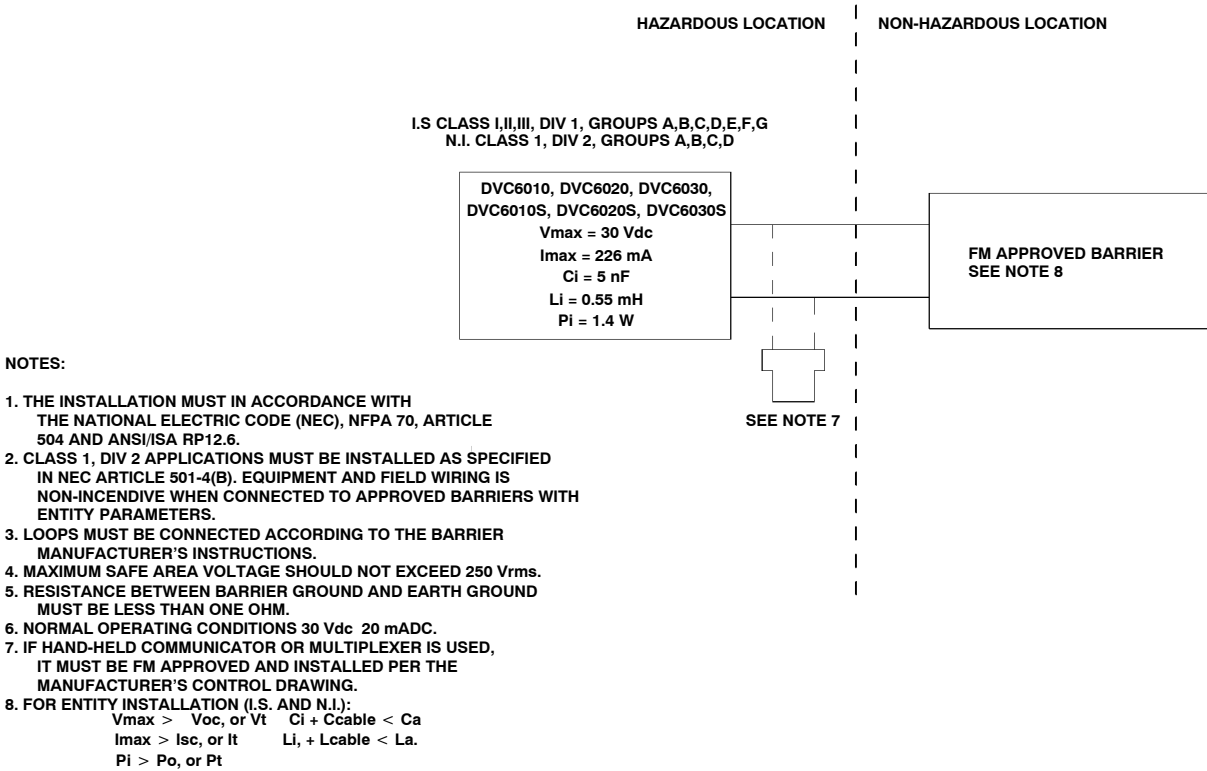
Figure 5-3. FM Schematic for Type DVC6000 and DVC6000S
