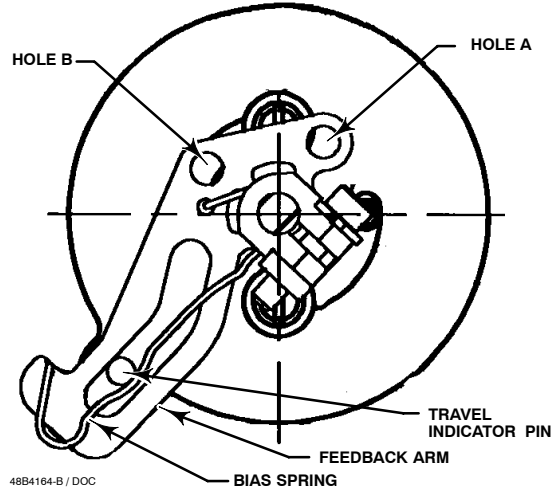
Figure 2-8. Positioning Travel Indicator Pin in the Feedback Arm (Viewed as if Looking from the DVC6030 toward the Actuator)
