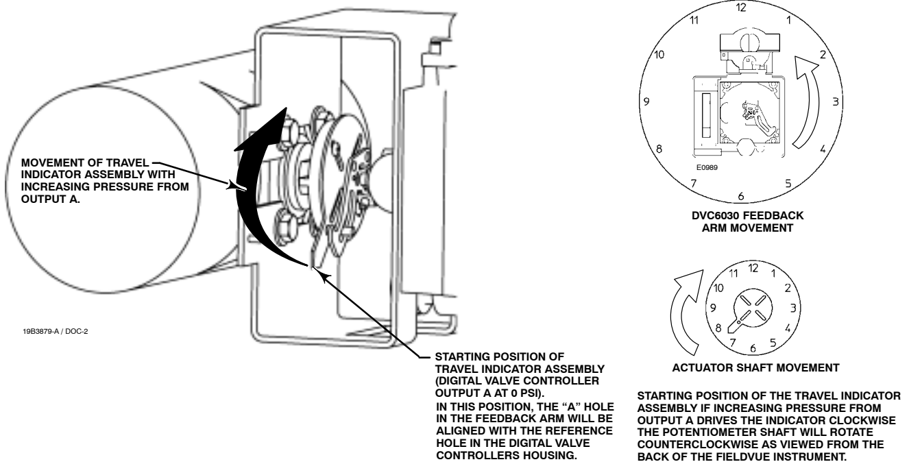
Figure 2-7. Explanation of Travel Indicator Starting Position and Movement if Counterclockwise Orientation is Selected for "Travel Sensor Motion" in AMS™ ValveLink® Software or the 375 Field Communicator
