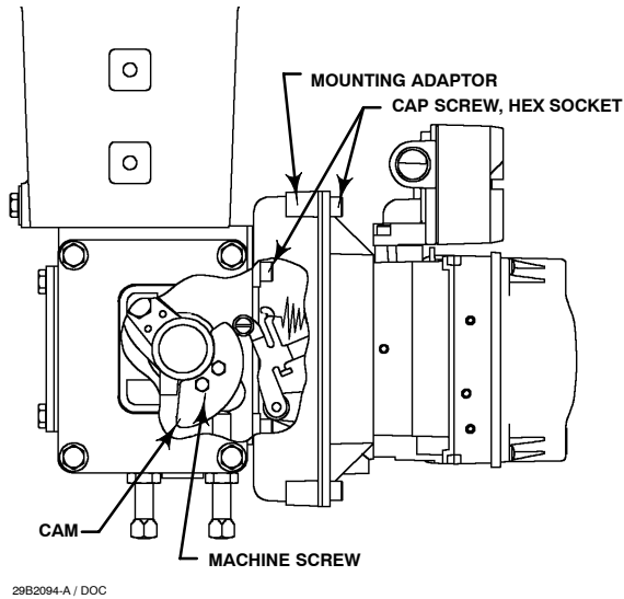
TYPICAL MOUNTING WITH SHORT FEEDBACK ARM (FISHER TYPE 1052 SIZE 33 ACTUATOR SHOWN)
