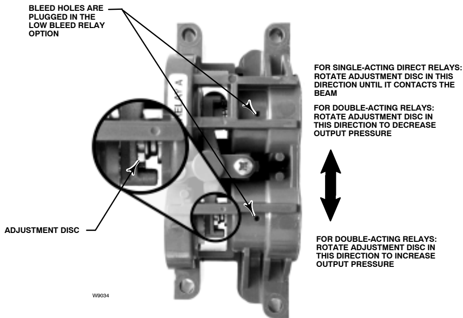
Figure 3-4. Relay A Adjustment (Shroud Removed for Clarity)
