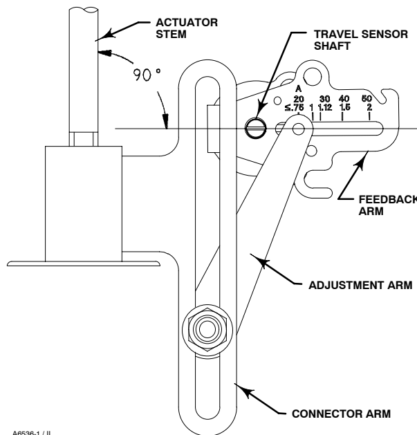
Figure 3-5. Crossover Point
