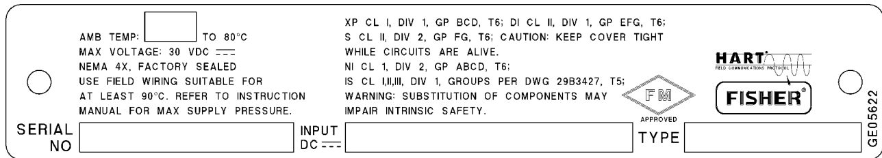
Figure 5-4. FM Nameplate
