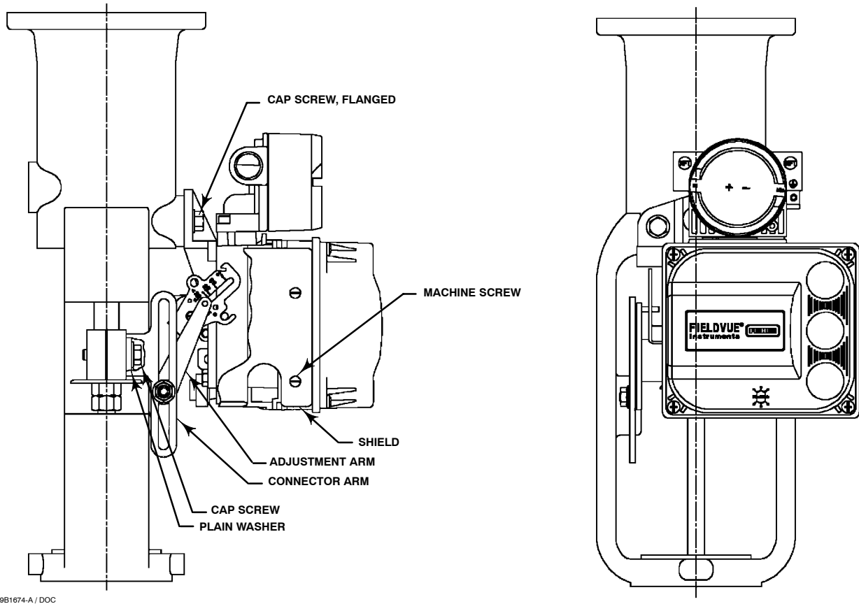
Figure 2-1. DVC6010 Digital Valve Controller Mounted on Sliding-Stem Actuators with up to 2 Inches Travel
