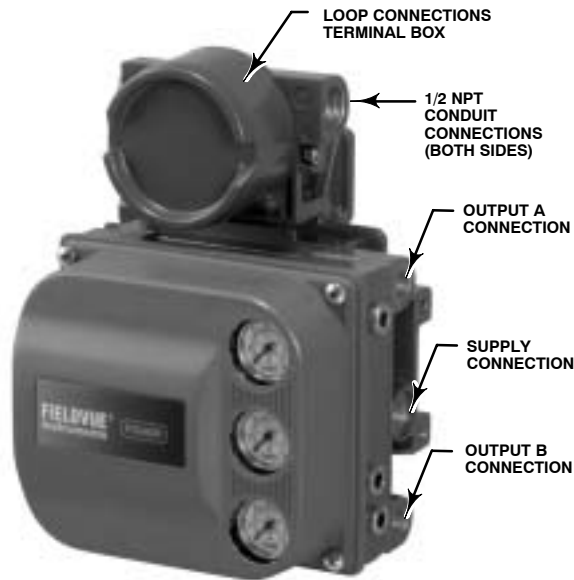
VALVE-MOUNTED INSTRUMENT
