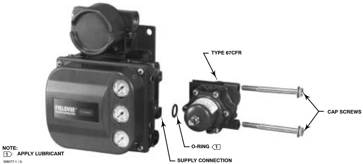
Figure 2-9. Mounting the Type 67CFR Regulator on a DVC6000 Series Digital Valve Controller
