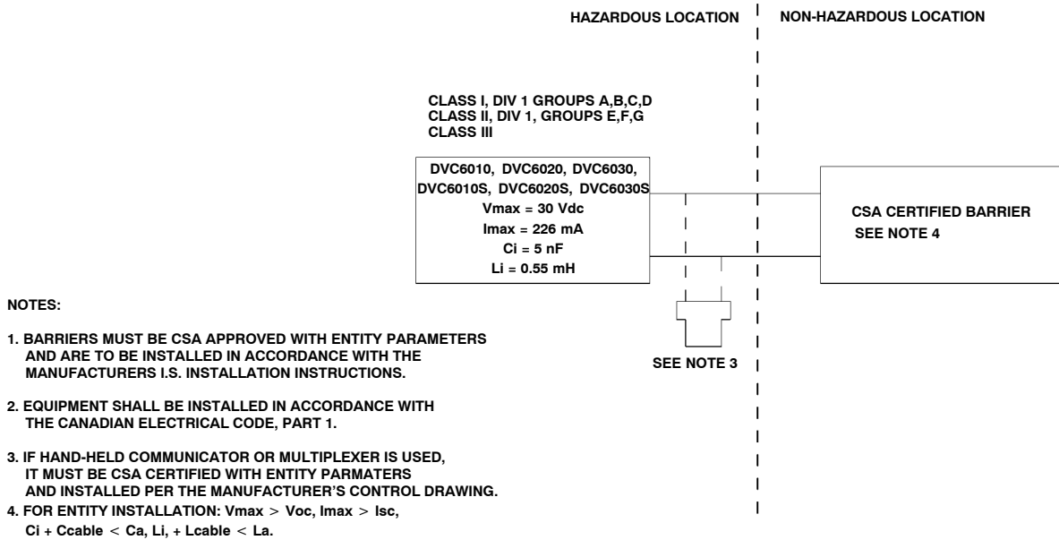
Figure 5-1. CSA Schematic for Type DVC6000 and DVC6000S
