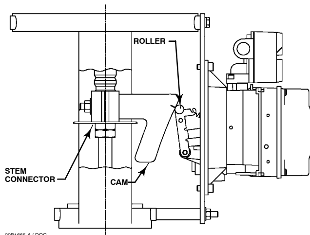
Figure 3-3. Feedback Connection for Typical Long-Stroke Sliding-Stem Actuator (4 to 24-inches travel)
