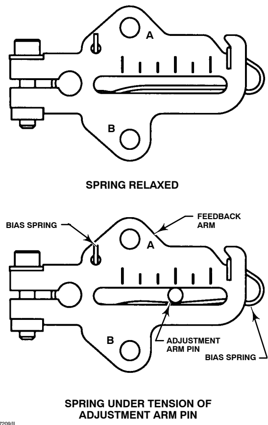
Figure 2-3. Locating Adjustment Arm Pin in Feedback Arm
