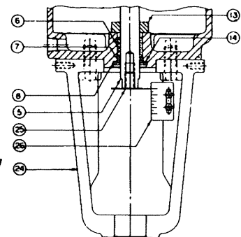
Figure 6 GB52/53/54UC GB52/53/54UW
