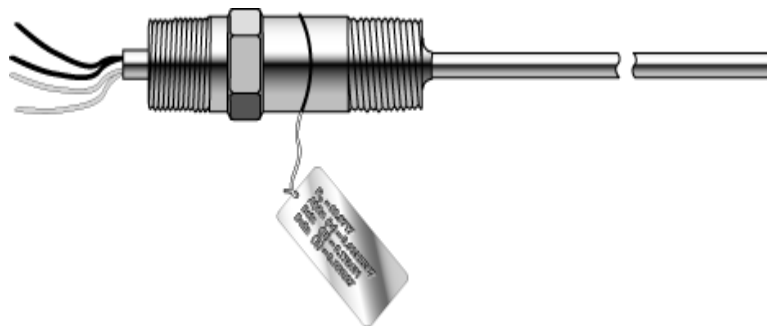
FIGURE 13. Typical Sensor Ordered with Option Code V
