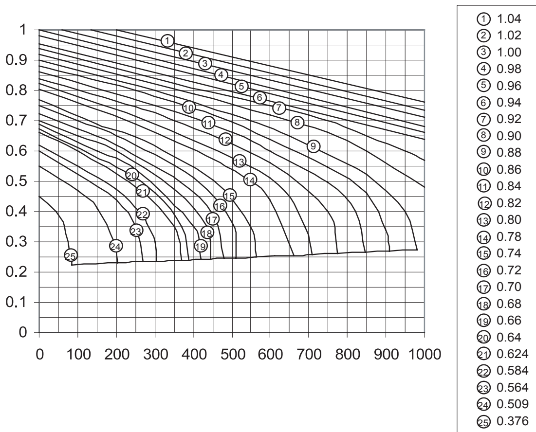
Figure A-3. Specific Gravity – Temperature Relationship for Petroleum Oils Reprinted with permission from the Oil and Gas Journal
