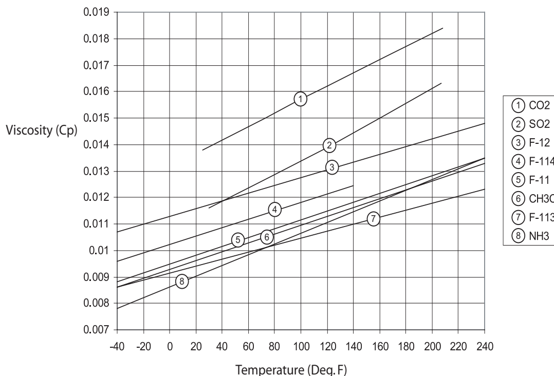
Figure A-6. Viscosity of Refrigerant Vapors (saturated and superheated vapors)
