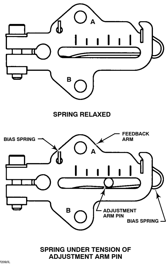
Figure 2-3. Locating Adjustment Arm Pin in Feedback Arm
