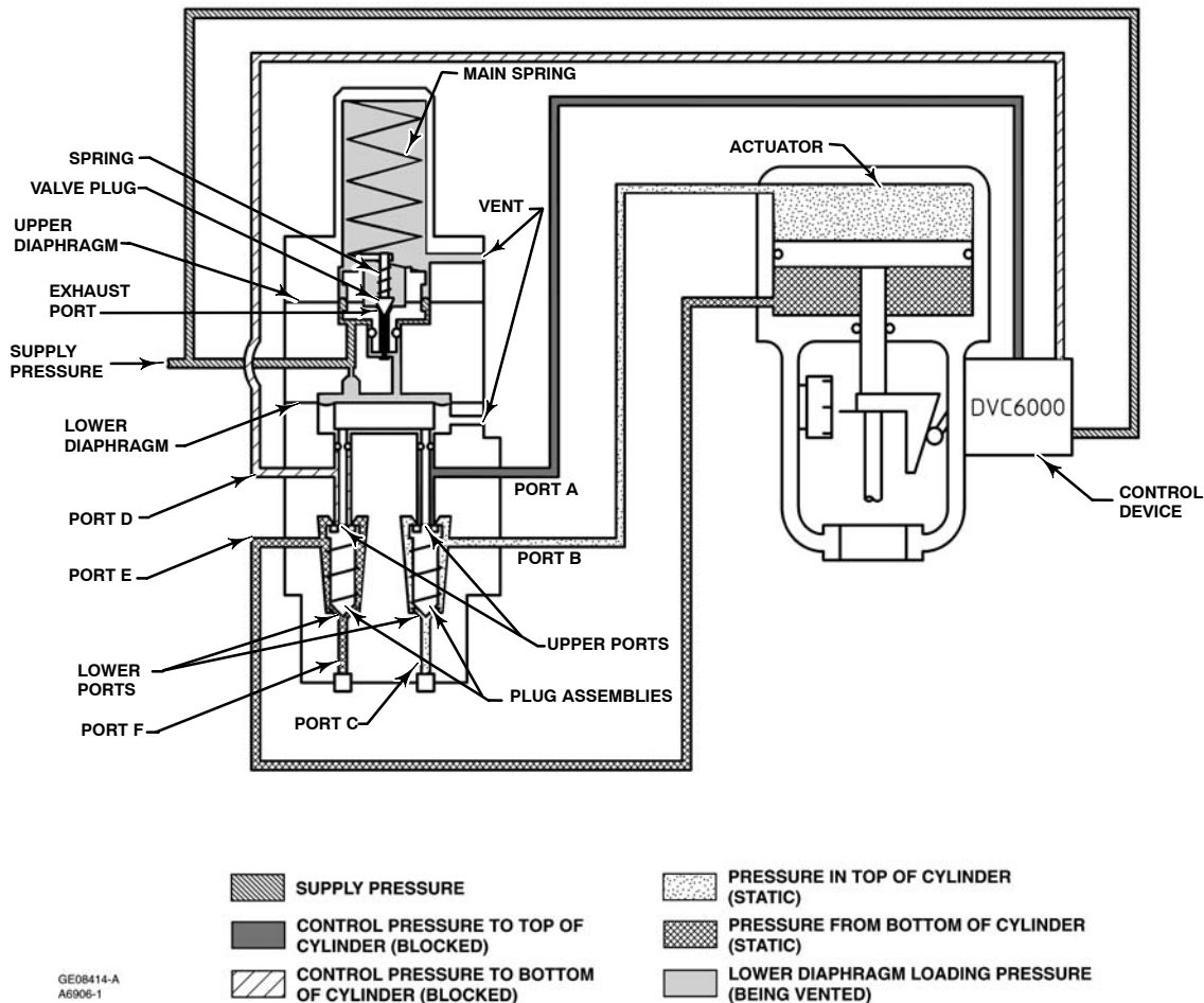
Figure 6. Type 377L Trip Valve Shown Tripped
