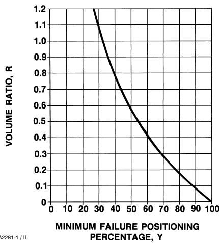
Figure 8. Volume Tank Sizing Graph
