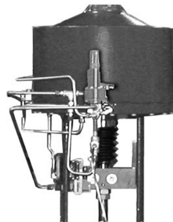
Figure 2. Type 377 Trip Valve Mounted on Size 130 Type 585C Actuator
