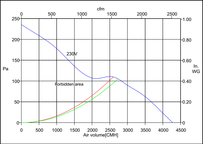
208/280-3-60 Power Exhaust Fan Curve
