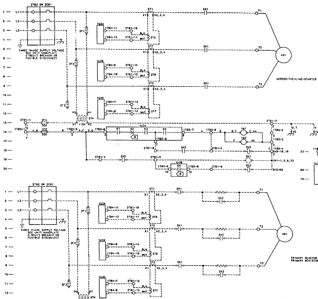
Figure 17 Available Starter Configurations
