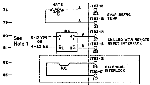
Figure 22 Remote Generic BAS/CWR Interface Option
