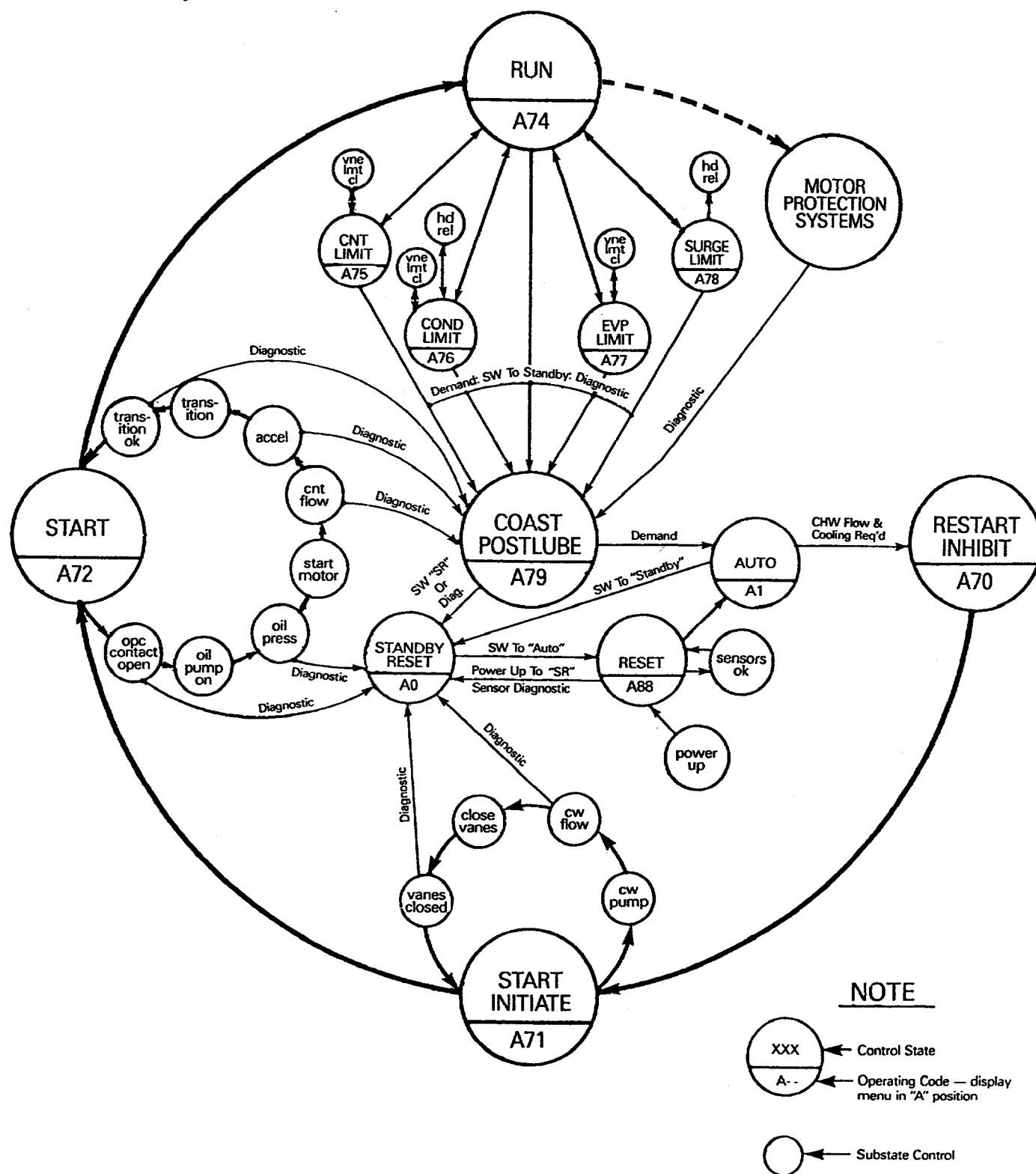
Figure 23 UCP Start-Run-Shutdown Sequence
