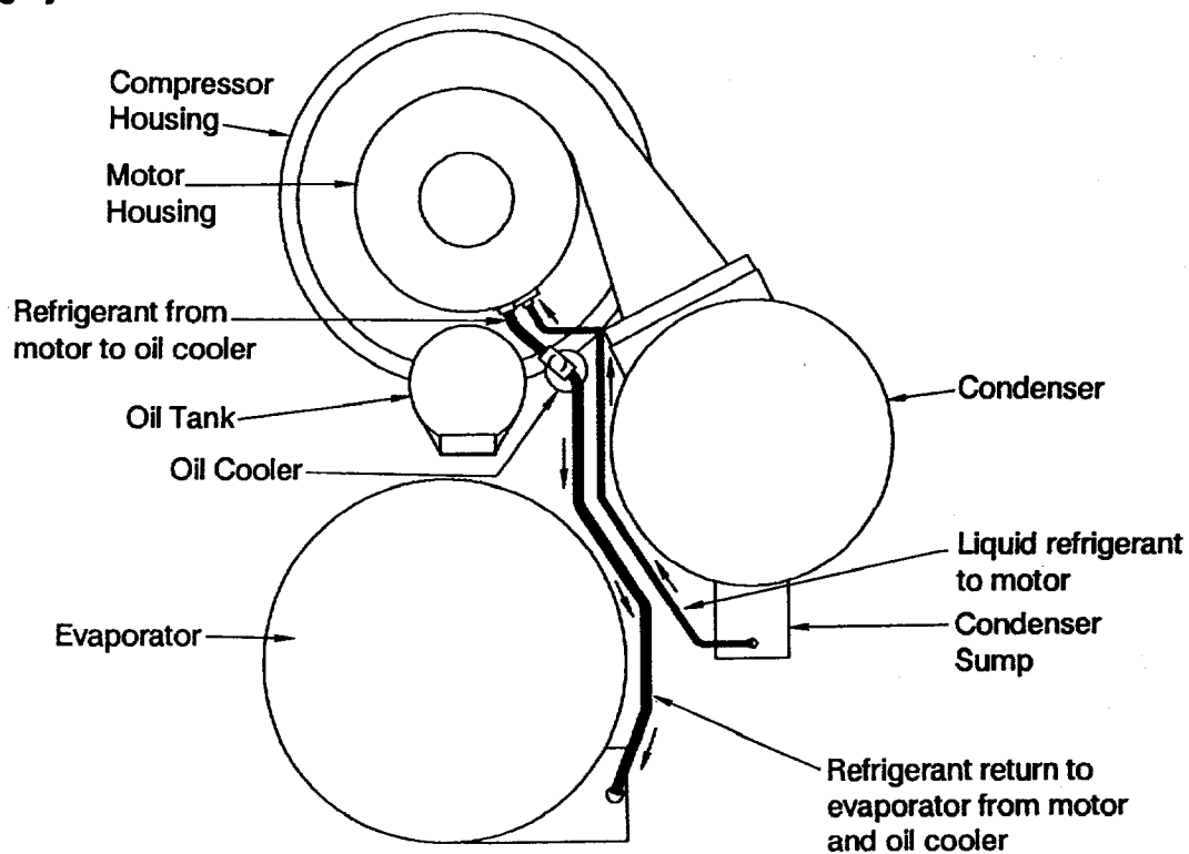
Figure 12 CVHF Motor Cooling System
