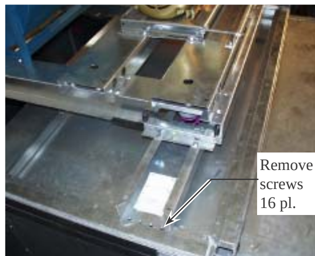
FIG. 8 - REMOVE SCREWS FROM ISOLATOR RAILS
