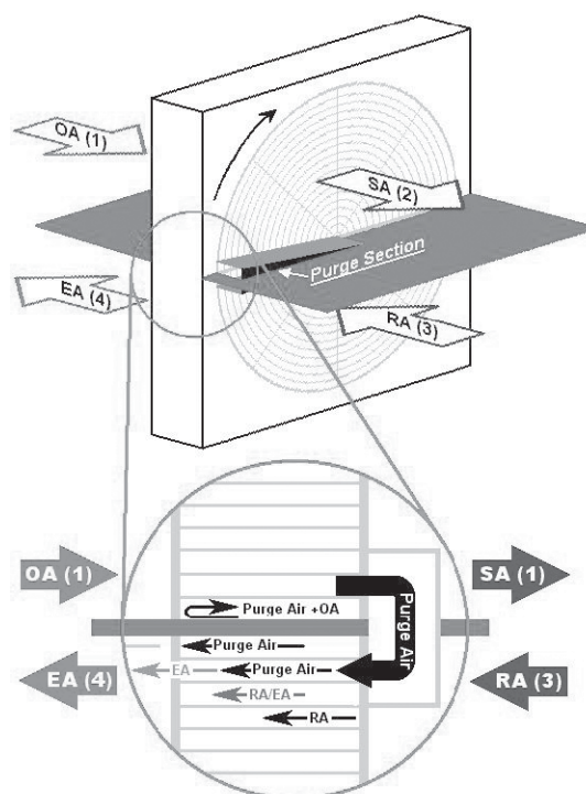
FIGURE 10 – ENERGY RECOVERY WHEEL WITH PURGE SECTION
