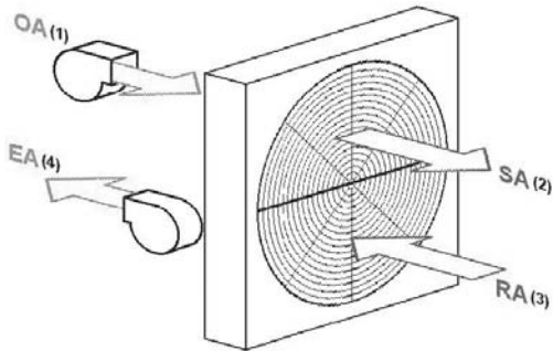
FIGURE 6 – BLOW-THRU SUPPLY/DRAW-THRU EXHAUST
