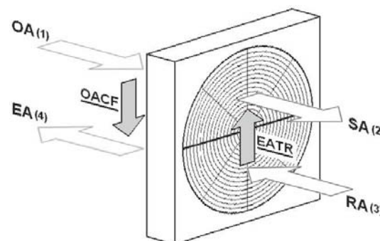
FIGURE 3 – AIR TRANSFER PATHS
