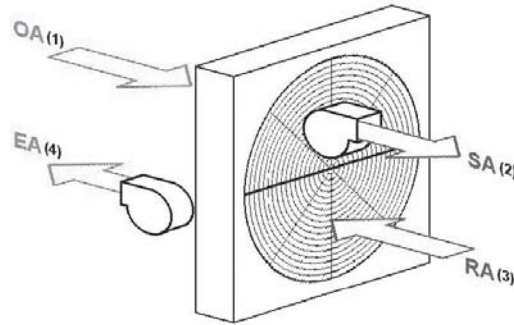
FIGURE 7 – DRAW-THRU SUPPLY/DRAW-THRU EXHAUST
