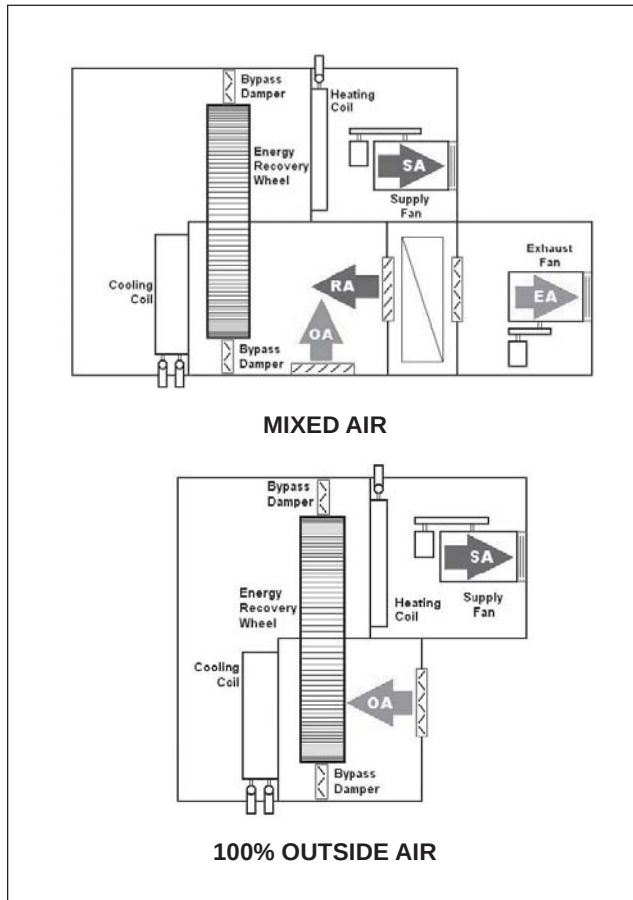
FIGURE 16 – SUPPLY AIR TEMPERATING (SERIES)
