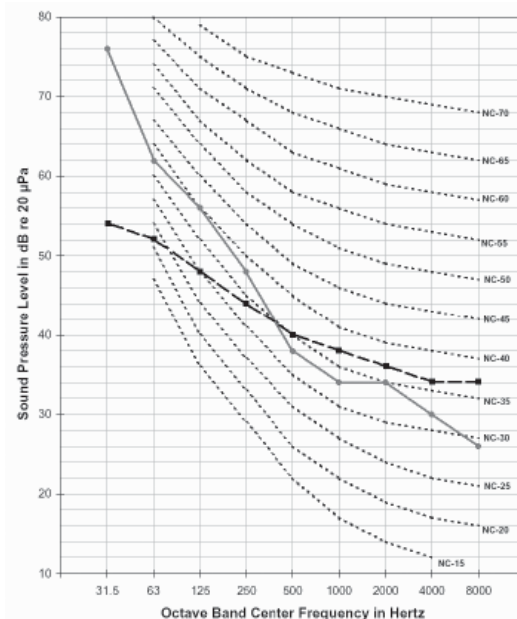
FIGURE 4 – NC CURVES
