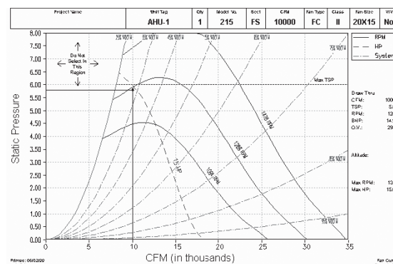
FIGURE 11 – POOR FAN SELECTION
