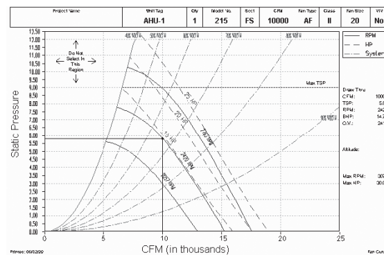
FIGURE 12 – GOOD FAN SELECTION
