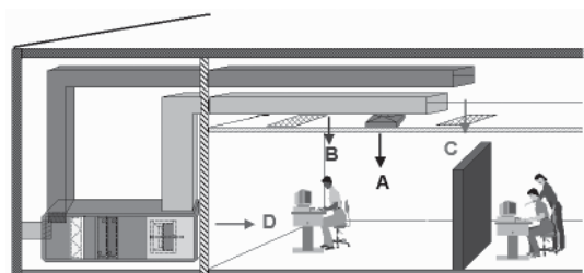
FIGURE 6 – CRITICAL SOUND PATHS
