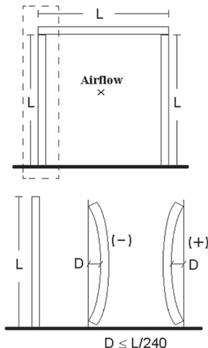
FIGURE 3. PANEL DEFLECTION
