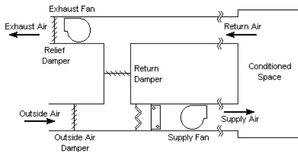
Figure 2. Exhaust Fan Economizer
