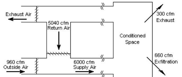
Figure 8. Return Fan Airflow with Space Losses
