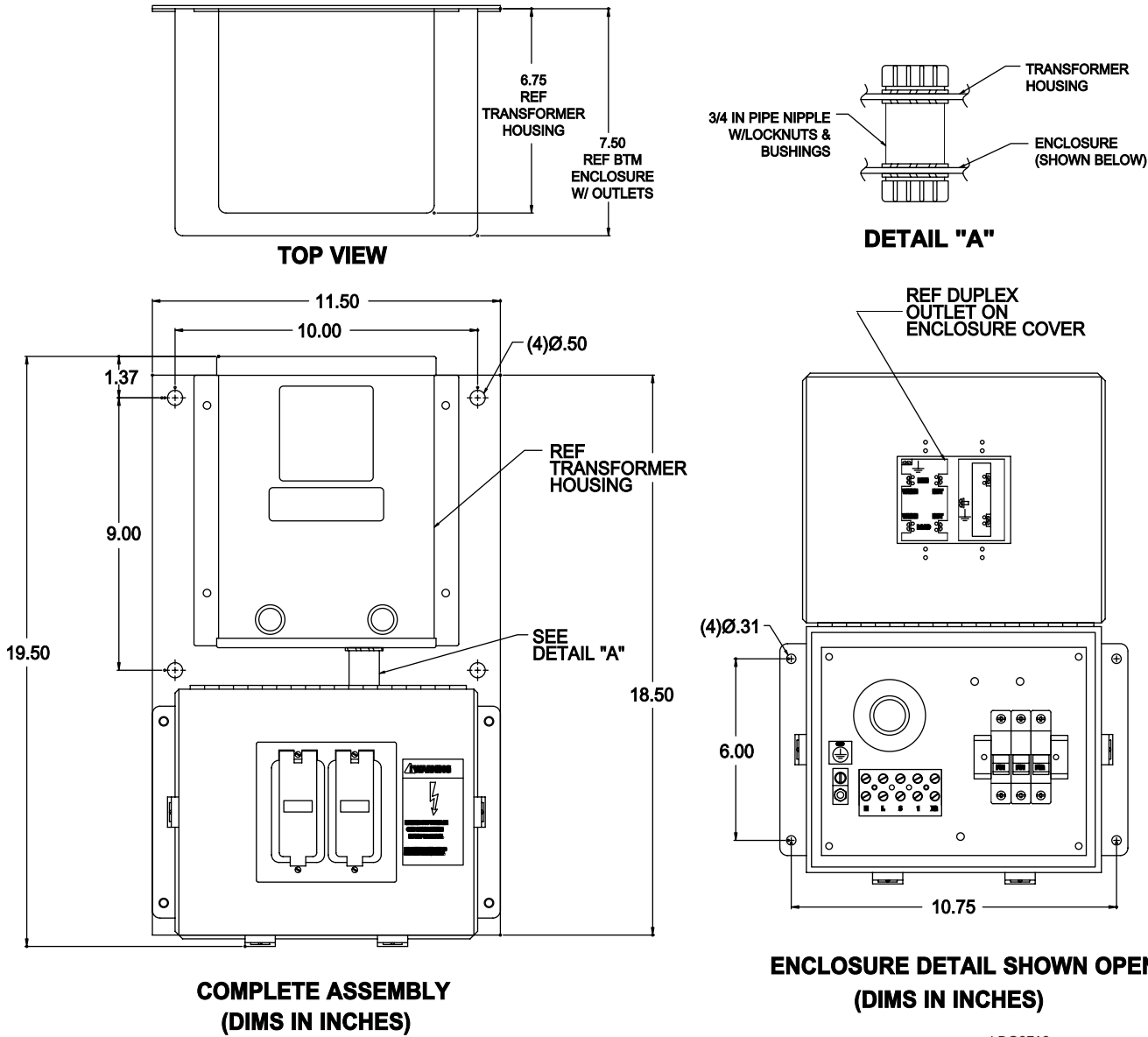
FIG. 21 - TRANSFORMER PANEL DIMENSIONS
