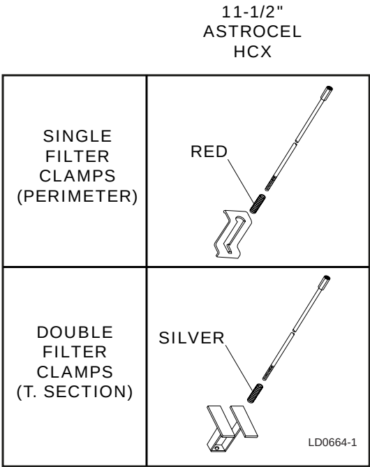
FIG. 16 - VISUAL CONTROL FILTER CLAMPS
