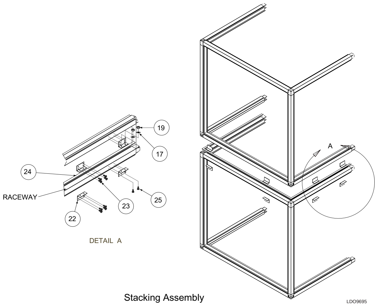
FIG. 11 - SPLICE & STACKING ASSEMBLIES
