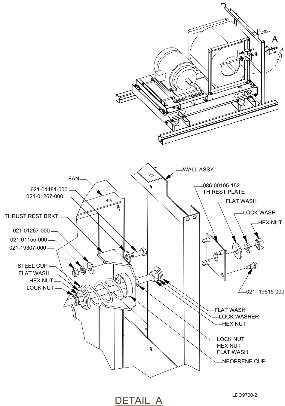
FIG. 3 - THRUST RESTRAINT INSTALLATION FOR COMEFRI AND INDUSTRIAL FANS DISCHARG- ING INTO WALLS
