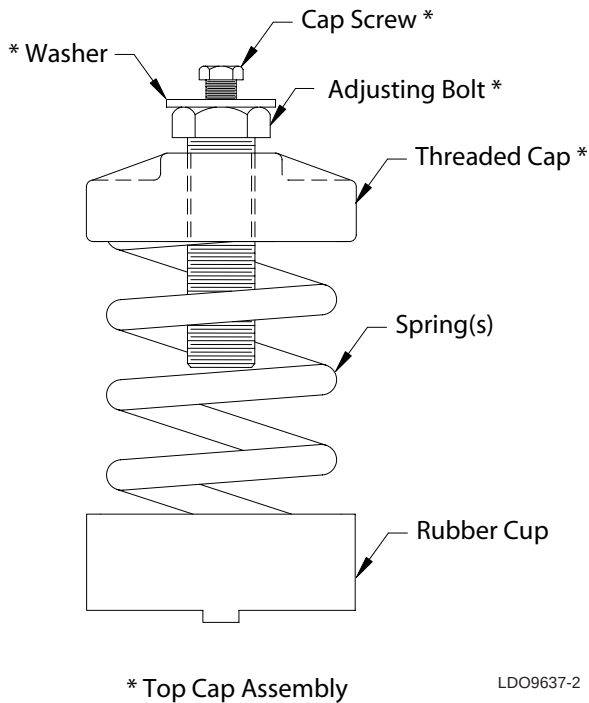
FIG. 10 - TYPICAL, ISOLATOR
