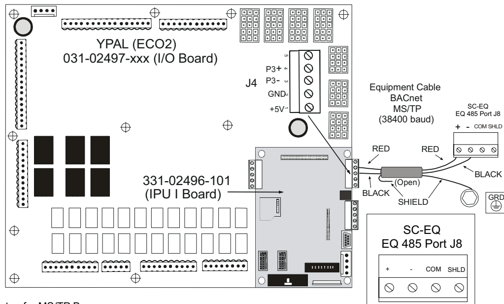
FIGURE 23 - SC-EQ COMM CARD CONNECTIONS FOR CHILLERS WITH THE 02550 MICROBOARD YCAL/YCUL/YLAA/YLPA/YCWL/YCRL/YSAA
