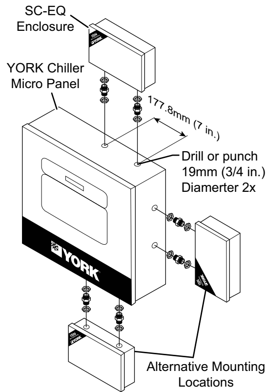
FIGURE 12 - MOUNTING ON THE EQUIPMENT
