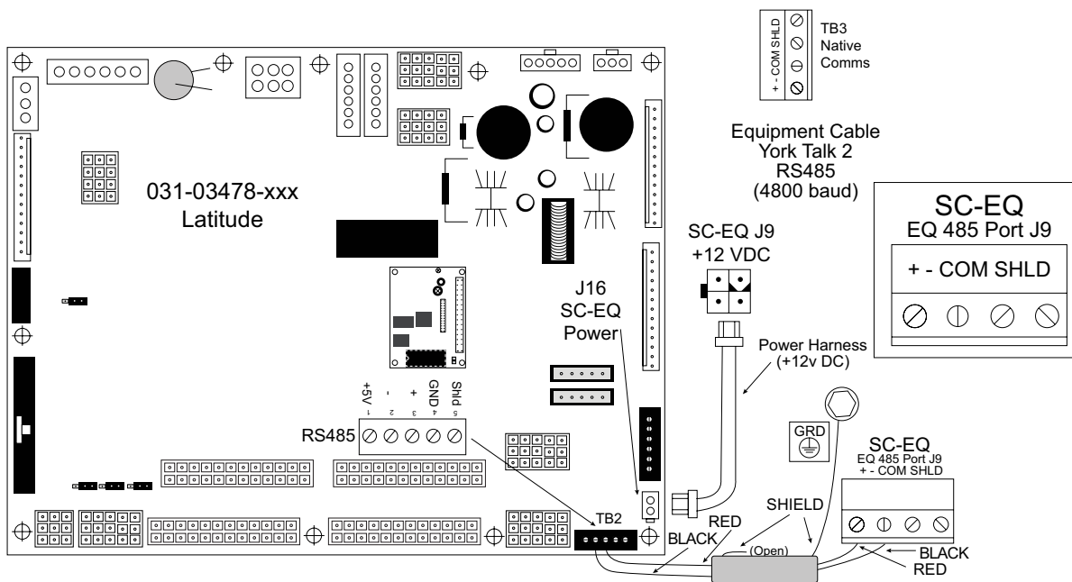
FIGURE 22 - SC-EQ COMM CARD CONNECTIONS FOR CHILLERS WITH THE 03478 MICROBOARD YCAV/ YCIV/YVAA/YVWA/YVFA
