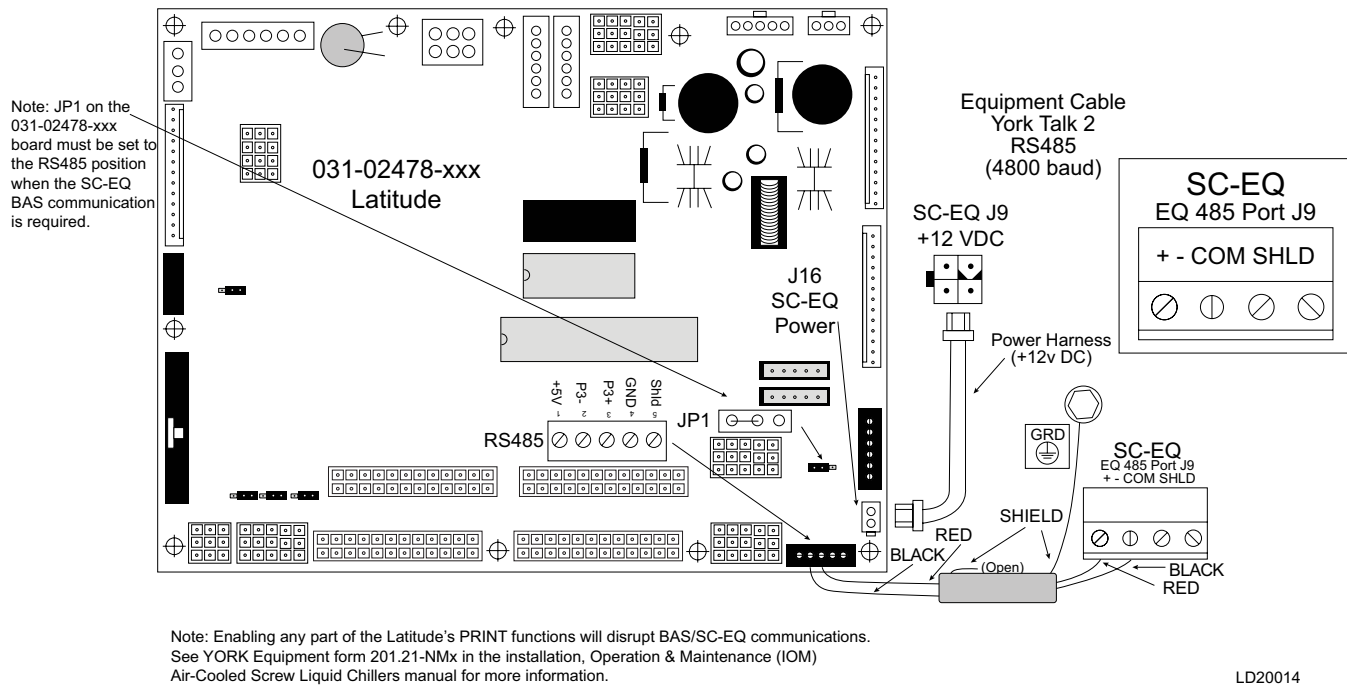
FIGURE 21 - SC-EQ COMM CARD CONNECTIONS FOR CHILLERS WITH THE 02478 MICROBOARD YCAV/ YCIV/YVAA/YVWA
