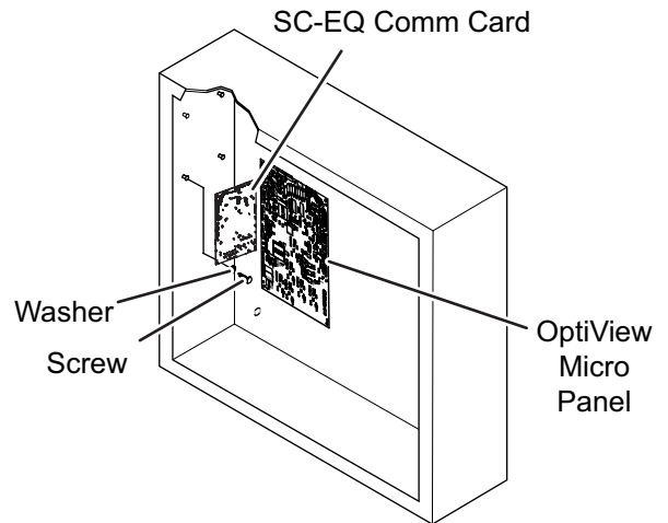
FIGURE 6 - SC-EQ INSTALLED IN OPTIVIEW (ALL CHILLERS EXCEPT YMC2)
