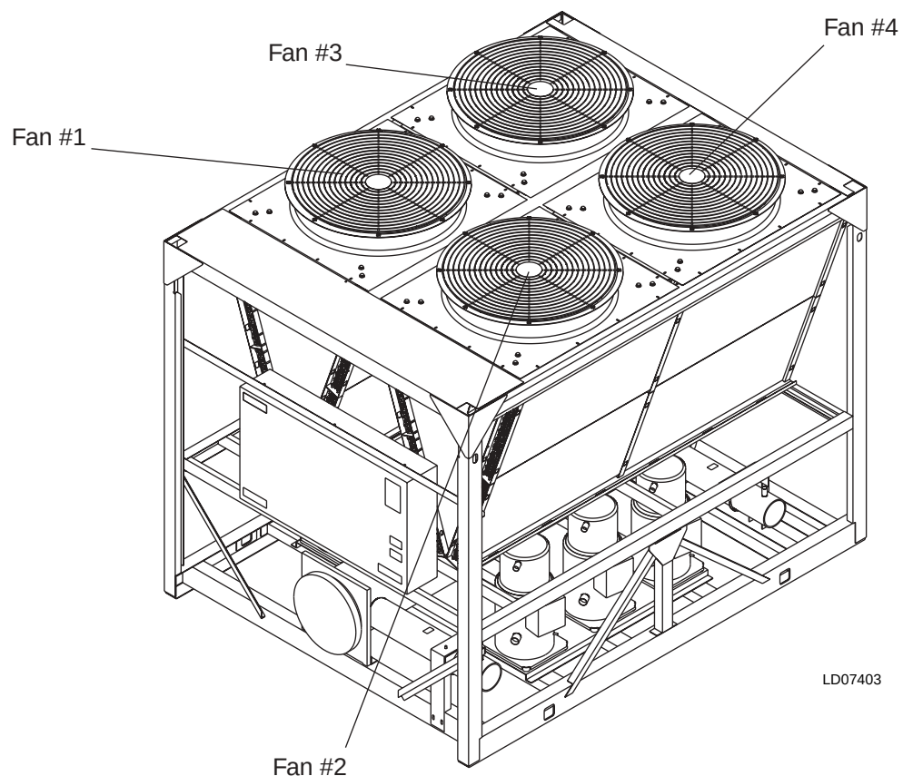
FIG. 9 – YCAL0014 – YCAL0253 FAN LOCATION (TYPICAL)
