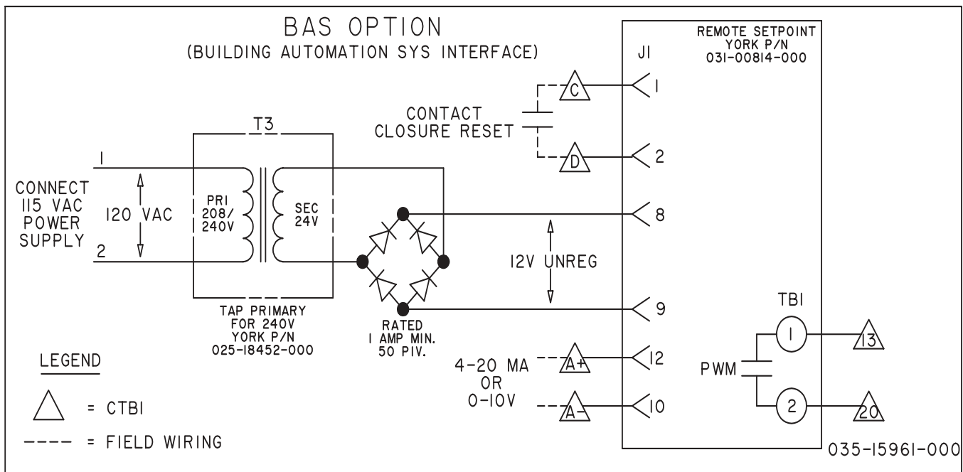
FIG. 12 – FIELD AND FACTORY ELECTRICAL CONNECTIONS OPTIONAL REMOTE TEMPERATURE RESET BOARD
