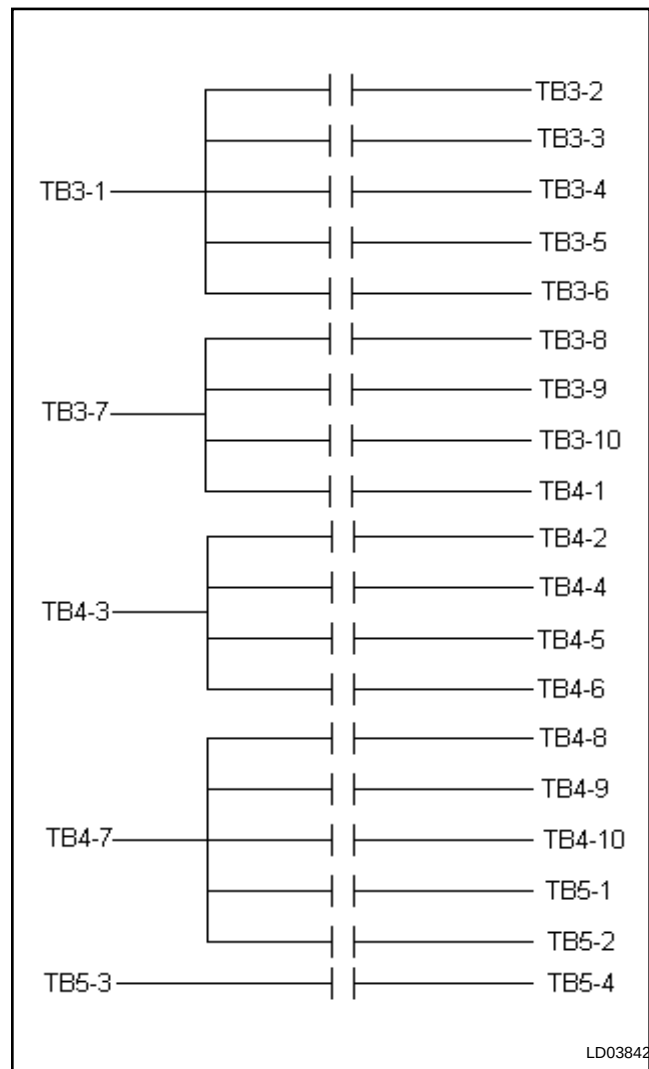
FIG. 14 – MICROBOARD RELAY CONTACT ARCHITECTURE
