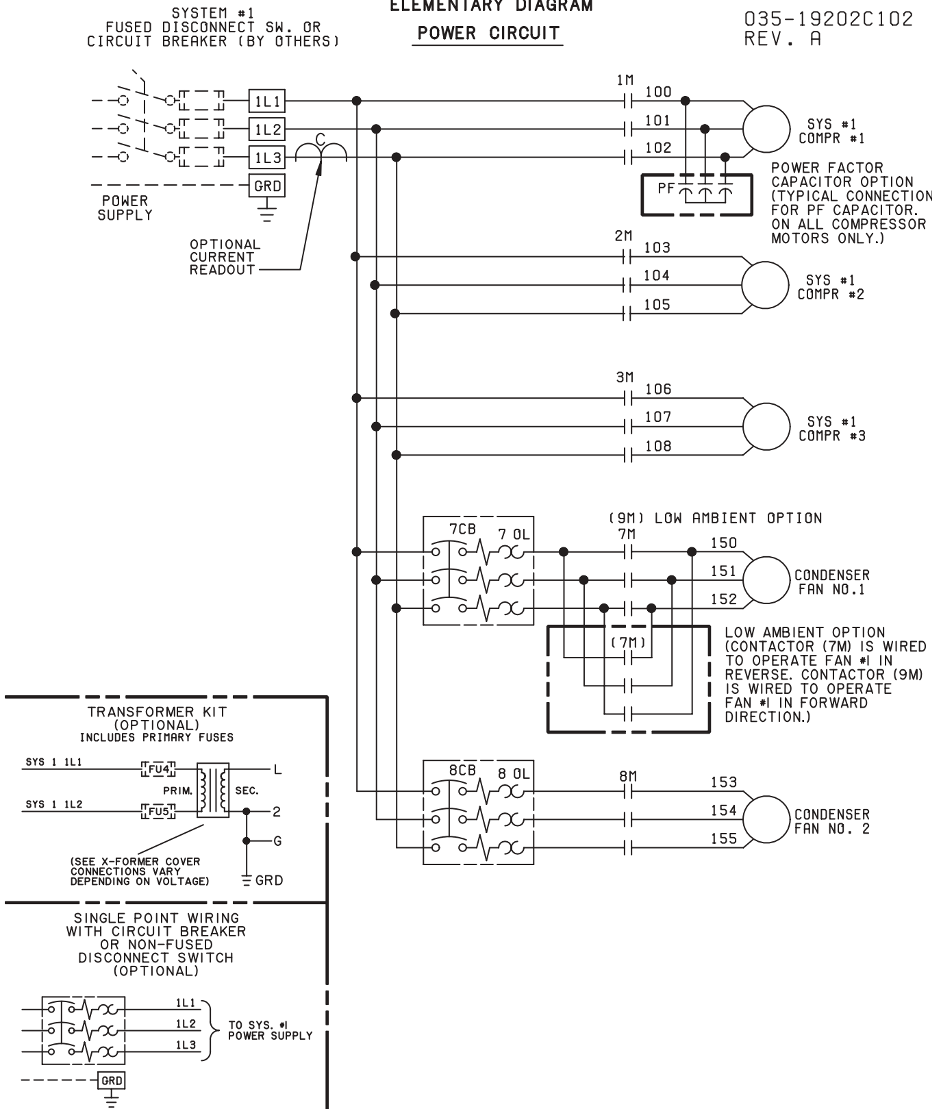
FIG. 21 – ELEMENTARY DIAGRAM, POWER CIRCUIT – YCAL0107E_
