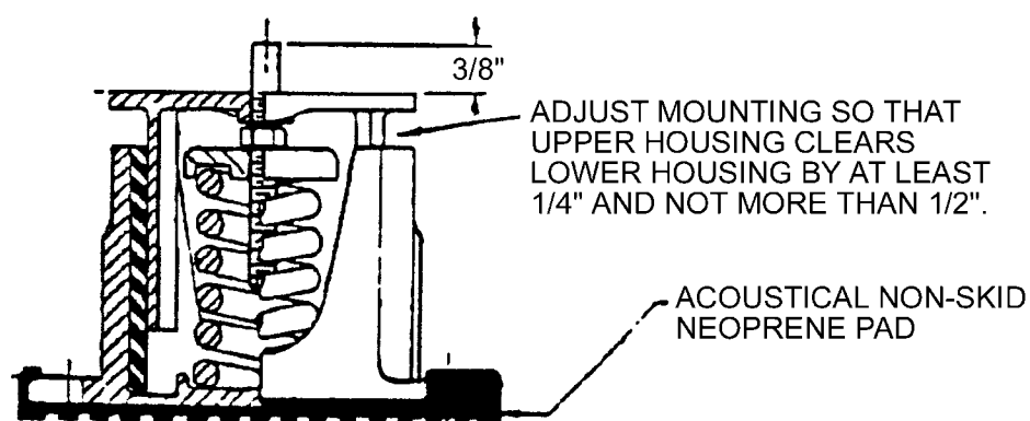
FIG. 43 – TYPE CP MOUNTING
