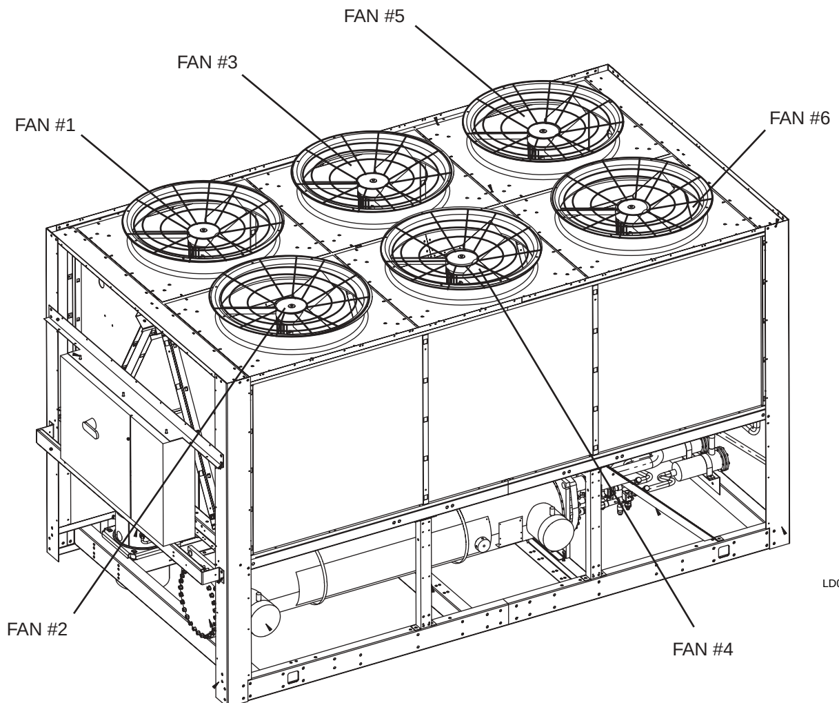
FIG. 10 – YCAL0287 – YCAL0377 FAN LOCATION
