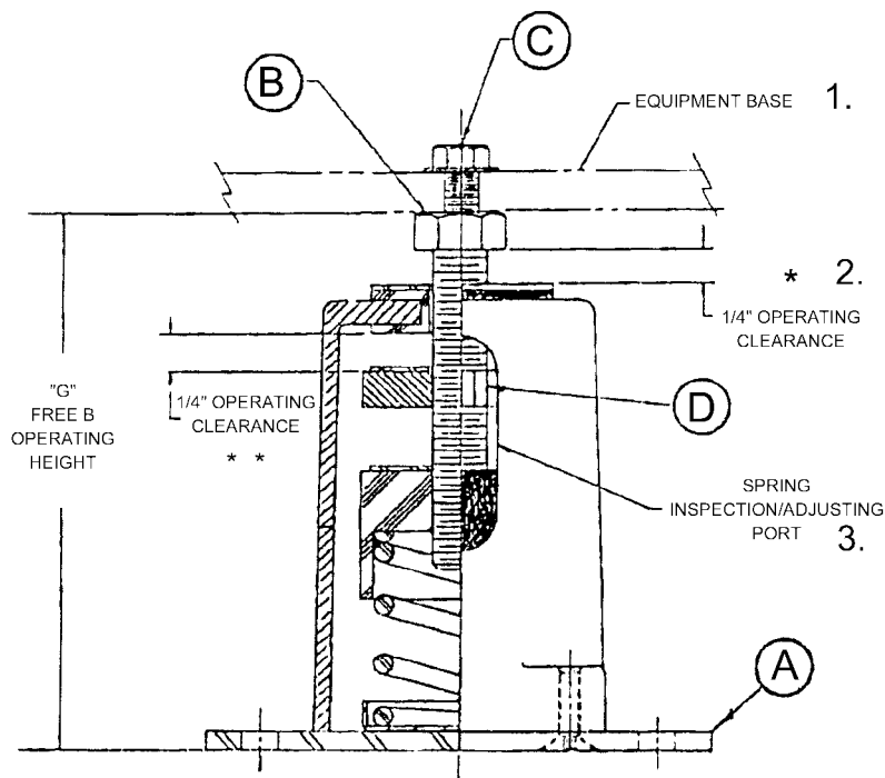
FIG. 44 – "AEQM" SPRING-FLEX MOUNTING
