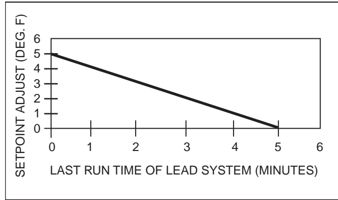
FIG. 7 – SETPOINT ADJUST
