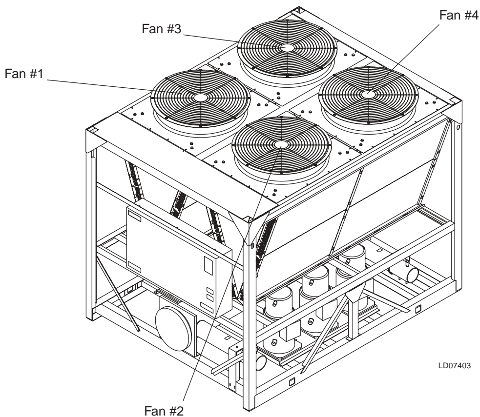
FIG. 9 – YCAL0014 – YCAL0080 FAN LOCATION (TYPICAL)
