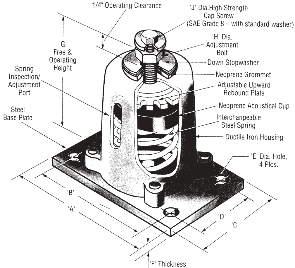
FIG. 36 – R SPRING SEISMIC ISOLATOR
