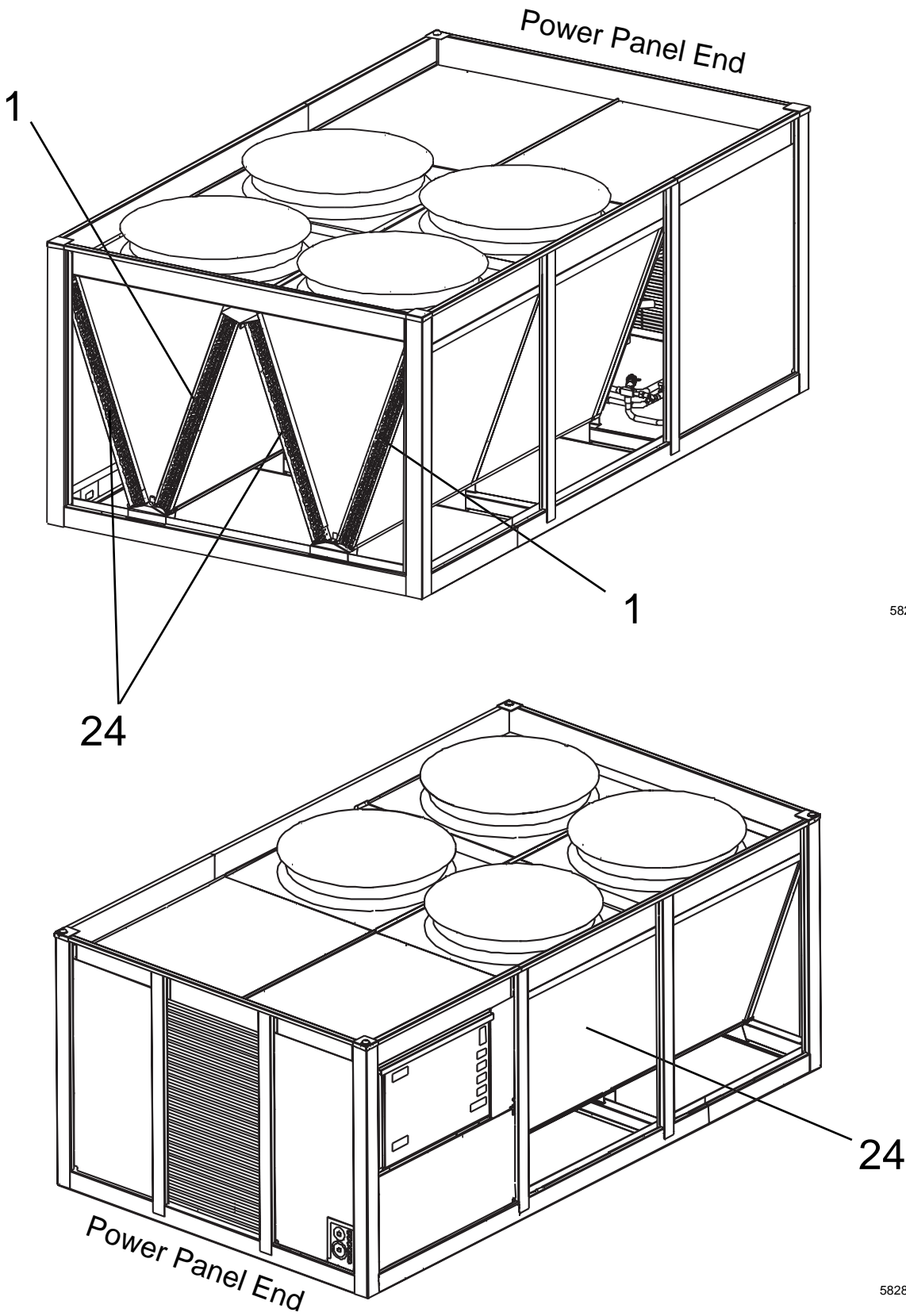
FIG. 2 – CONDENSER COIL LAYOUT (REF. TABLE 2, PAGE 9)
