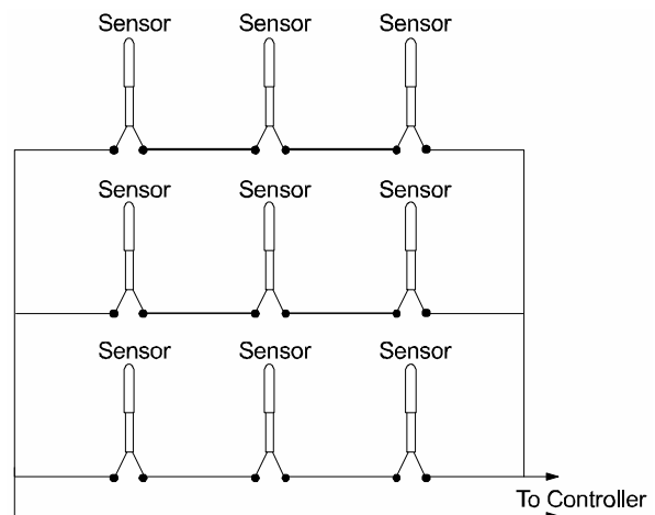
Four and Nine Temperature Sensors Wired in Series/Parallel Arrangement Schematics
