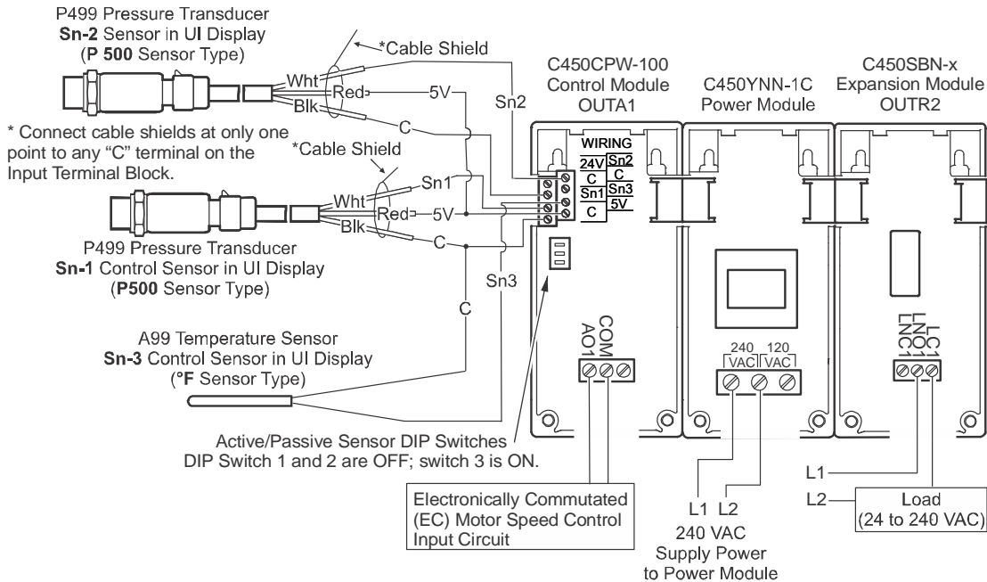
Figure 13: System 450 Hybrid Analog Output Control System Example with Condenser Fan (EC) Motor Speed Control, High Input Signal Selection
