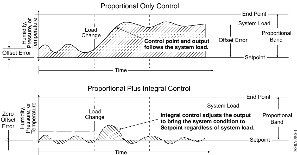
Figure 8: Proportional Only Control Versus Proportional Plus Integral Control
