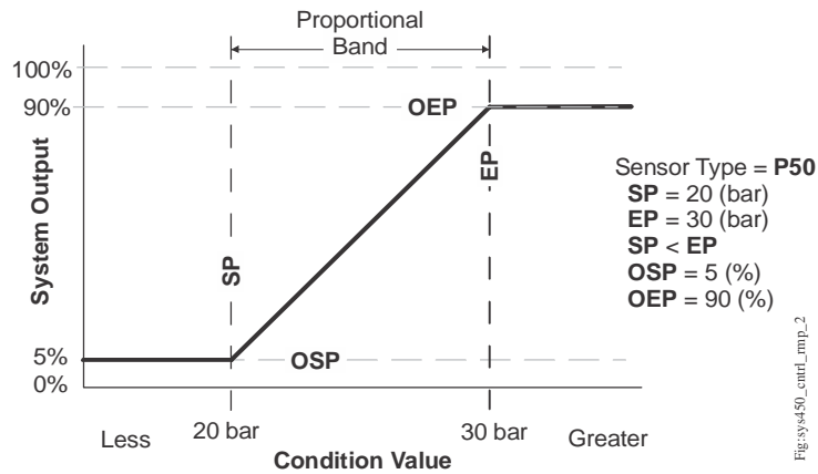
Figure 24: Relationship between Setpoint, End Point, Output at Setpoint, and Output at End Point for an Analog Output That Controls Condenser Fan Speed
