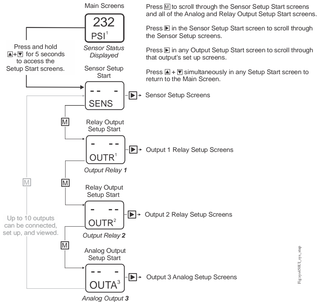
Figure 18: Accessing the Setup Start Screens in the System 450 UI
