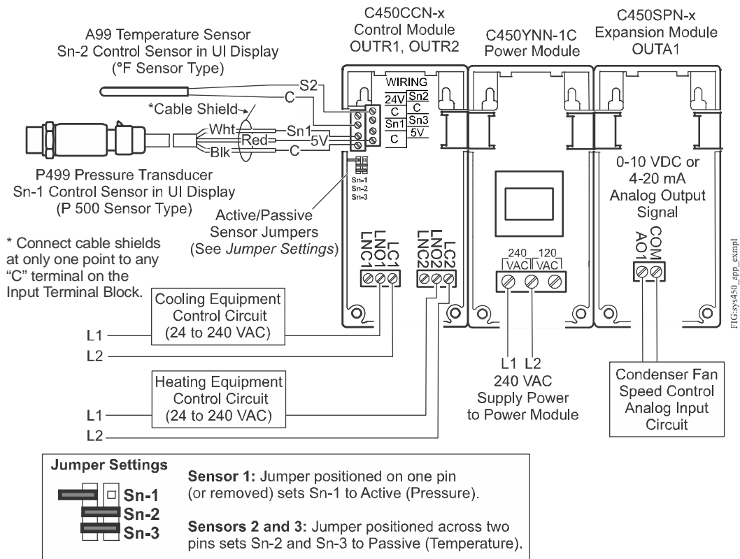
Figure 1: System 450 Standard Control System Connected as a Room Heating and Cooling Control System with Condenser Fan Speed Control
