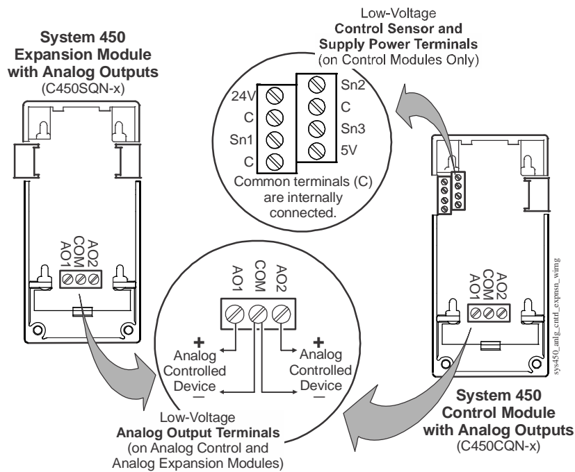
Figure 16: Wiring Terminal Details for System 450 Control and Expansion Modules with Analog Outputs
