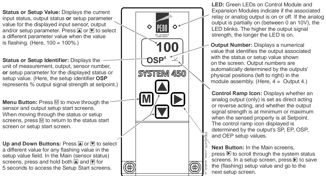
Figure 2: System 450 Control Module with Analog Outputs Showing LCD and Four-Button Touchpad User Interface
