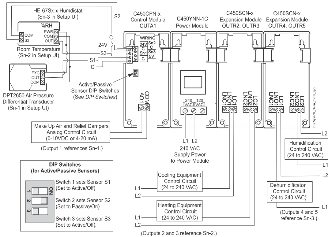
Figure 9: Standard System 450 Control System Example for a Clean Room Application That Controls Temperature, Pressure, and Humidity Simultaneously
