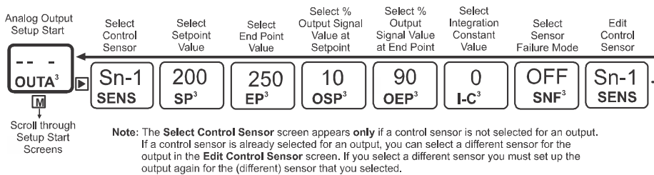
Figure 25: Analog Output Setup Start Screen and Setup Screen Flow
