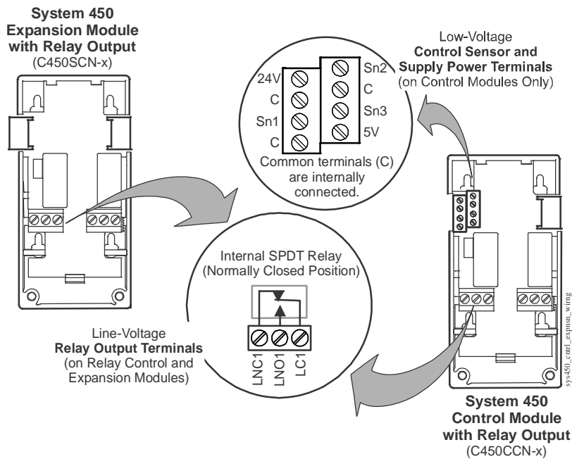
Figure 15: Wiring Terminal Details for System 450 Control and Expansion Modules with Relay Output
