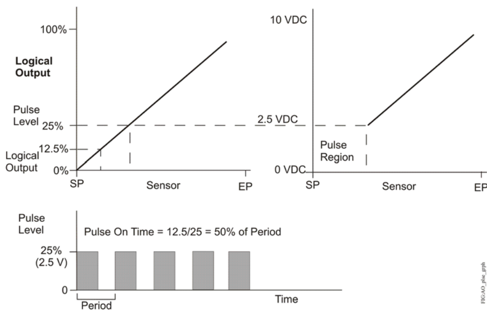
Figure 5: Pulse Signal with Pulse Level = 25% and Logical Output = 12.5%
