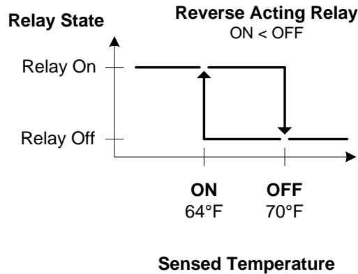
Figure 21: Reverse Acting Relay (ON < OFF) Set Up to Control Heating
