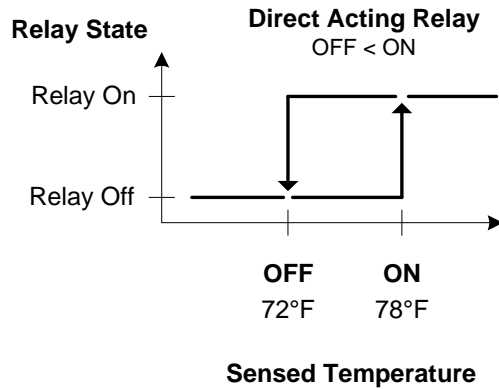
Figure 20: Direct Acting Relay (OFF < ON) Set Up to Control Cooling
