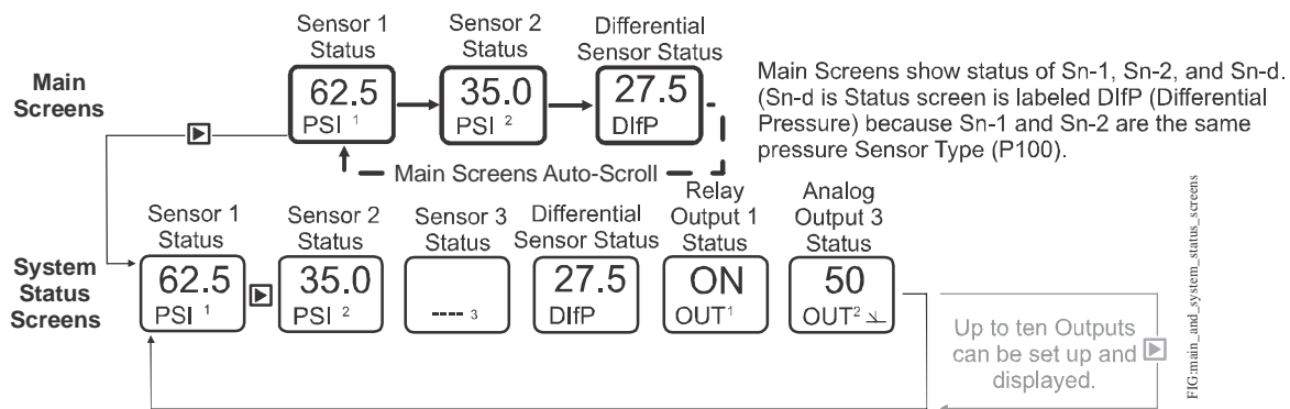
Figure 17: Main Screens and System Status Screens Example for a Standard System 450 Control System Set Up for Differential Control
