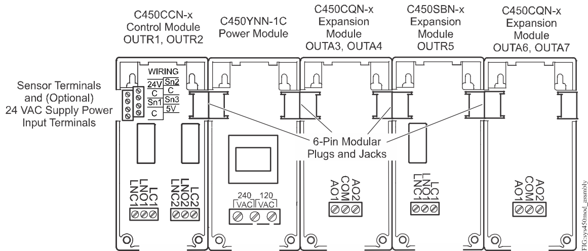
Figure 4: System 450 Module Assembly Example Showing Standard Control Module Positions, Output Positions, and Output Numbers
