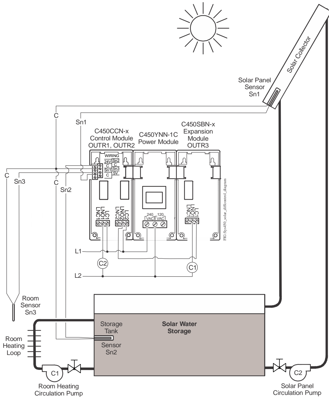
Figure 11: Solar Water Space Heating Control System Example That Uses the Differential Control Feature
