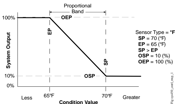
Figure 23: Relationship between Setpoint, End Point, Output at Setpoint, and Output at End Point for an Analog Output That Controls Room Heating
