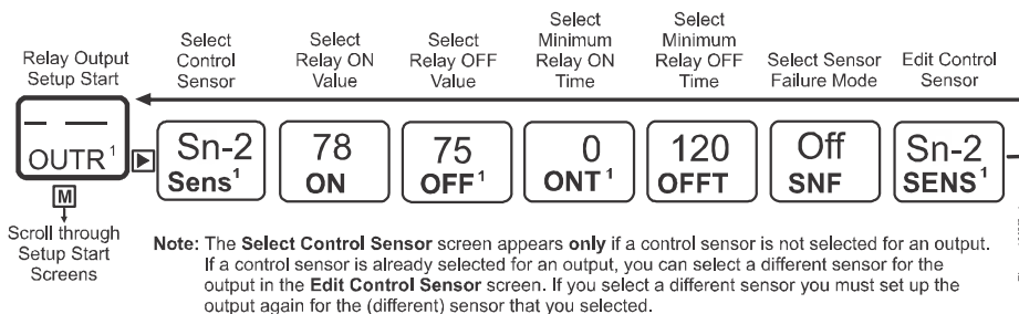
Figure 22: Relay Output Setup Start Screen and Setup Screen Flow
