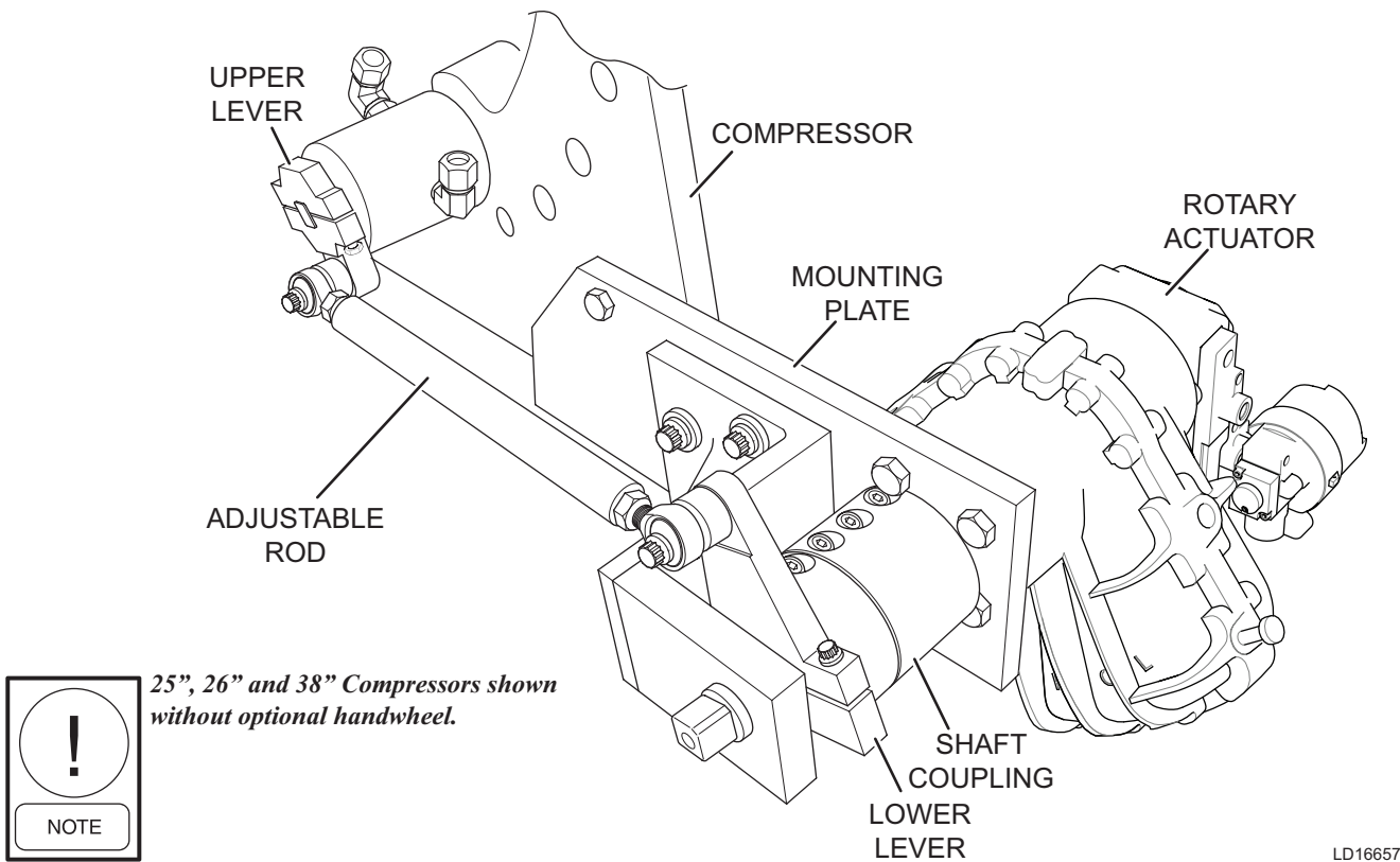
FIGURE 2 - KINETROL PNEUMATIC ACTUATOR WITH PRV ACTUATOR MOUNTING KIT
