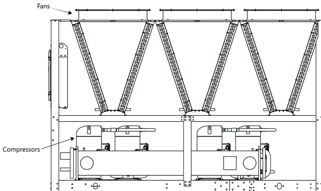
Schematic Diagram of Air-Cooled Chiller Primary Sound Source
