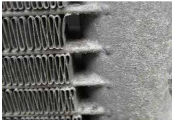
FIGURE 7 – Typical MCHX with Visible Flux Residue
