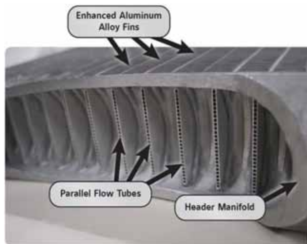
FIGURE 1 – Cut Away View of Basic Microchannel Heat Exchanger Construction
