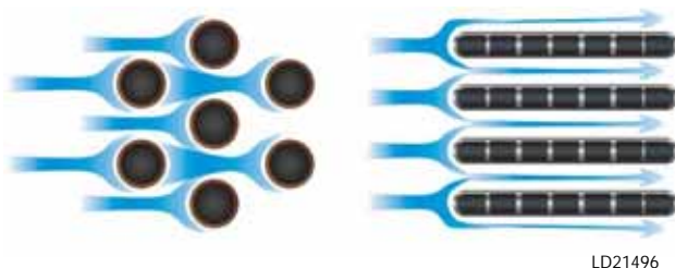
FIGURE 3 – RTPF vs. MCHX Air Flow
