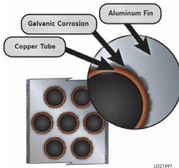
FIGURE 4 – Galvanic Corrosion between Copper Tubes and Aluminum Fin
