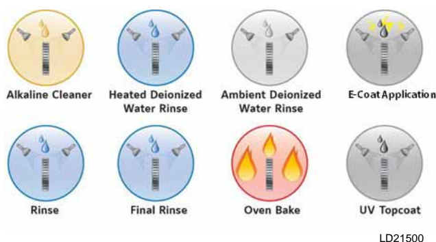
FIGURE 8 – E-coat Process
