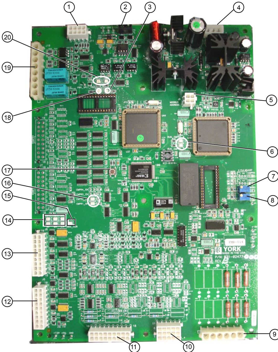
FIG. 3 – LATITUDE COMPRESSOR DRIVE LOGIC BOARD DETAILS
