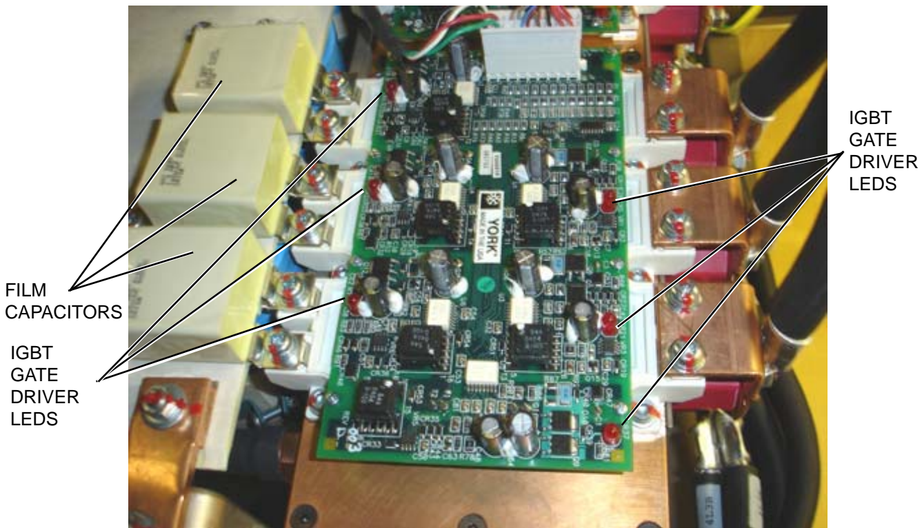
FIG. 4 – IGBT GATE DRIVER BOARD
