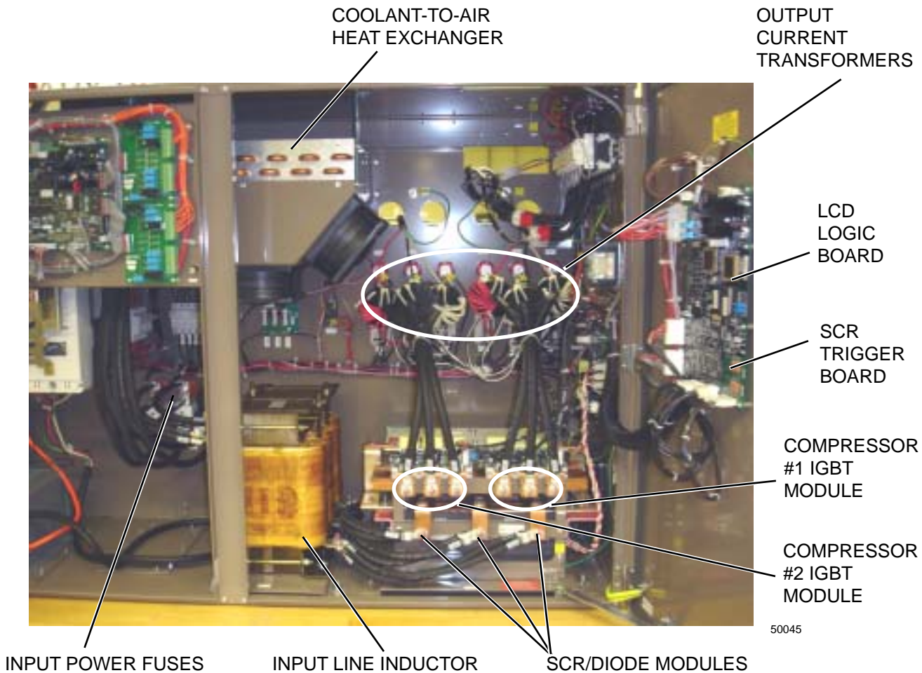
FIG. 1 – LCD CONTROL PANEL
