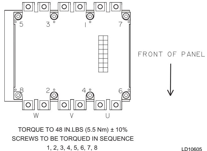
FIG. 13 – IGBT MODULE TORQUE SEQUENCE
