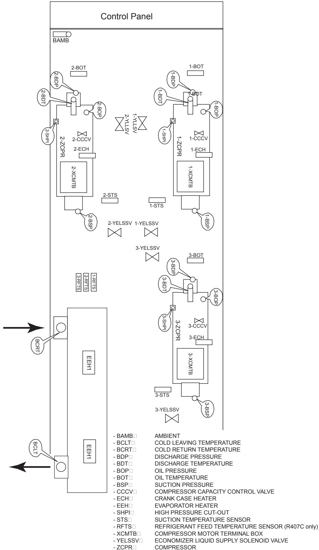
FIG. 65 – COMPONENT LOCATIONS
