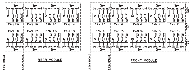
FIG. 80 – CONDENSER FAN CONTROL LAYOUT FOR DXST COMPRESSORS UNITS
