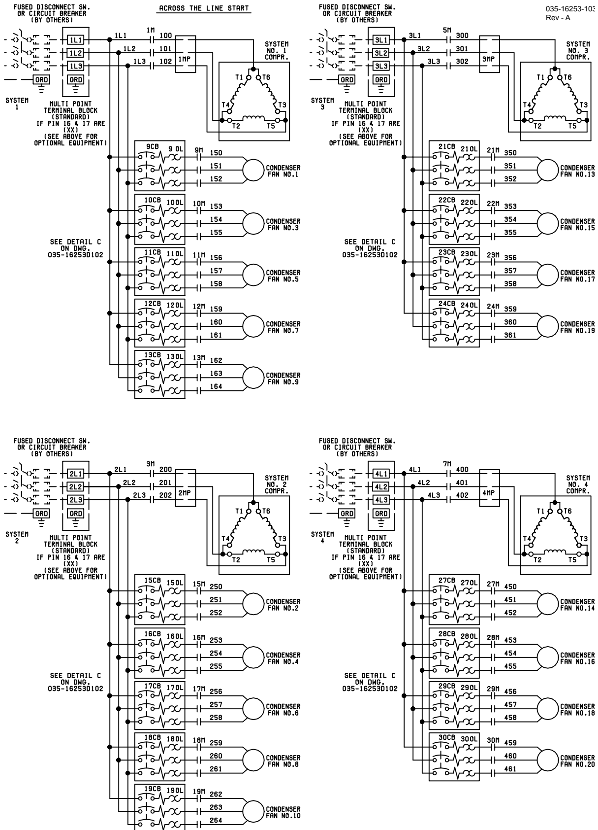
FIG. 36 – ELEMENTARY WIRING DIAGRAM - WYE DELTA START
