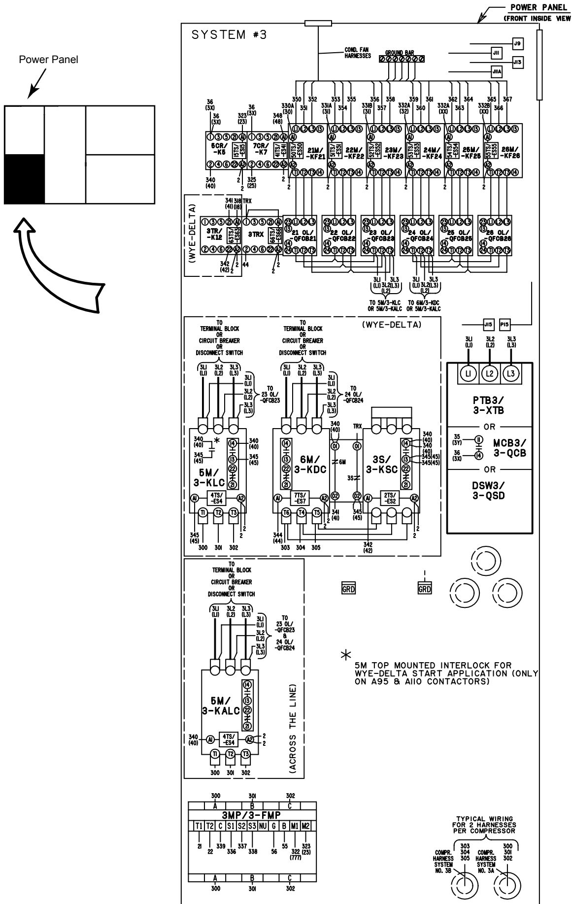
FIG. 29 – CONNECTION DIAGRAM 3 COMPRESSOR ELECTRONIC PANEL
