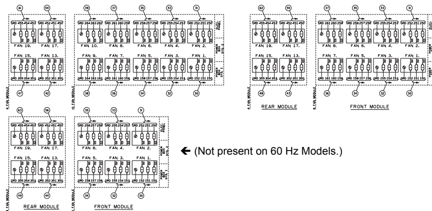
FIG. 79 – CONDENSER FAN CONTROL LAYOUT FOR DXST COMPRESSORS UNITS
