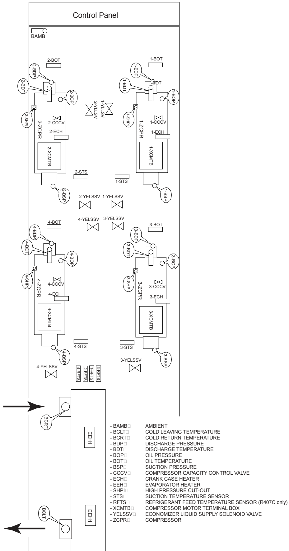
FIG. 65 – COMPONENT LOCATIONS (CONT'D)
