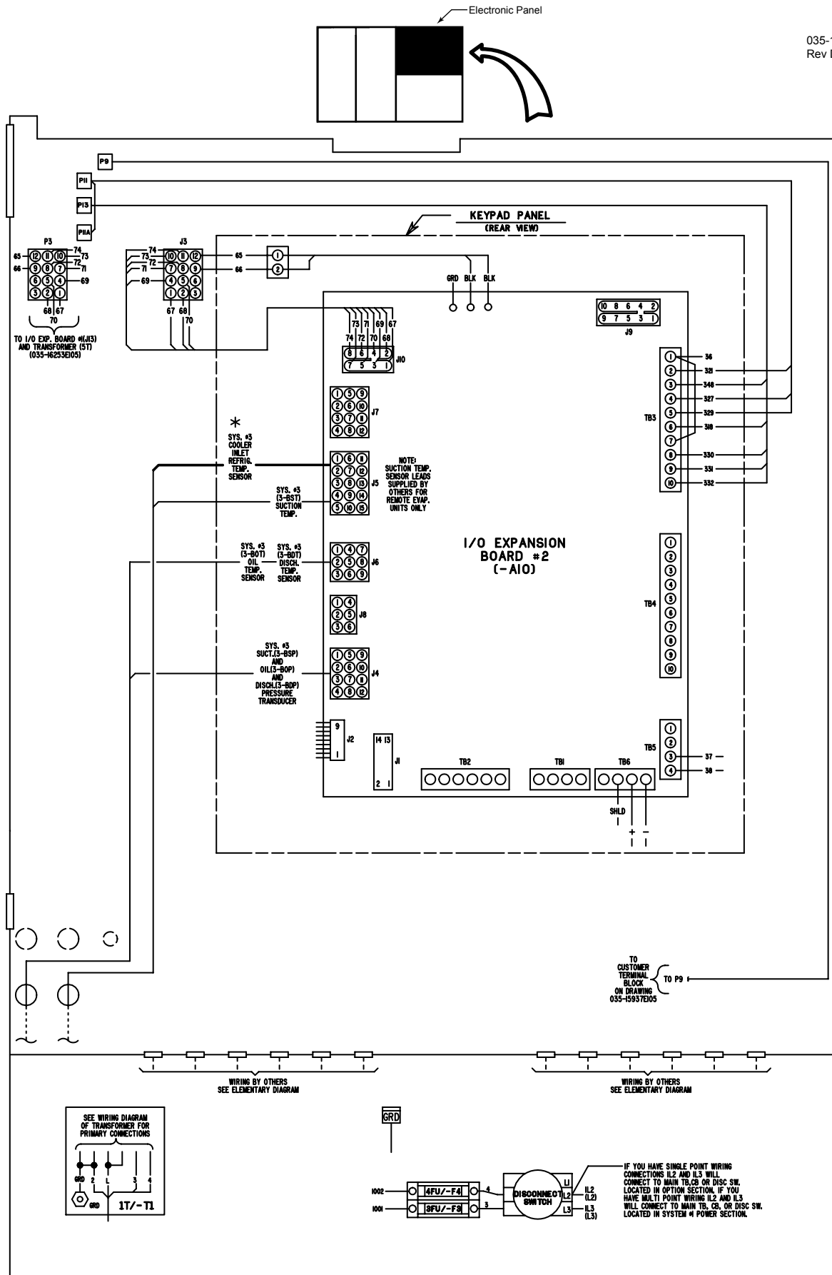
FIG. 30 – ELEMENTARY DIAGRAM 3 COMPRESSOR DXST DIRECT DRIVE CONTROL CIRCUIT
