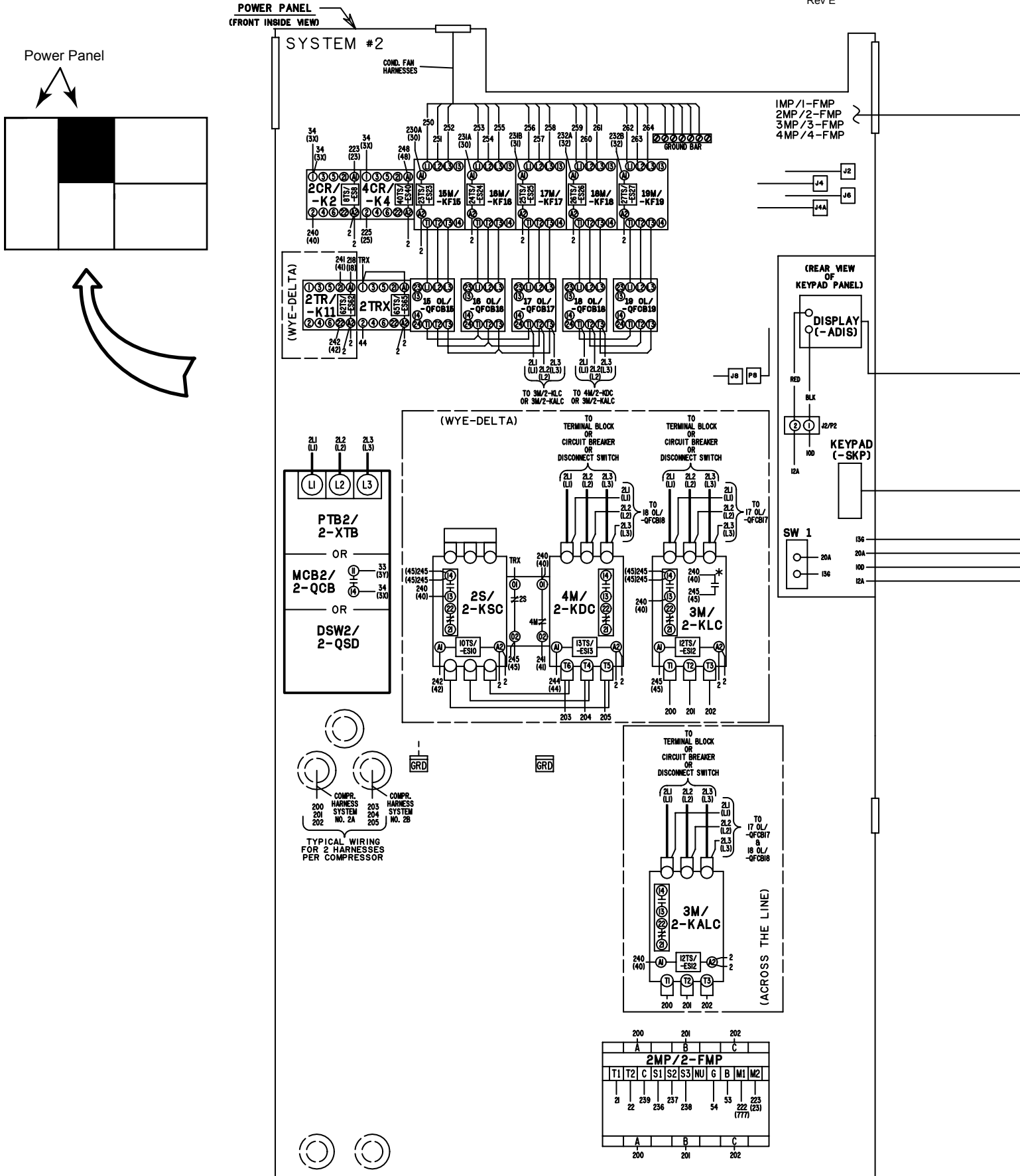
FIG. 27 – CONNECTION DIAGRAM 3 COMPRESSOR POWER PANEL
