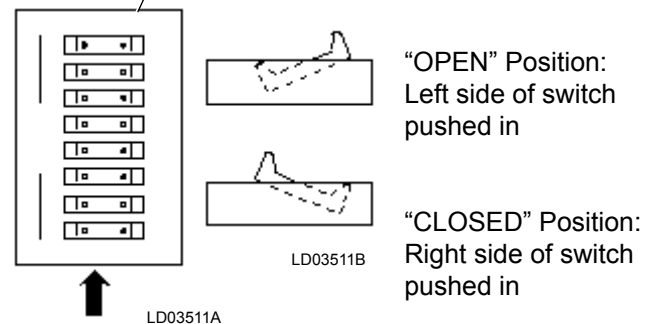
FIG. 77 – ENLARGED PHOTOGRAPH OF DIP SWITCHES ON MICROPROCESSOR BOARD
