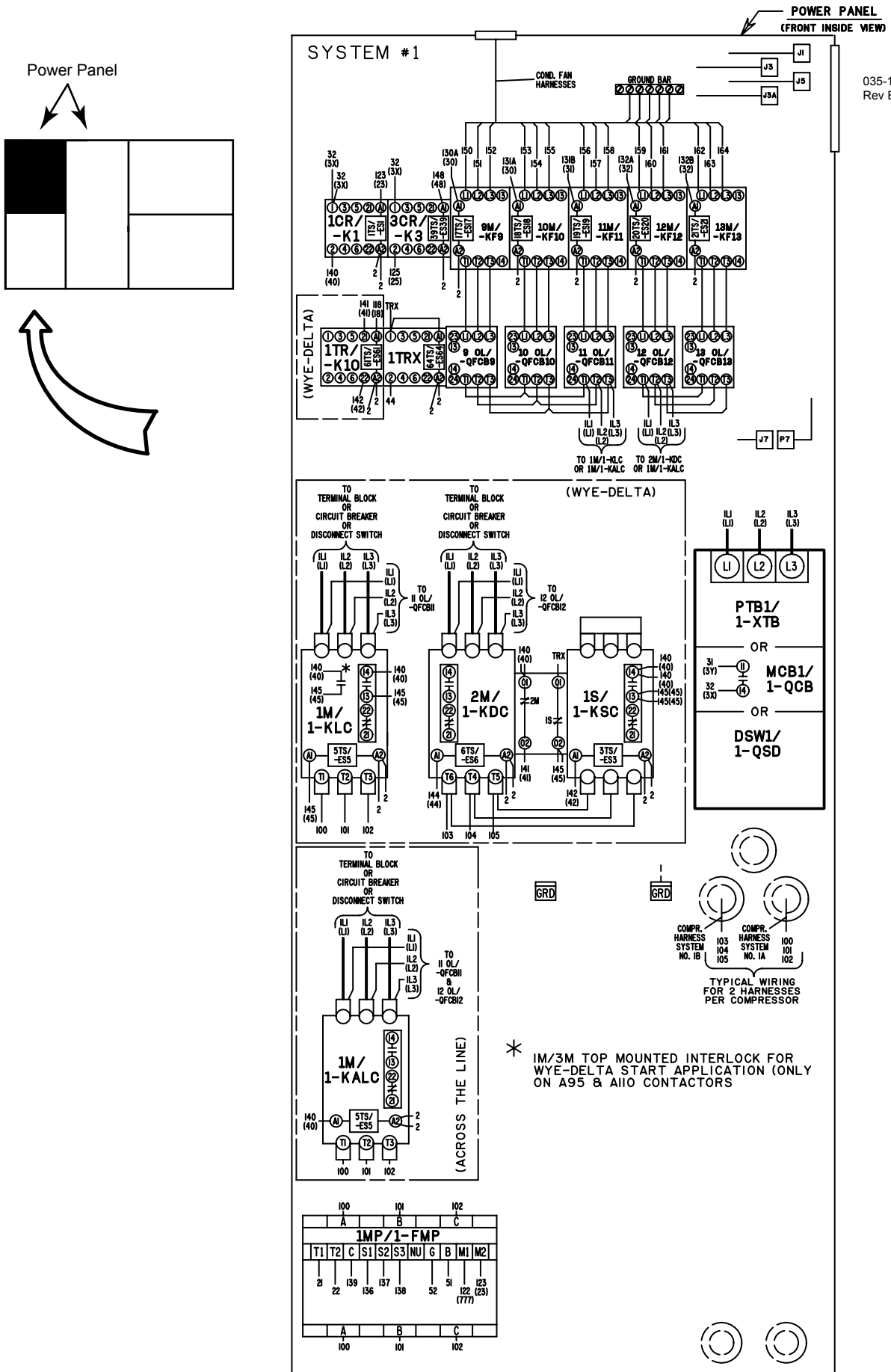
FIG. 26 – CONNECTION DIAGRAM 3 COMPRESSOR POWER PANEL
