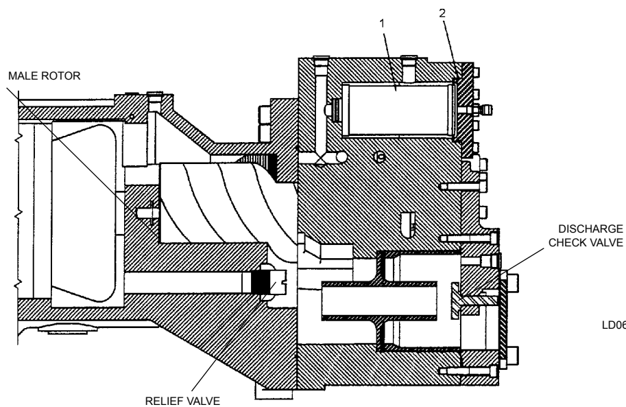
FIG. 69 – COMPRESSOR COMPONENTS
