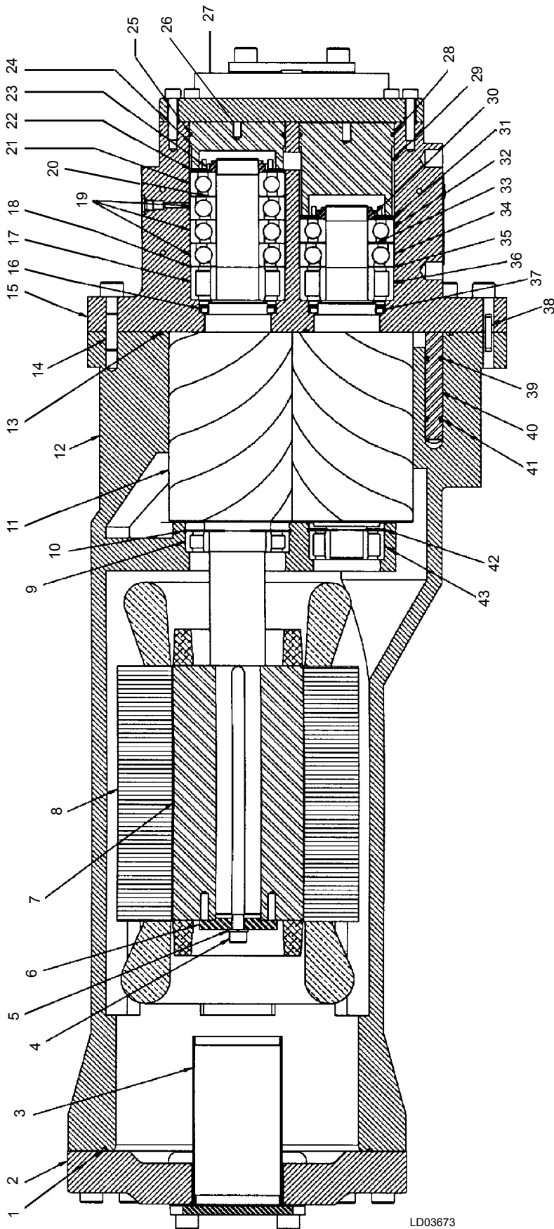
FIG. 70 – COMPRESSOR COMPONENTS
