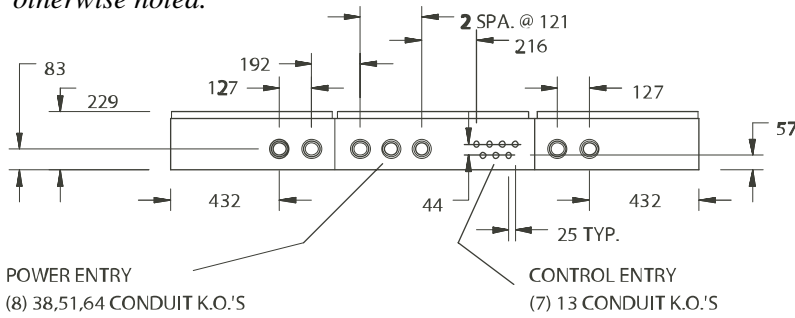
VIEW B-B
