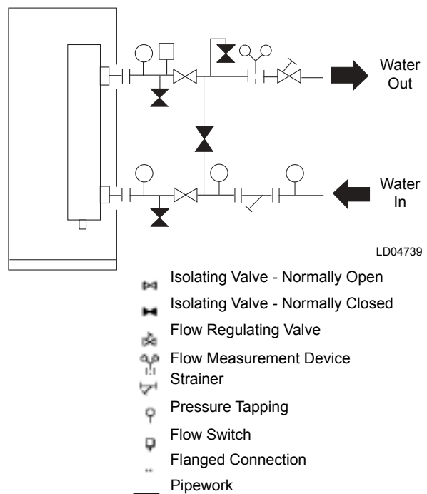
FIG. 6 – PIPEWORK ARRANGEMENT
