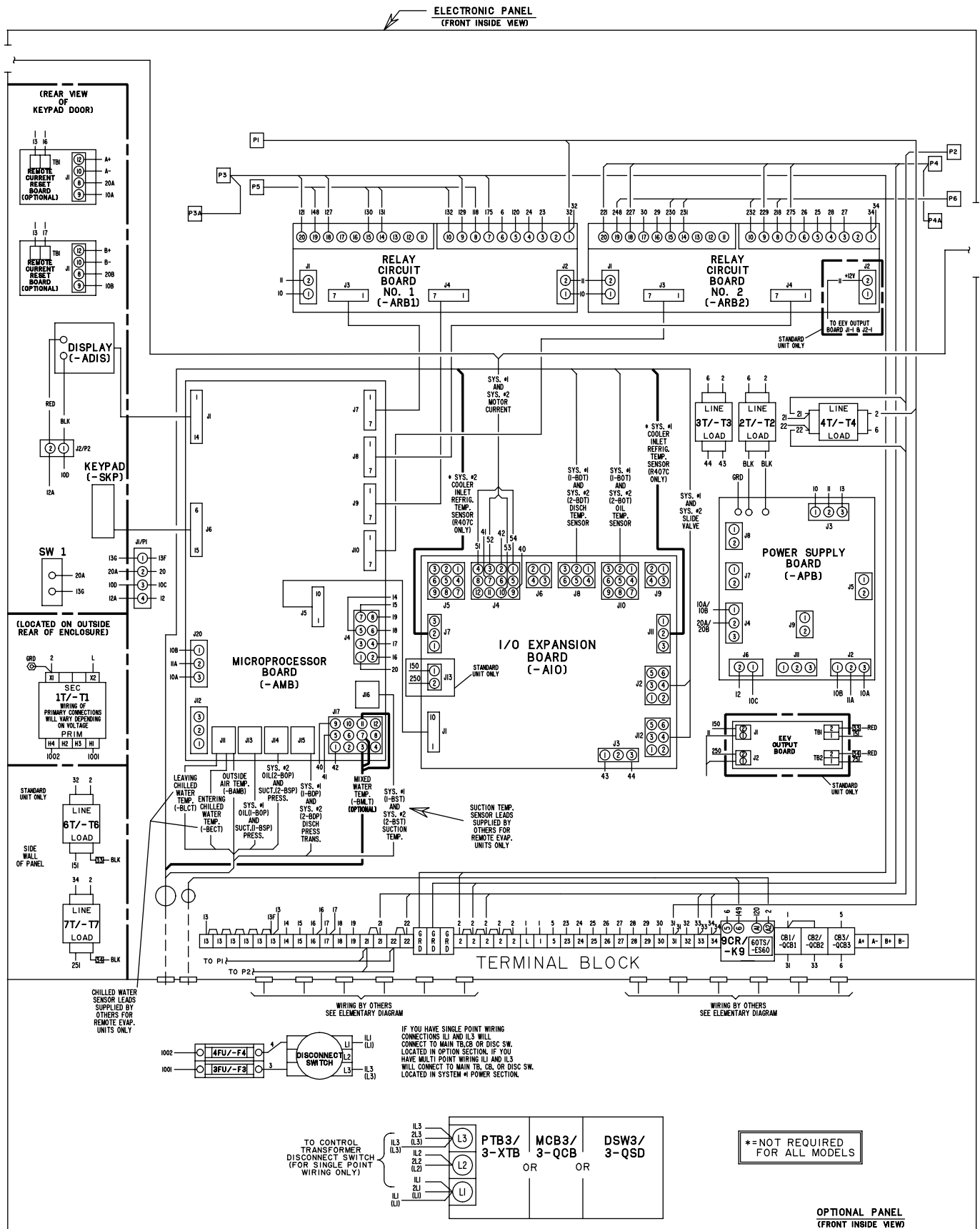
FIG. 22B – CONTROL PANEL COMPONENT LOCATION
