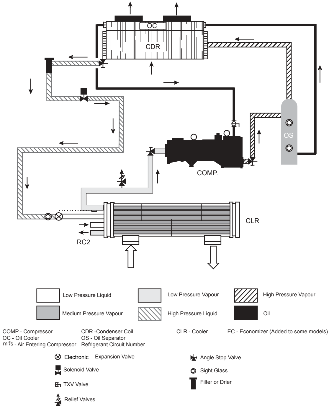
FIG. 42 – REFRIGERANT FLOW DIAGRAM
