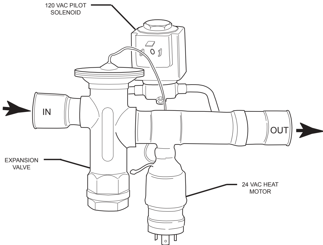
FIG. 57 – ELECTRONIC EXPANSION VALVE
