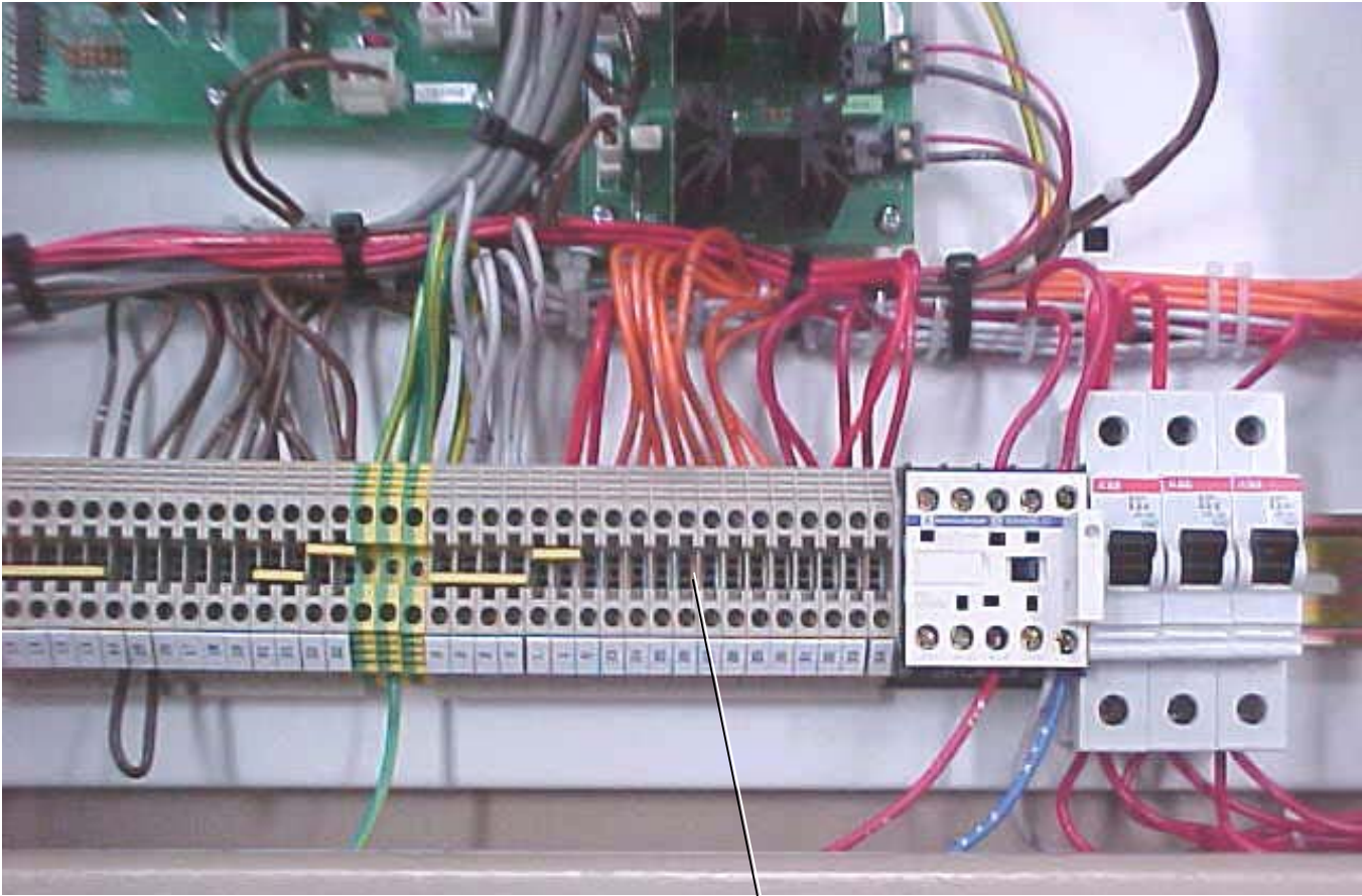
TERMINALS 13-34
