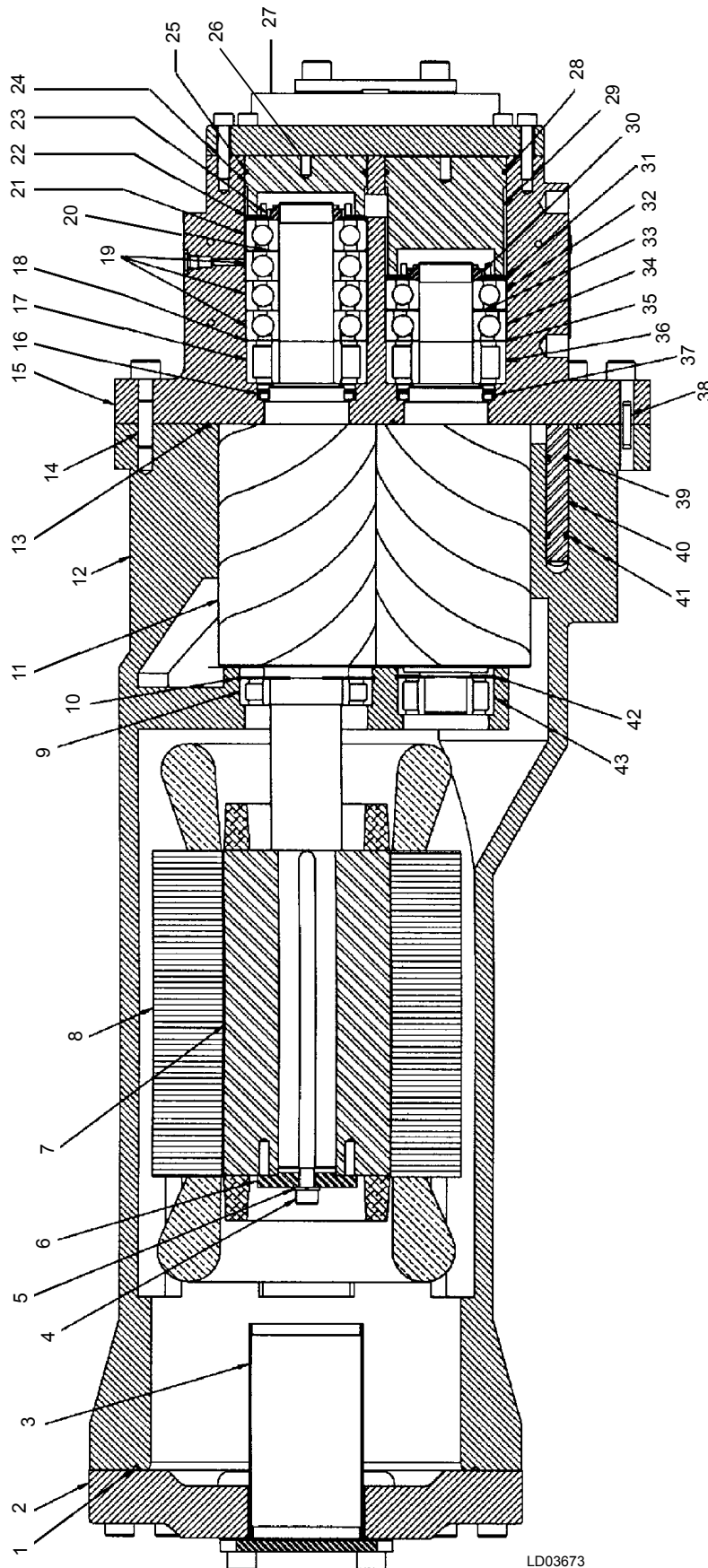
FIG. 49 – COMPRESSOR COMPONENTS
