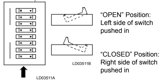
FIG. 56 – ENLARGED PHOTOGRAPH OF DIP SWITCHES ON MICROPROCESSOR BOARD
