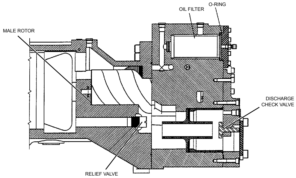
FIG. 48 – COMPRESSOR COMPONENTS
