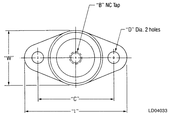
TYPE R OR RD IF BOLTING IS PREFERRED— Type R or RD mountings are furnished with a tapped hole in the center. This enables the equipment to be bolted securely to the mounting.
