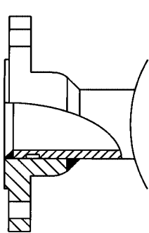
Weld Flange
