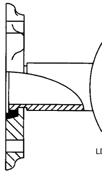
Victaulic Adapter
