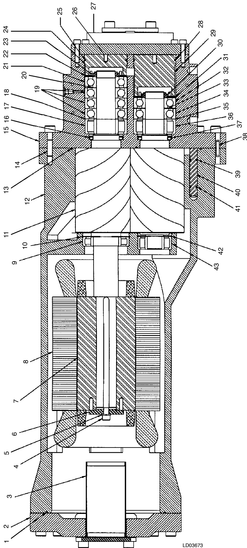
FIG. 43 – COMPRESSOR COMPONENTS
