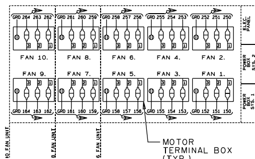
FIG. 50 – CONDENSER FAN CONTROL LAYOUT FOR DXST COMPRESSORS UNITS
