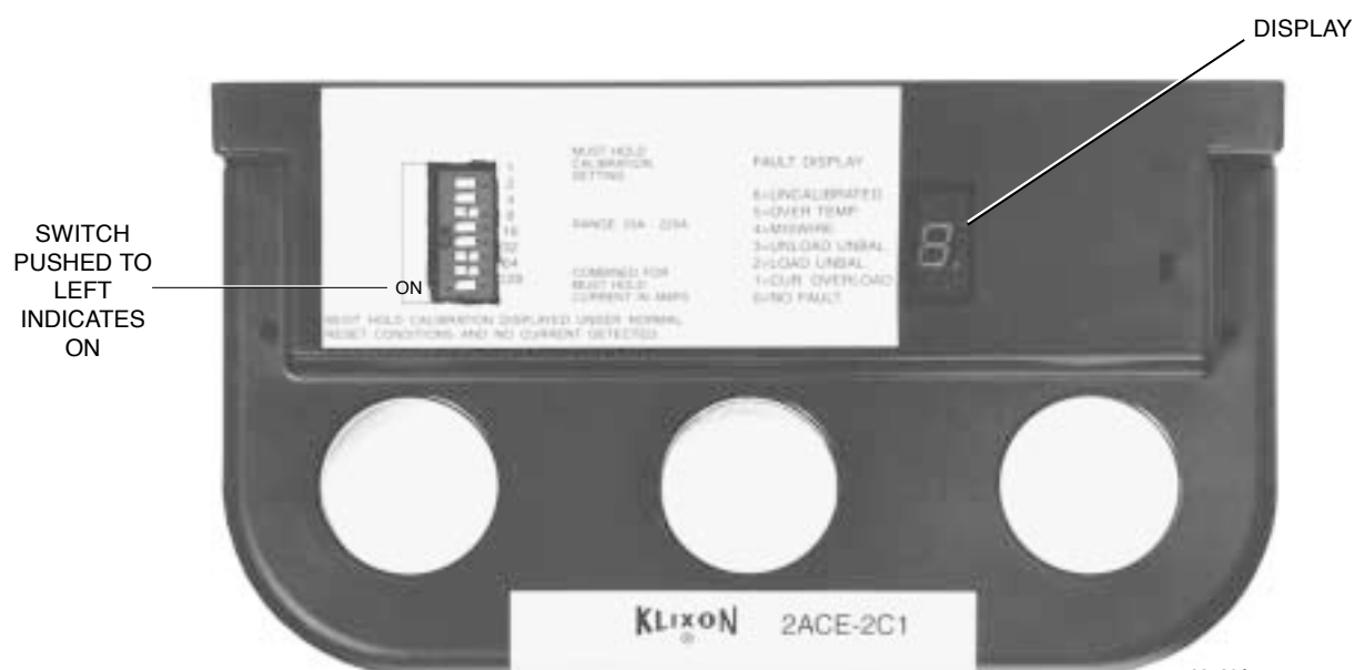
SIDE VIEW
