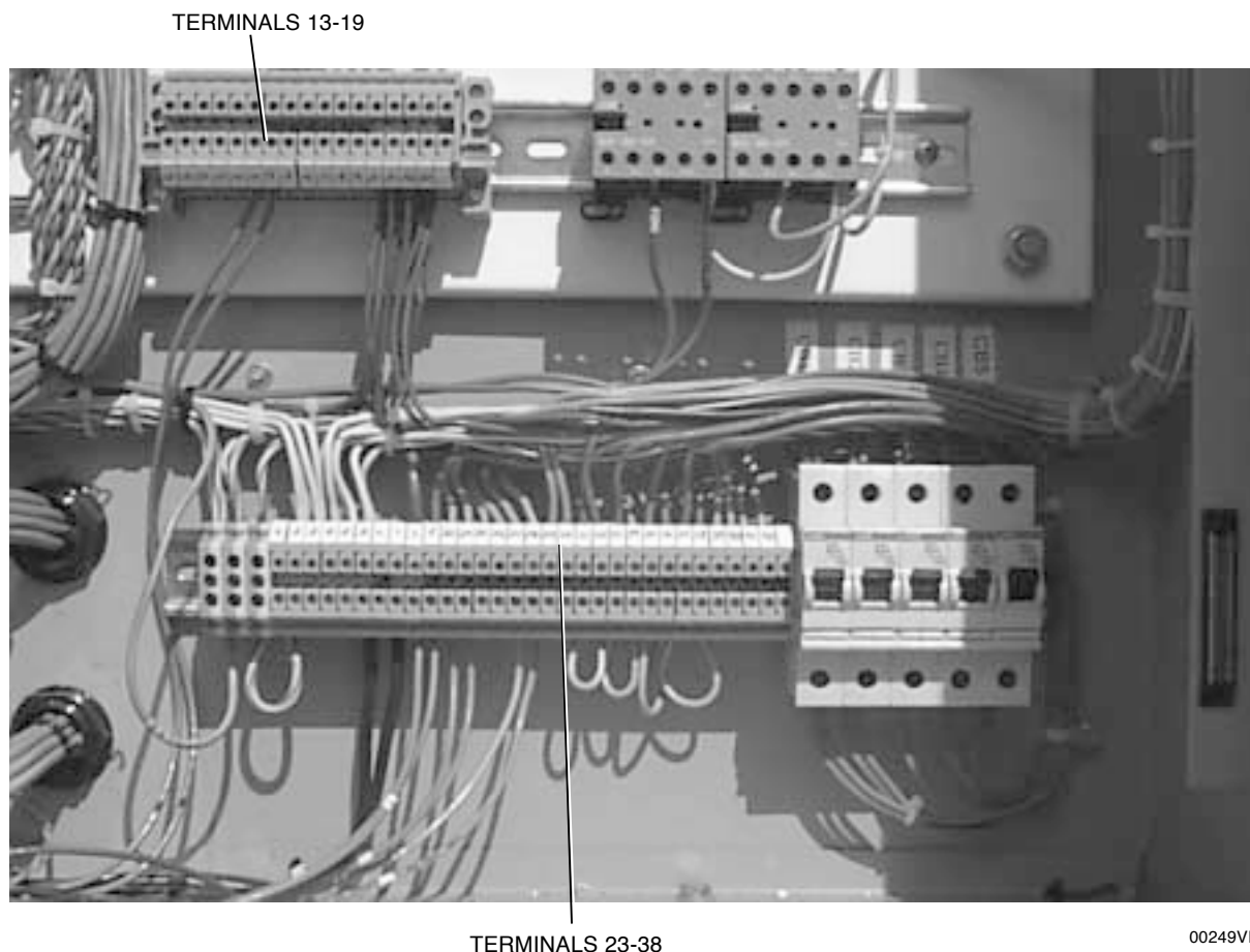
TERMINALS 23-38
