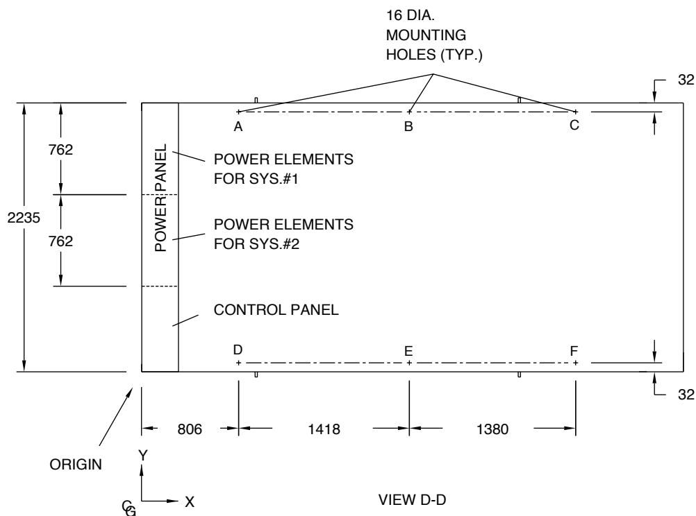
CENTER OF GRAVITY (Alum.)
