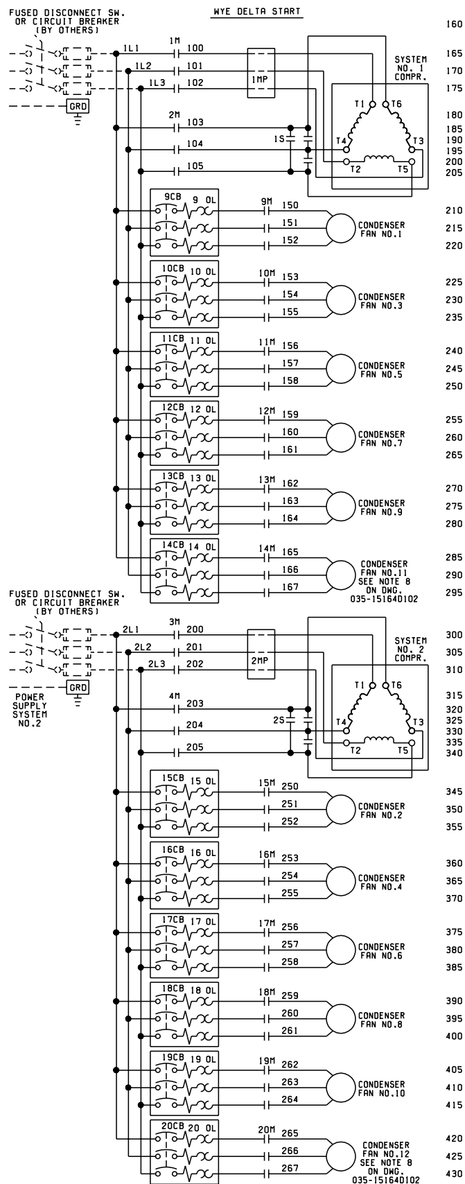
FIG. 20 – ELEMENTARY DIAGRAM – WYE-DELTA START
