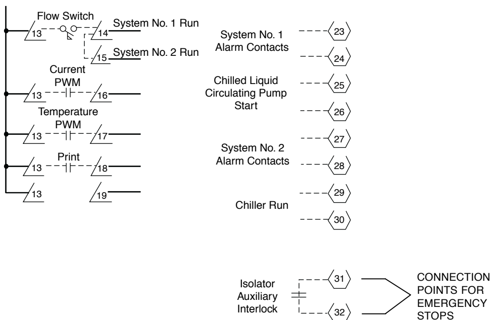
FIG. 12 – CUSTOMER CONNECTIONS
