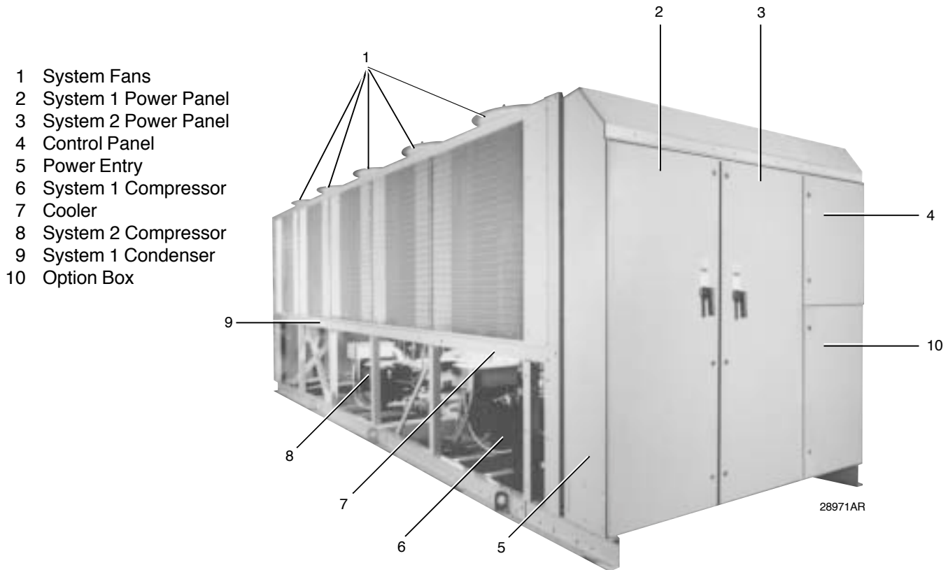
FIG. 1 – COMPONENT LOCATIONS
