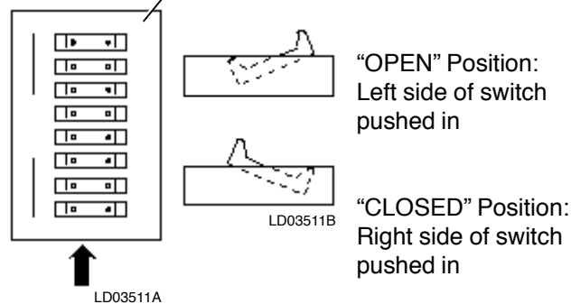
FIG. 49 – ENLARGED PHOTOGRAPH OF DIP SWITCHES ON MICROPROCESSOR BOARD
