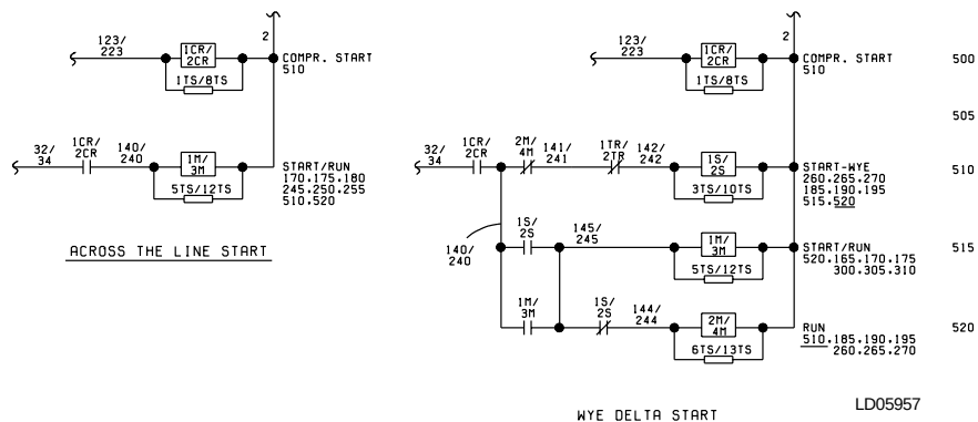
WYE DELTA START
