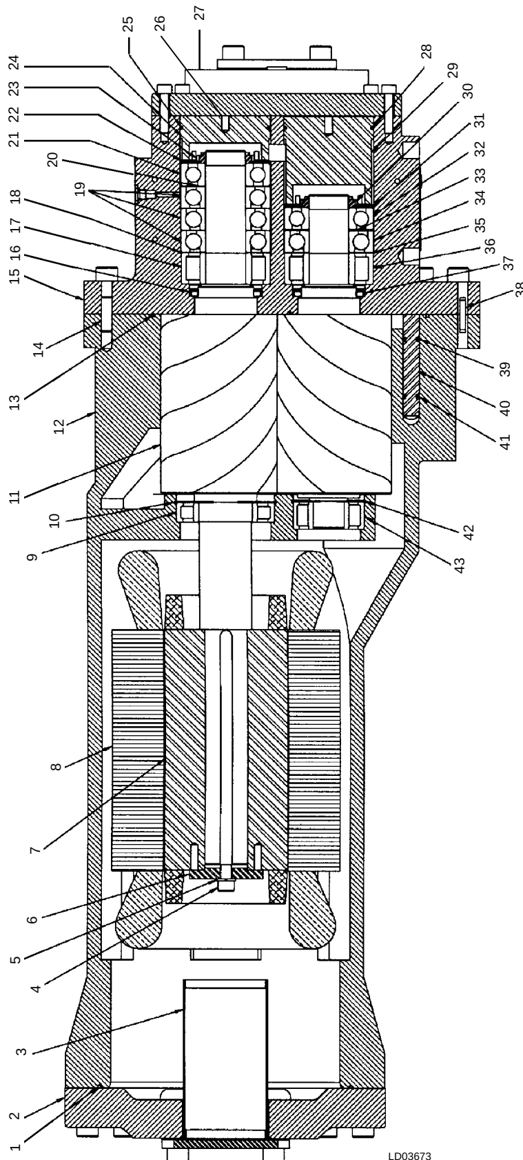
FIG. 34 – COMPRESSOR COMPONENTS
