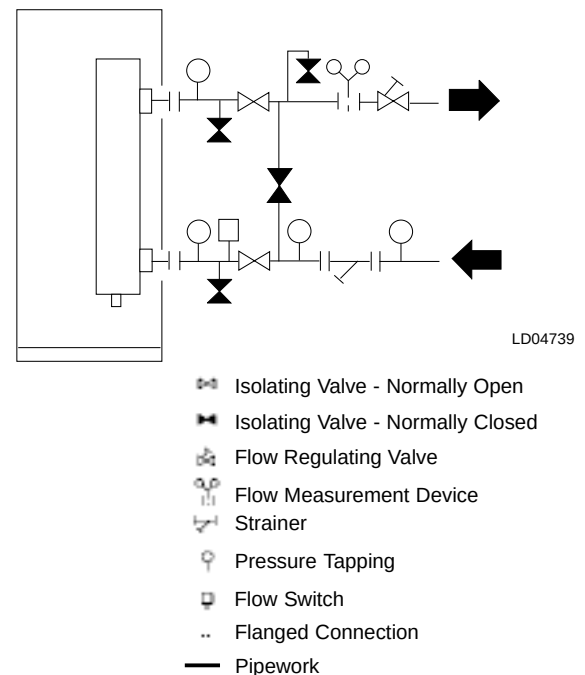
FIG. 5 – PIPEWORK ARRANGEMENT
