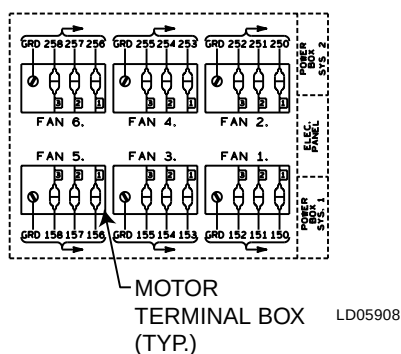
FIG. 41 – CONDENSER FAN CONTROL LAYOUT FOR DXST COMPRESSORS UNITS
