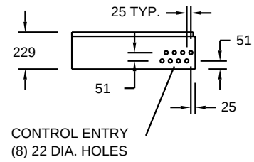
VIEW C-C
