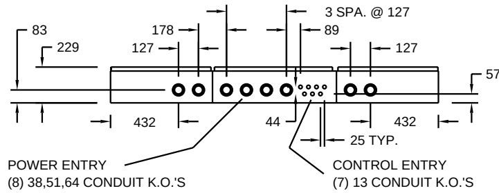
VIEW B-B
