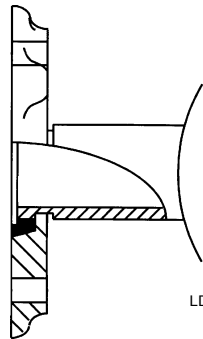
Victaulic Adapter
