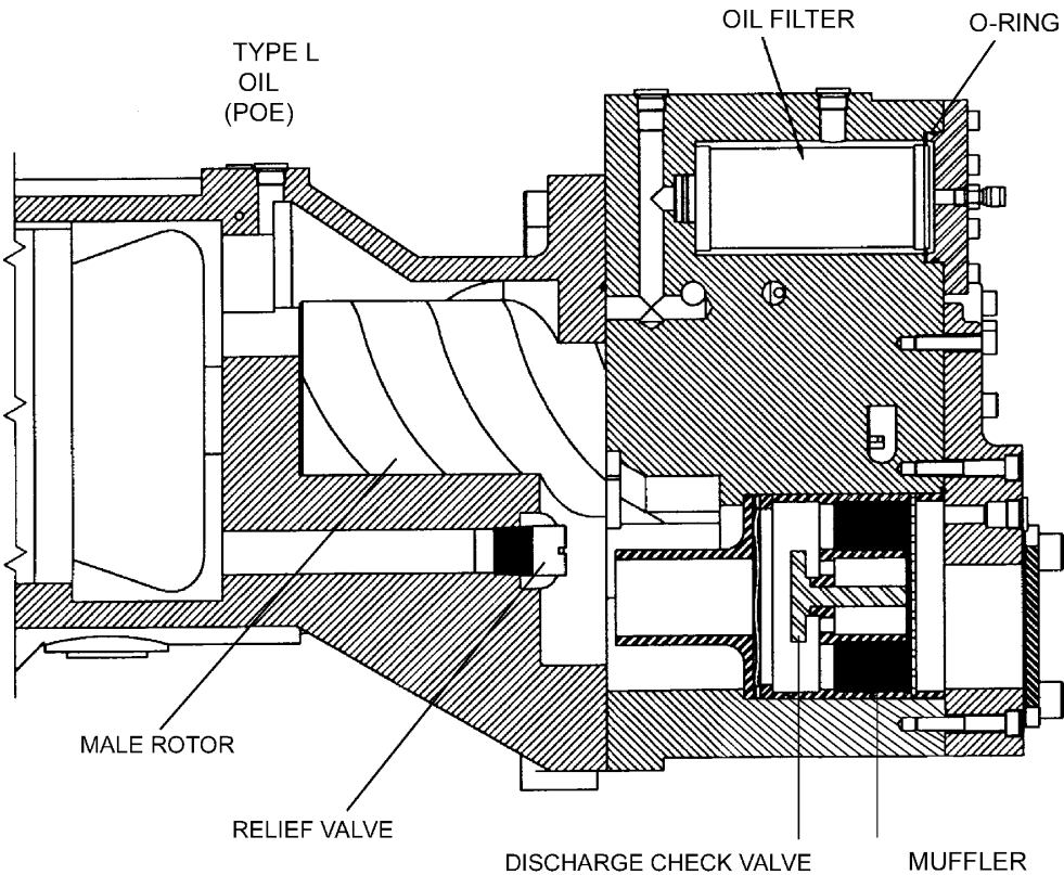
FIG. 33 – COMPRESSOR COMPONENTS
