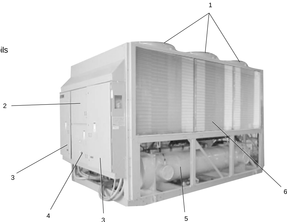
FIG. 1 – COMPONENT LOCATIONS
