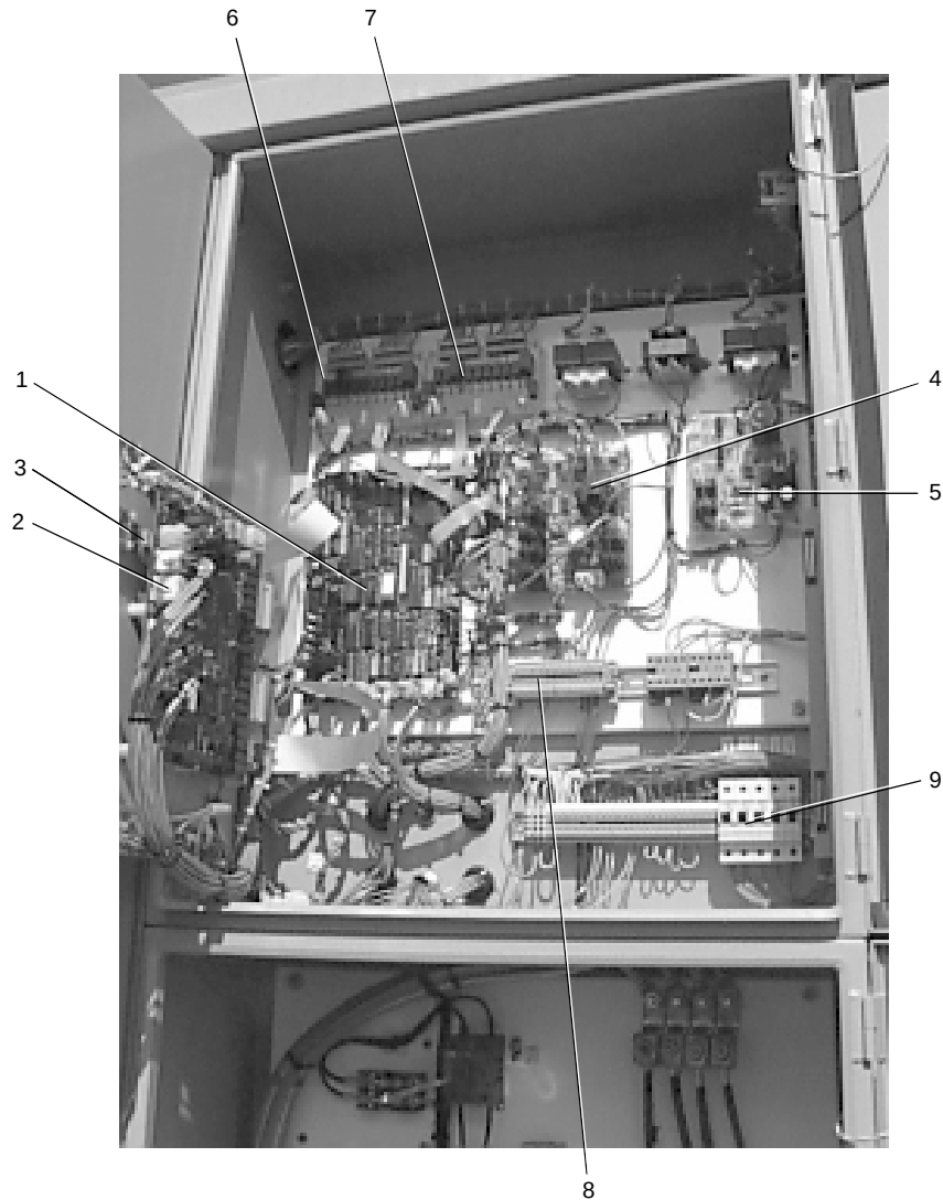
PHOTOGRAPH OF 50 HZ MODEL LOGIC SECTION
