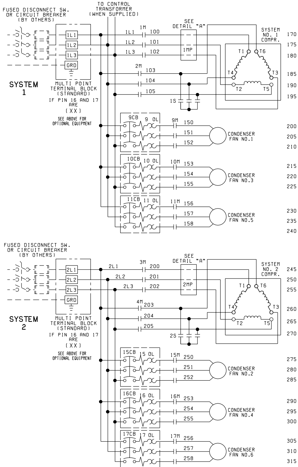
FIG. 17 – WIRING DIAGRAM – ACROSS-THE-LINE START
