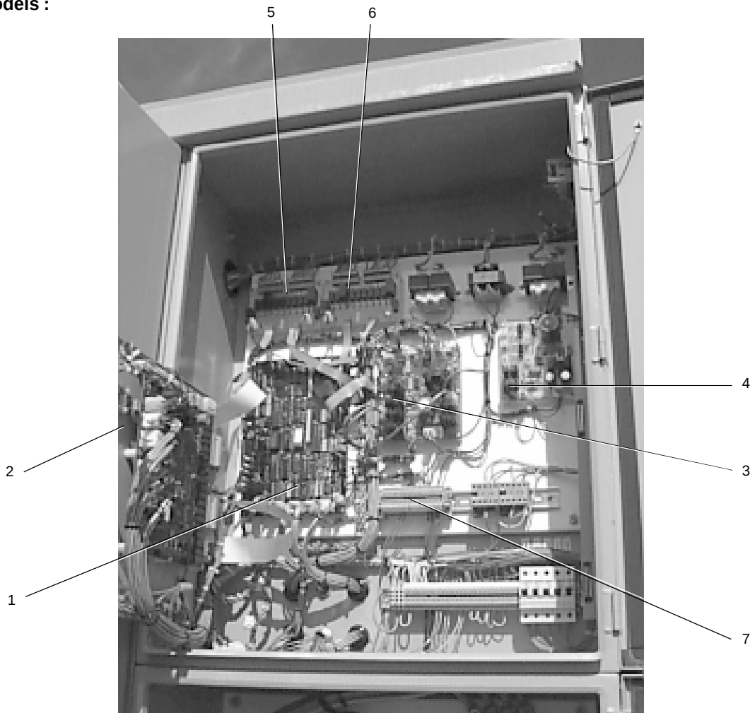
PHOTOGRAPH OF 50 HZ MODEL LOGIC SECTION
