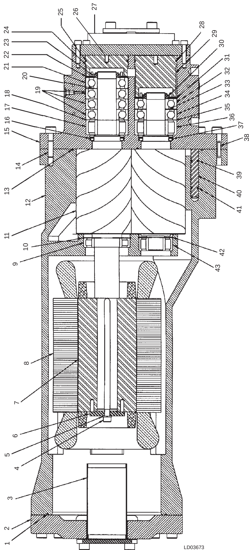
FIG. 38 – COMPRESSOR COMPONENTS
