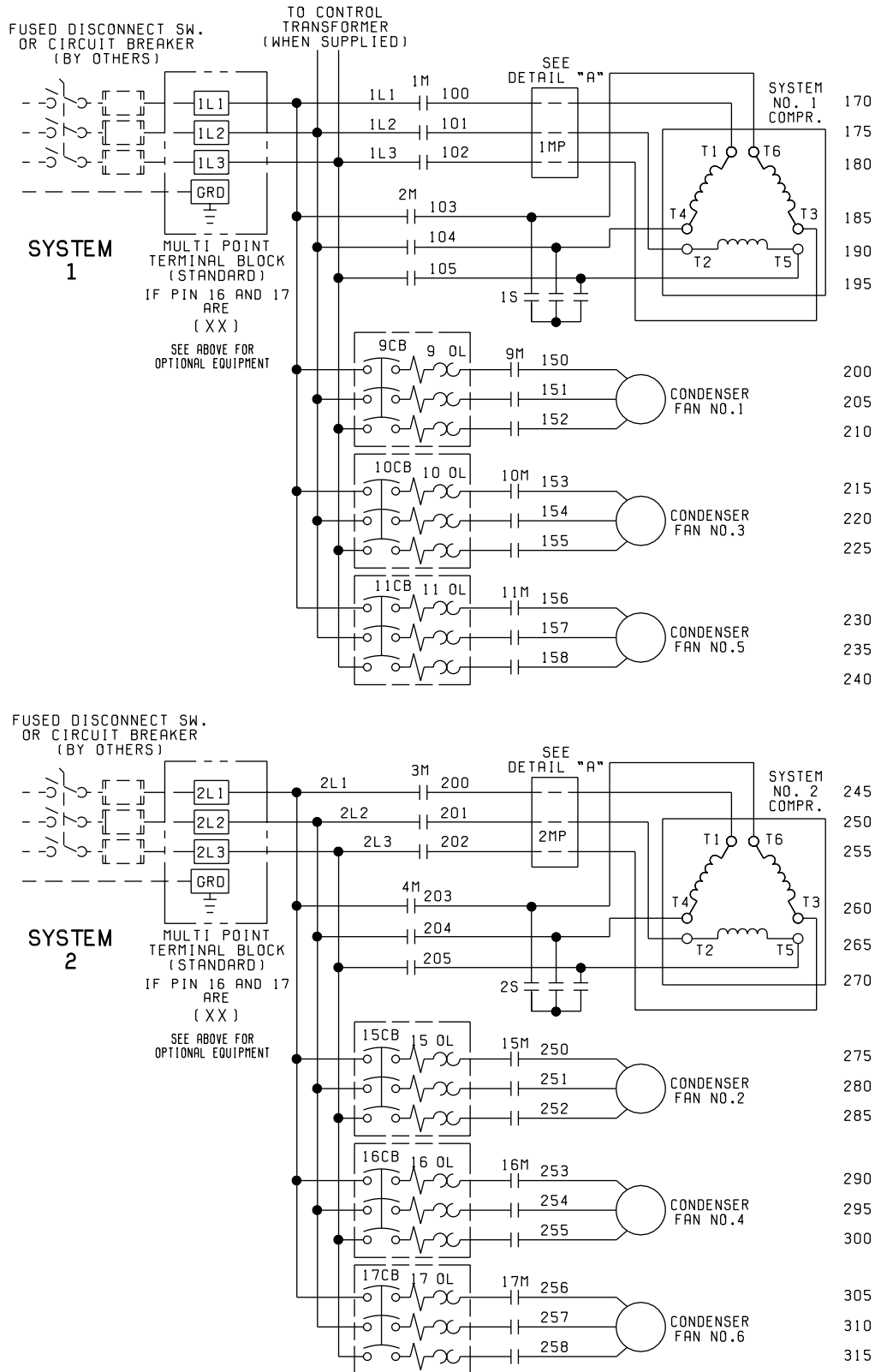
FIG. 17 – WIRING DIAGRAM – ACROSS-THE-LINE START
