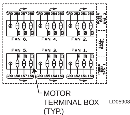
FIG. 45 – CONDENSER FAN CONTROL LAYOUT FOR DXST COMPRESSORS UNITS
