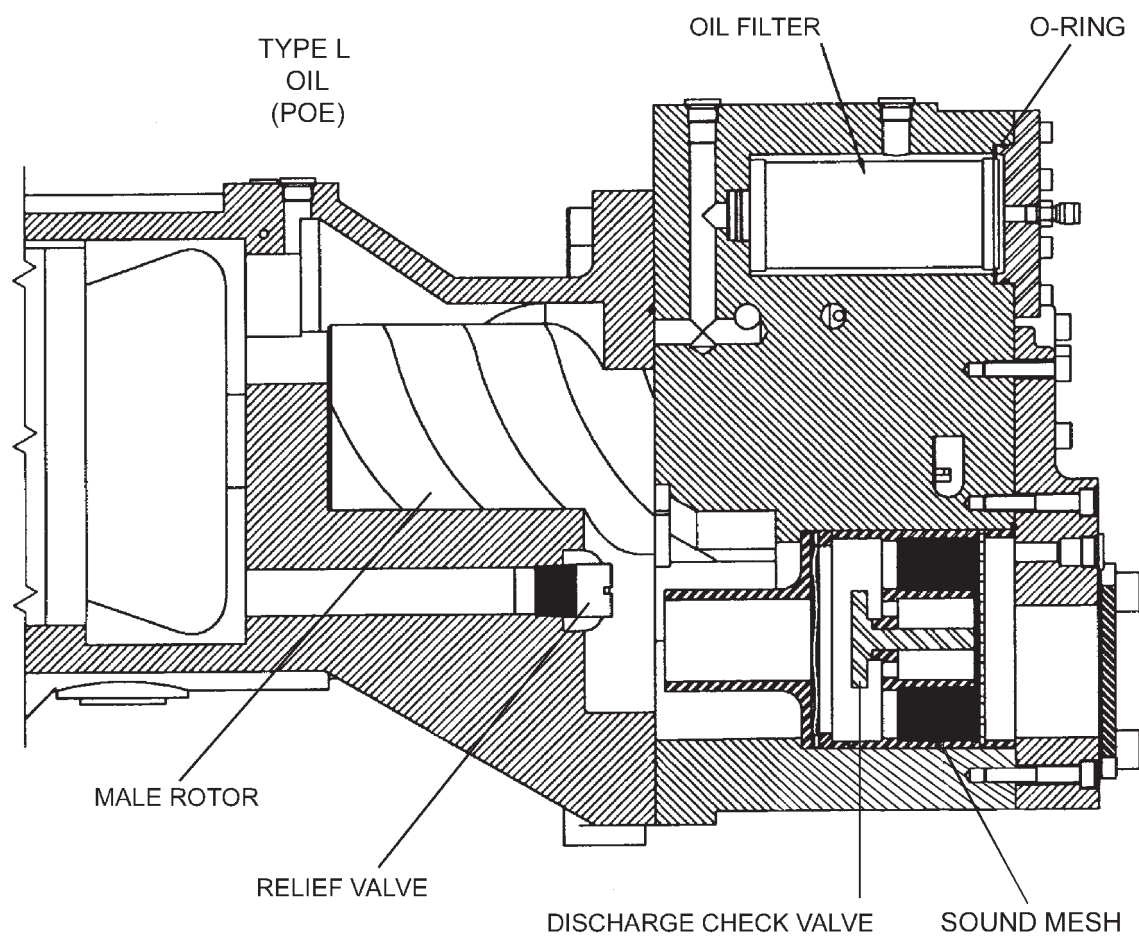
FIG. 37 – COMPRESSOR COMPONENTS
