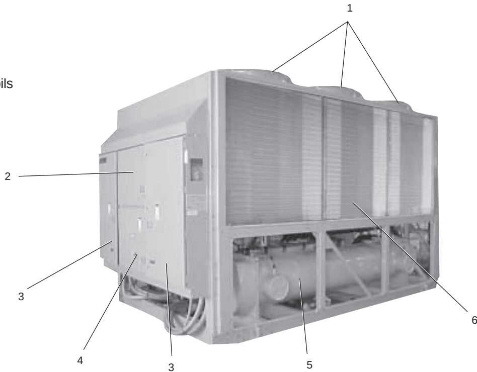
FIG. 1 – COMPONENT LOCATIONS
