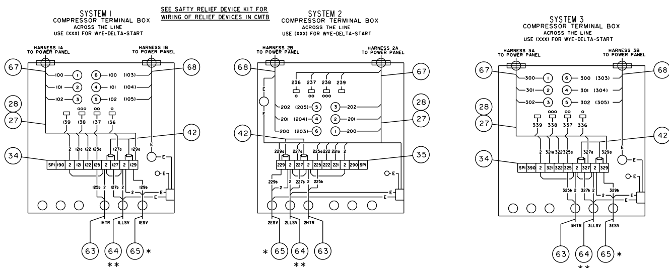
FIG. 34 – CONNECTION DIAGRAM SYSTEM WIRING
