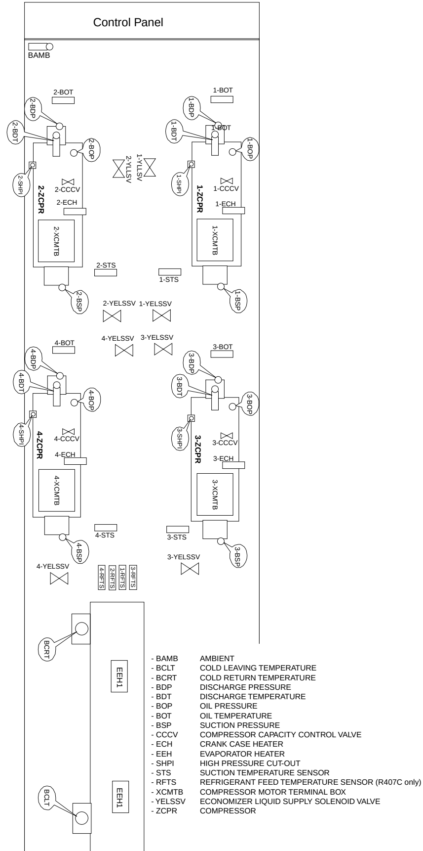
FIG. 55 – COMPONENT LOCATIONS (CONT'D)
