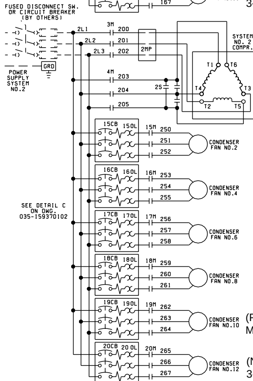
FIG. 21 – STANDARD 3 COMPRESSOR POWER SUPPLIES - WYE-DELTA START
