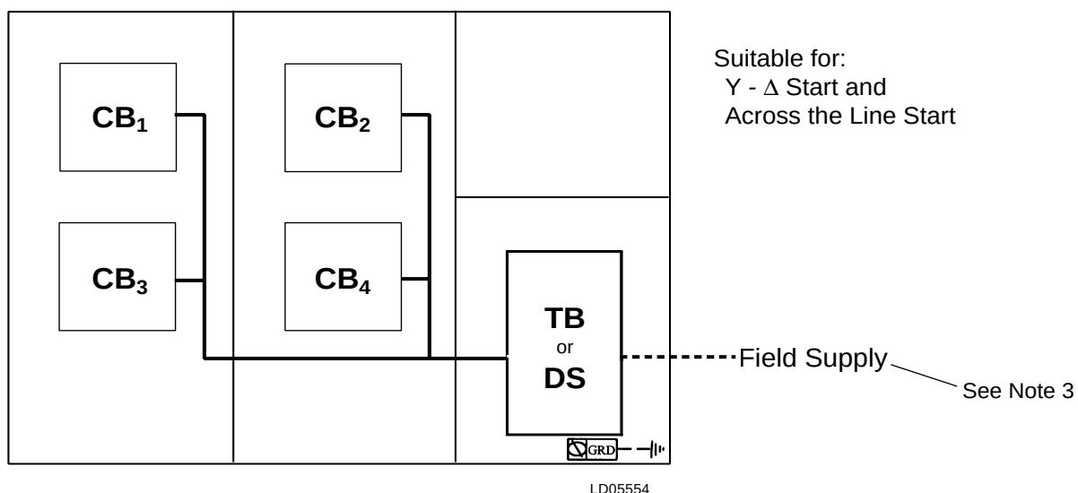
FIG. 17 – OPTIONAL SINGLE-POINT POWER SUPPLY CONNECTION WITH INDIVIDUAL SYSTEM CIRCUIT BREAKERS
