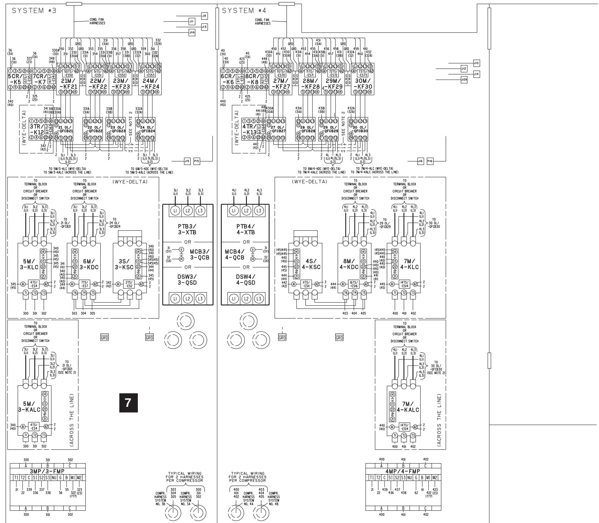
FIG. 42 – CONNECTION DIAGRAM
