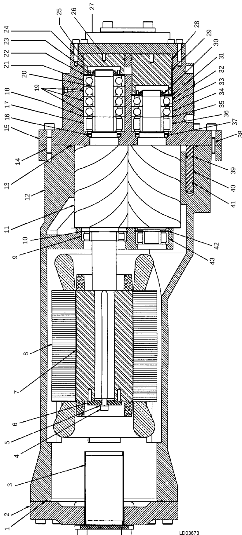
FIG. 61 – COMPRESSOR COMPONENTS
