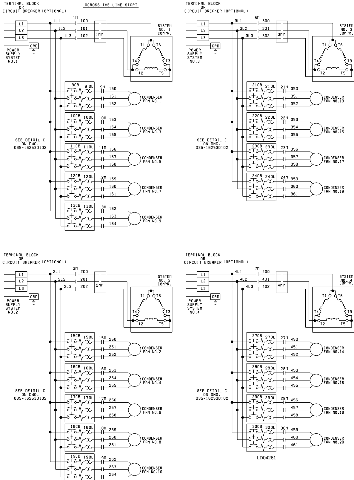
FIG. 39 – STANDARD POWER SUPPLY - ACROSS-THE-LINE START
