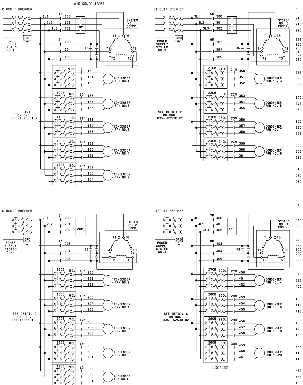
FIG. 38 – STANDARD POWER SUPPLY - WYE-DELTA START
