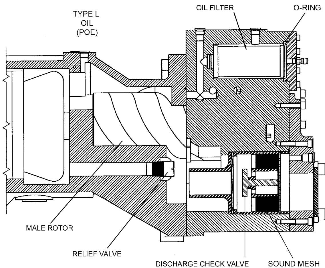
FIG. 59 – COMPRESSOR COMPONENTS
