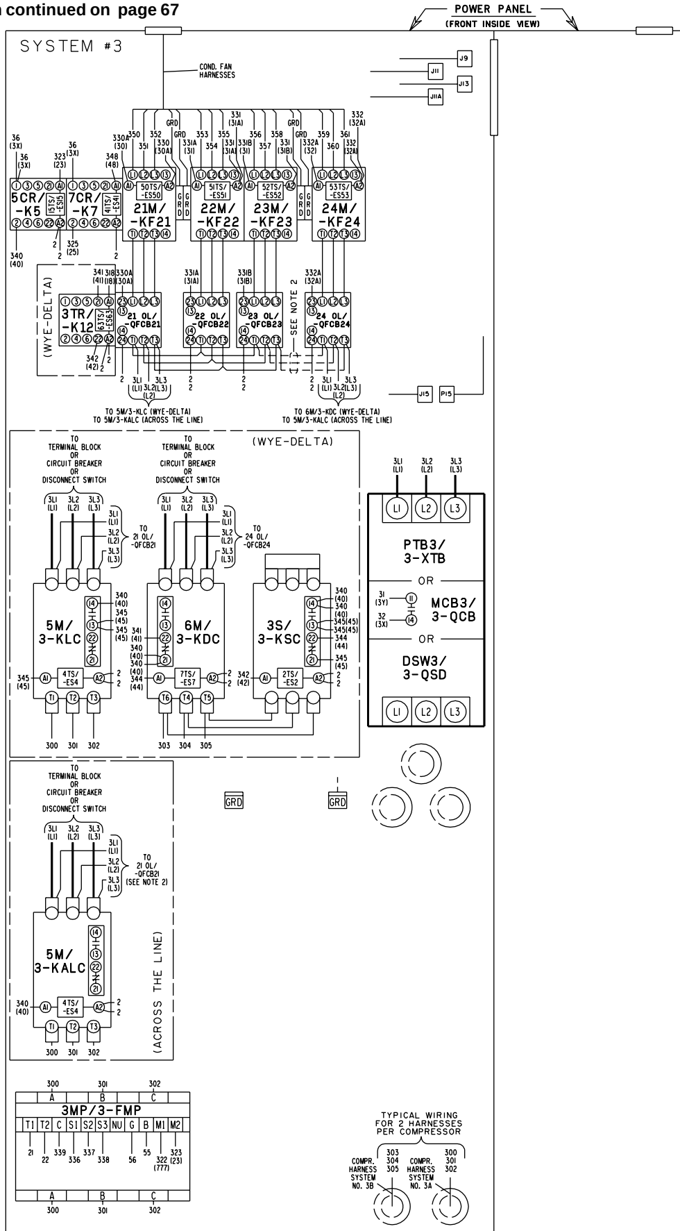
FIG. 25 – CONNECTION DIAGRAM
