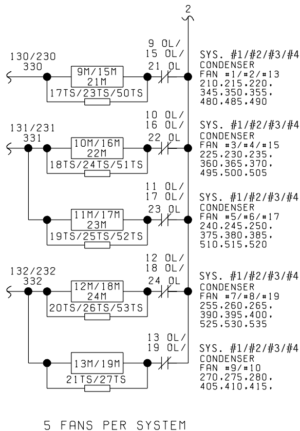
FIG. 32 – ELEMENTARY DIAGRAM, DXST DIRECT DRIVE - CONTROL CIRCUIT
