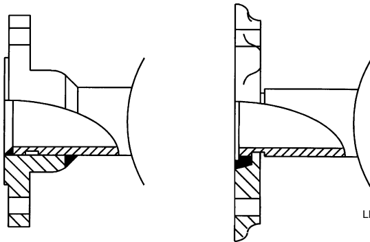
Weld Flange
