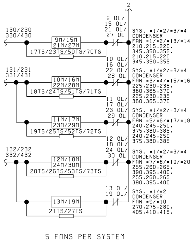
FIG. 47 – ELEMENTARY DIAGRAM, DXST DIRECT DRIVE - CONTROL CIRCUIT
