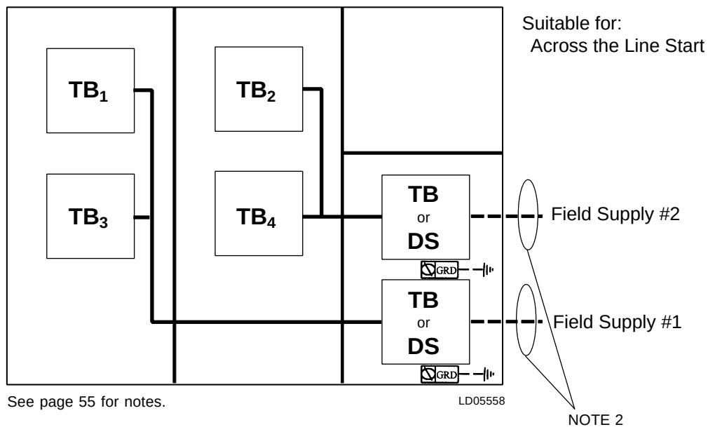
FIG. 15 – MULTIPLE POINT POWER SUPPLY CONNECTION
