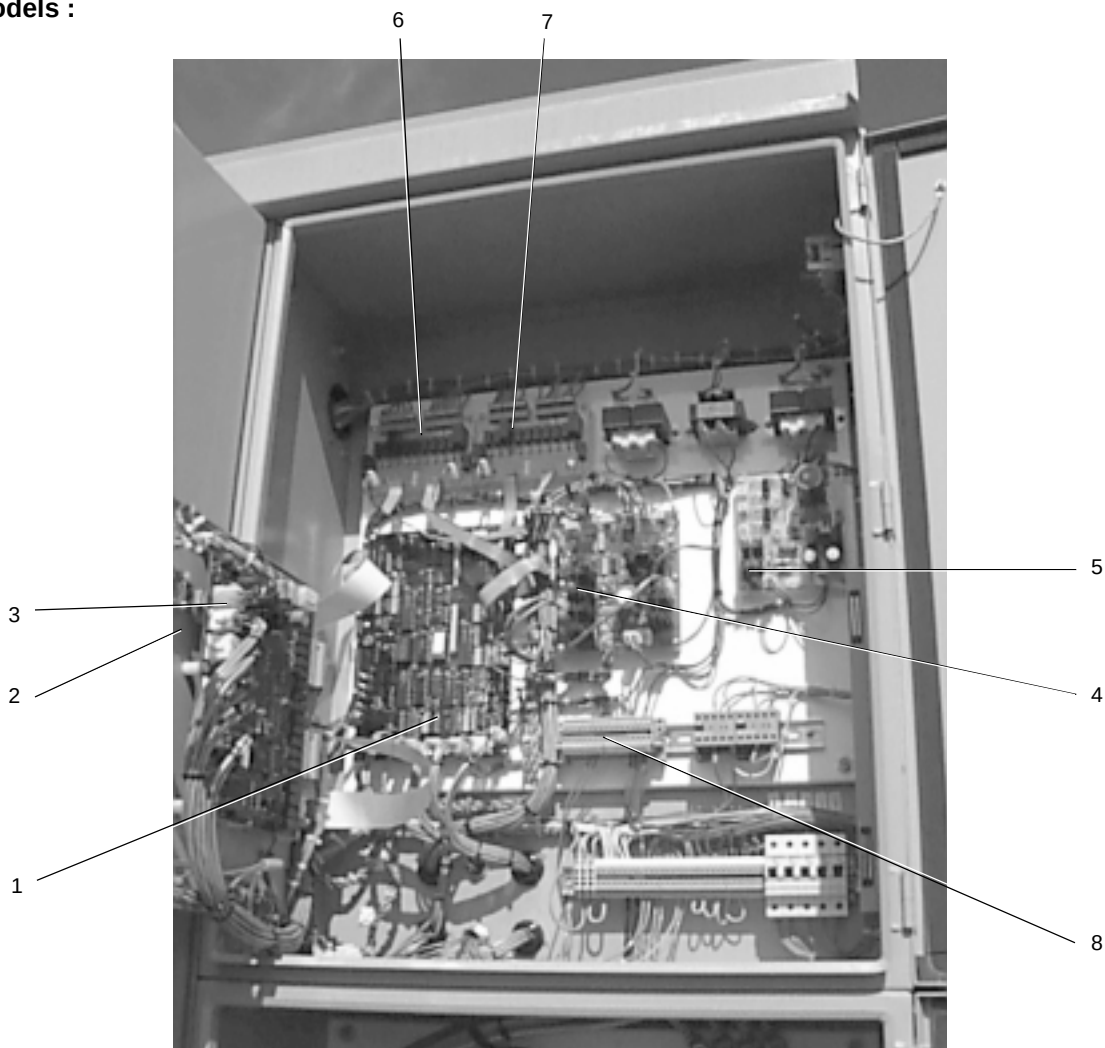
PHOTOGRAPH OF 50 HZ MODEL LOGIC SECTION
