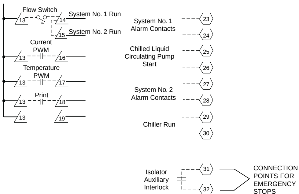
FIG. 11 – CUSTOMER CONNECTIONS
