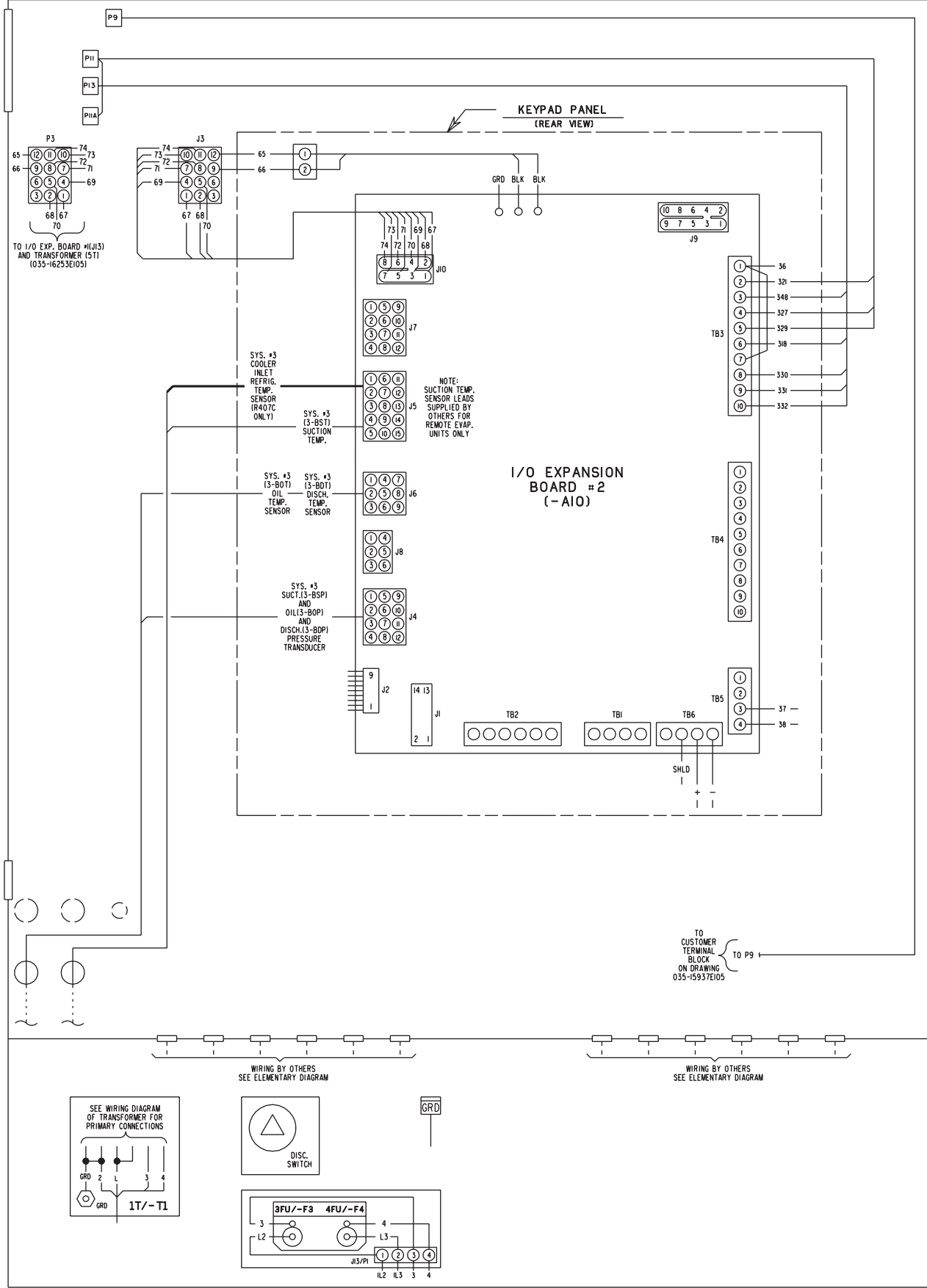
FIG. 26 – CONNECTION DIAGRAM
