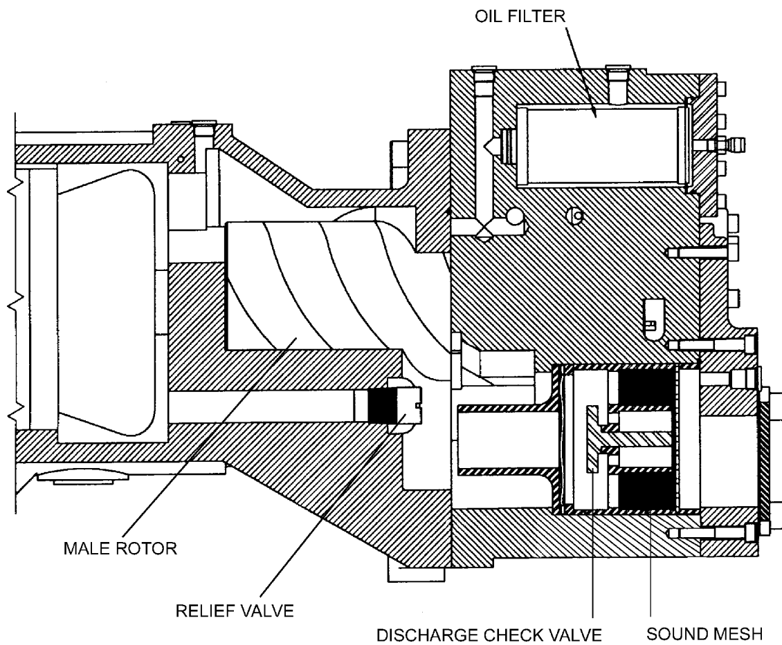
FIG. 36 – COMPRESSOR COMPONENTS
