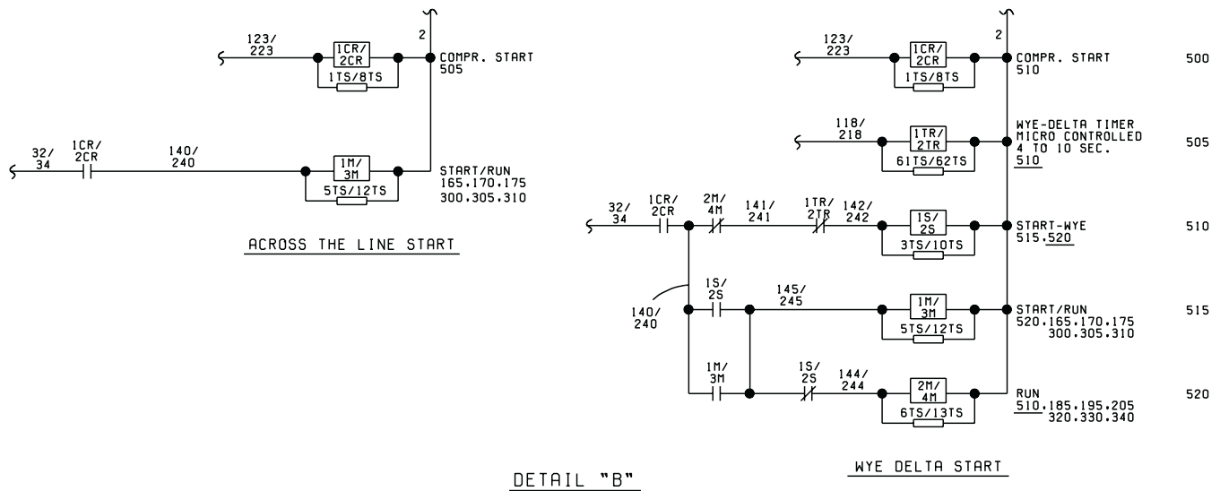
FIG. 24 – DETAIL "B"
