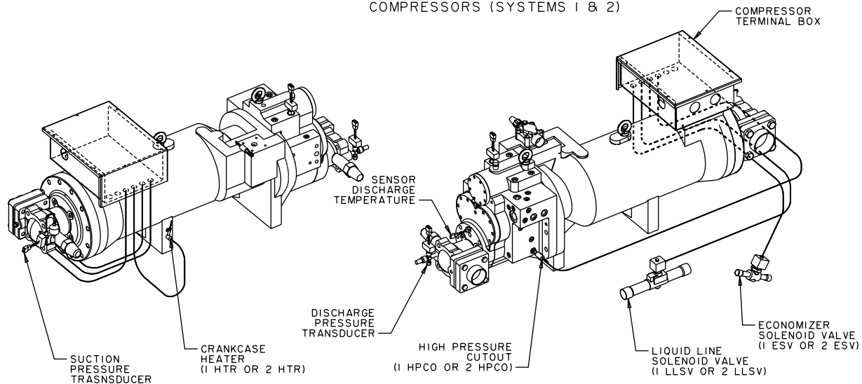
FIG. 22 – COMPRESSORS (SYSTEMS 1 & 2)
