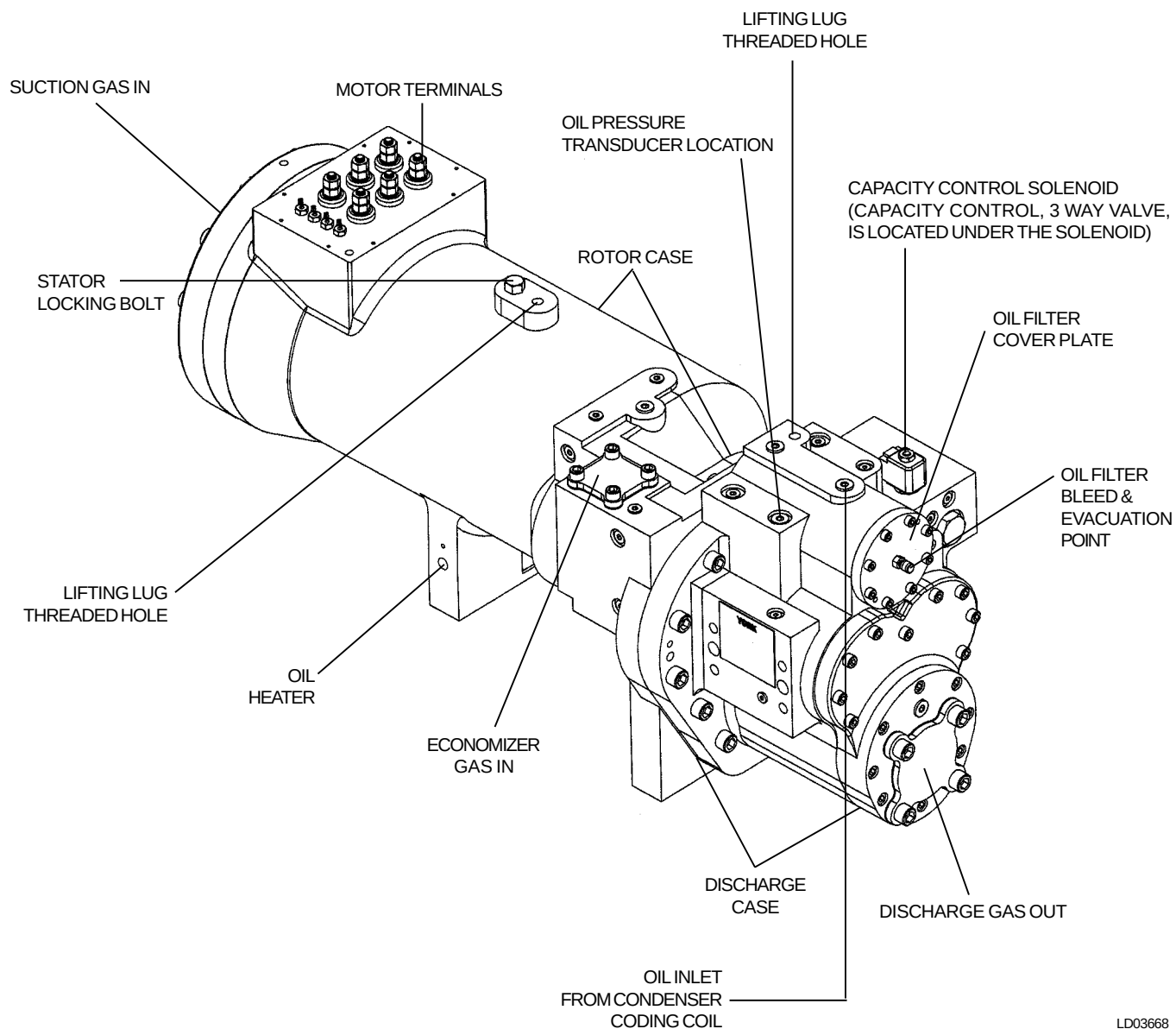
FIG. 33 – COMPRESSOR COMPONENTS
