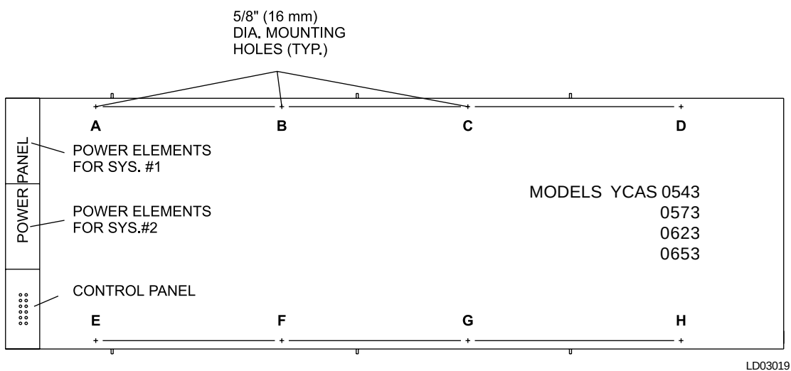
FIG. 28 – ISOLATOR LOCATIONS
