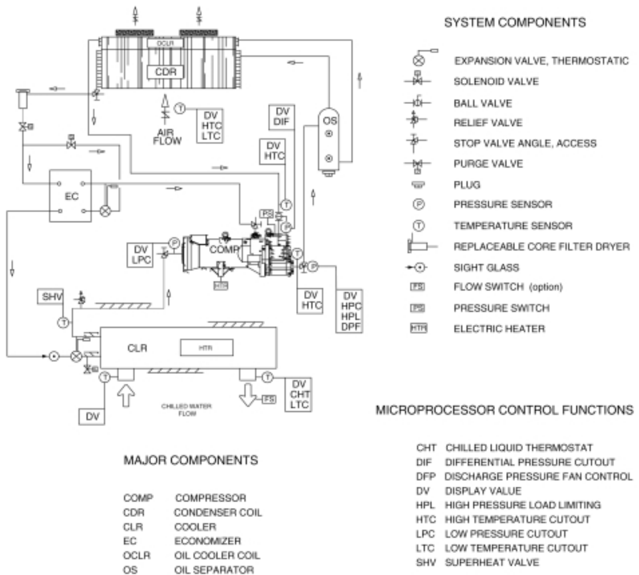
FIG. 31 – PROCESS AND INSTRUMENTATION DIAGRAM
