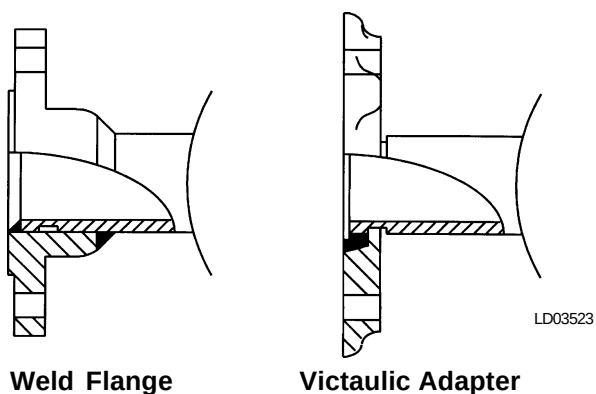
FIG. 7 – FLANGE ATTACHMENTS
