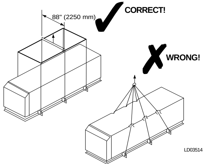
FIG. 3 – UNIT RIGGING
