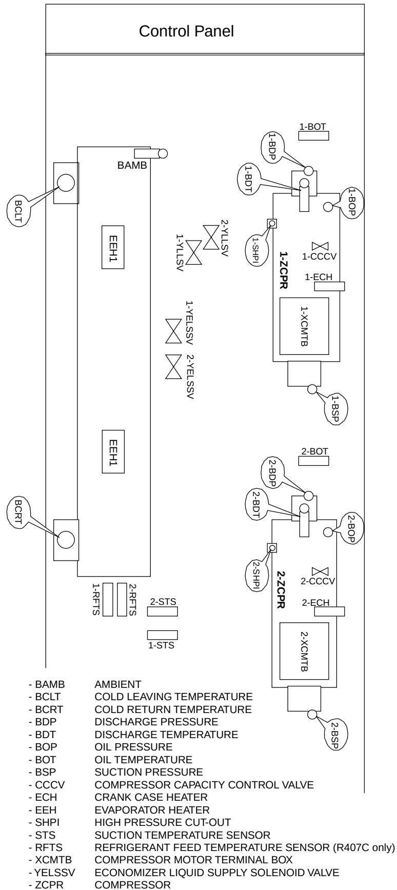
FIG. 32 – COMPONENT LOCATIONS
