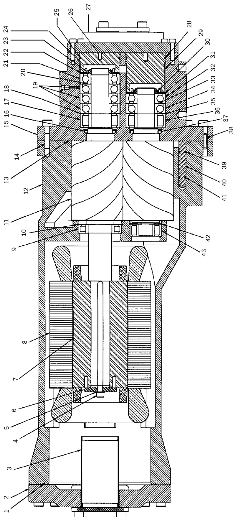
FIG. 38 – COMPRESSOR COMPONENTS
