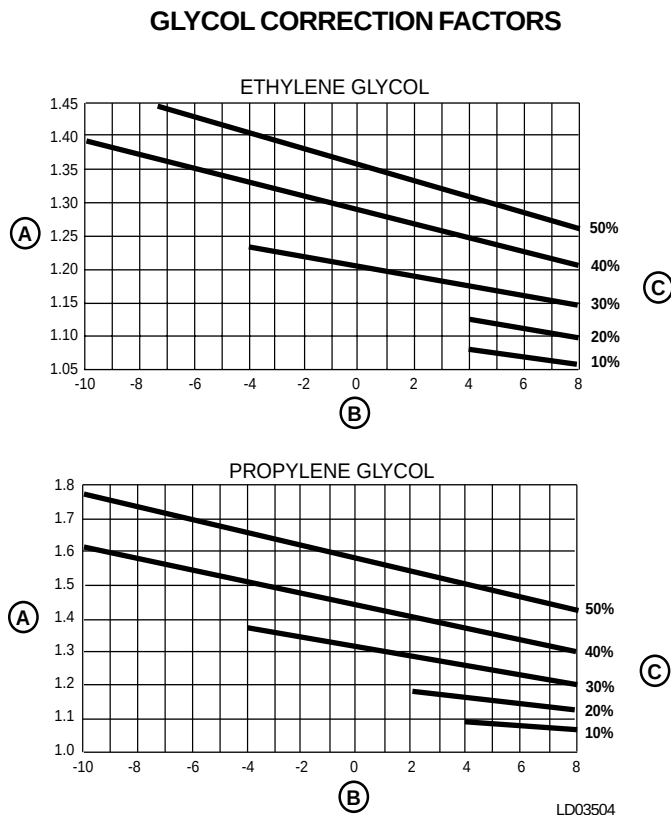
FIG. 11 – GLYCOL CORRECTION FACTORS
