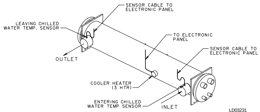
FIG. 21 – SENSOR CONNECTION
