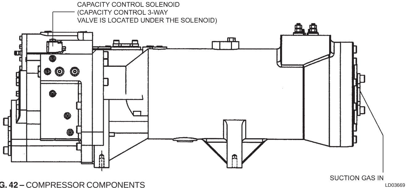
FIG. 42 – COMPRESSOR COMPONENTS
