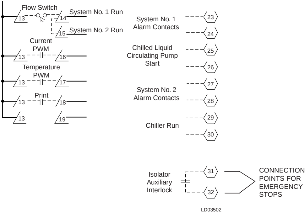
FIG. 12 – CUSTOMER CONNECTIONS
