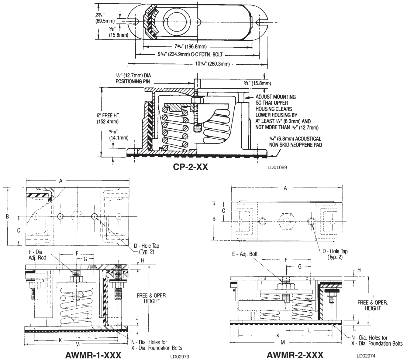
FIG. 37 – ISOLATOR DETAILS
