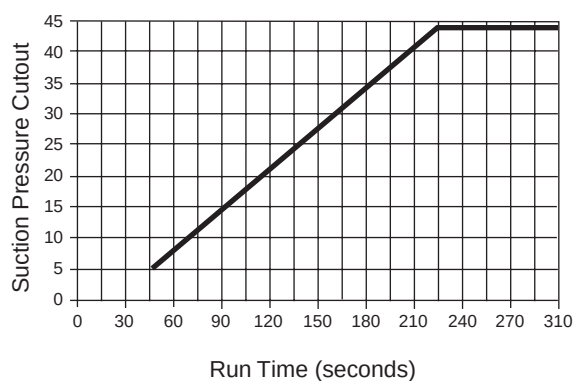
Suction Pressure Cutout With 44 PSIG Programmed Cutout
