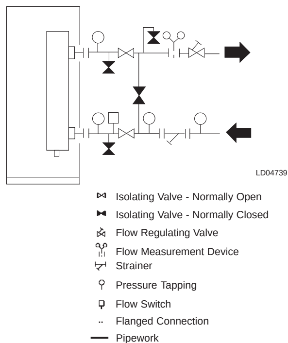
FIG. 5 – PIPEWORK ARRANGEMENT
