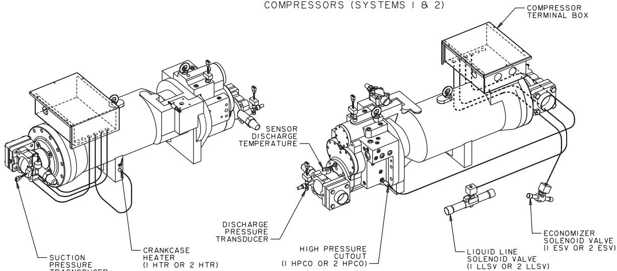
FIG. 28 – COMPRESSORS (SYSTEMS 1 & 2)
