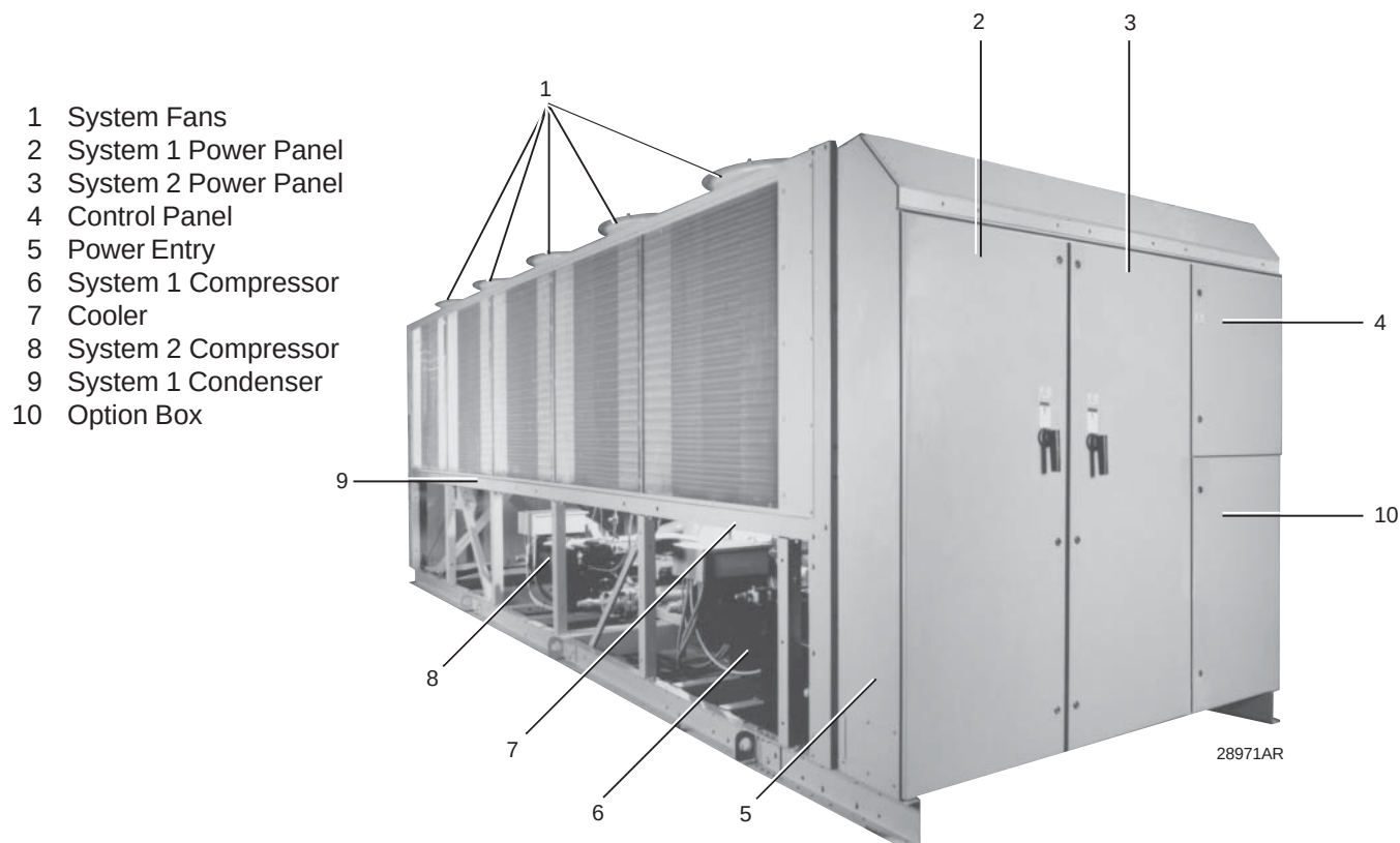
FIG. 1 – COMPONENT LOCATIONS
