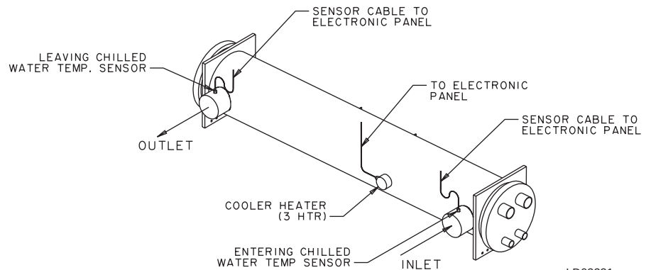
FIG. 27 – SENSOR CONNECTION
