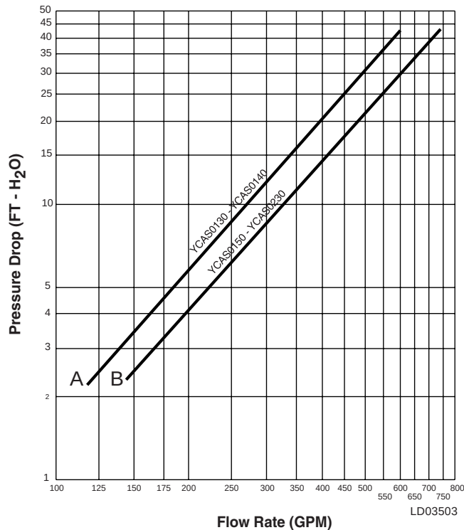
FIG. 14 – FLOW RATE AND PRESSURE DROP CHARTS
