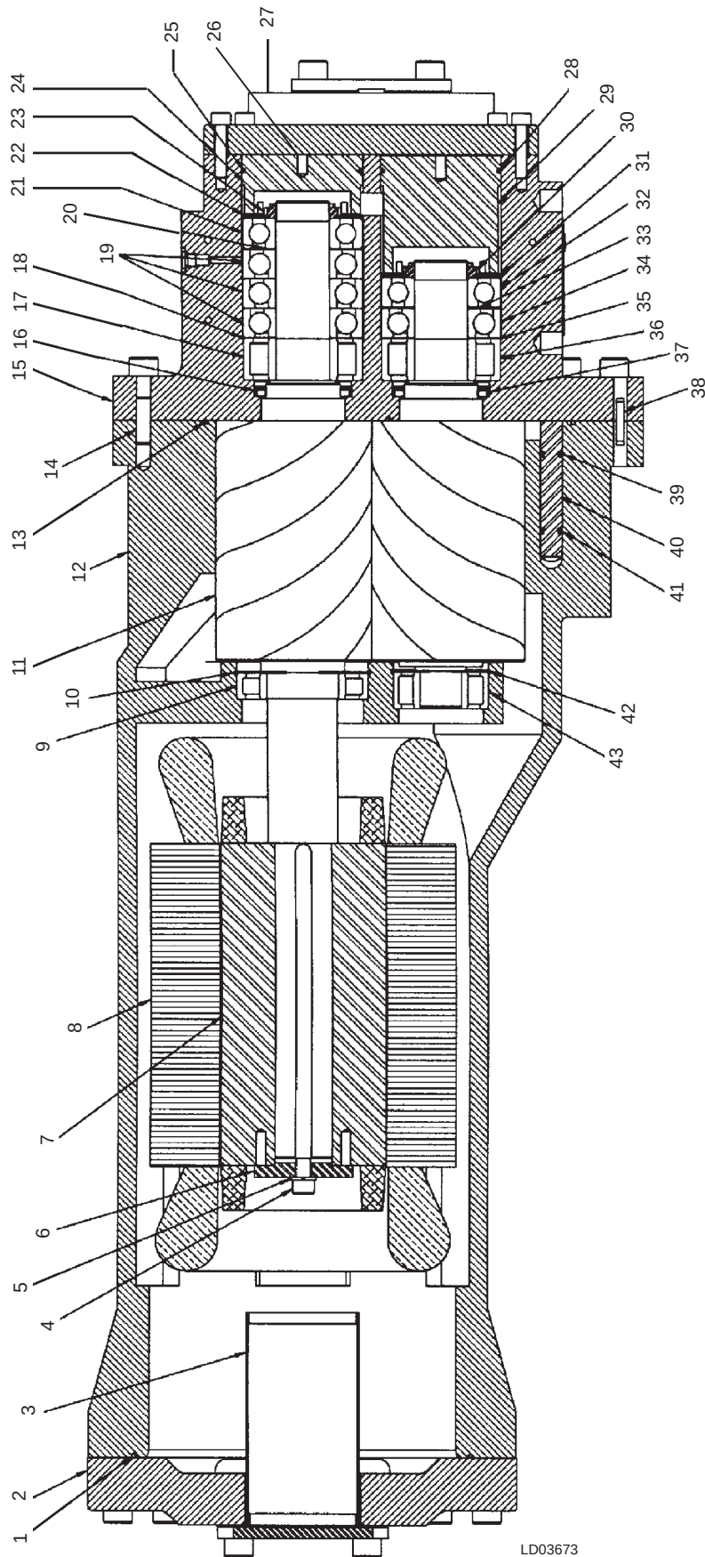
FIG. 45 – COMPRESSOR COMPONENTS
