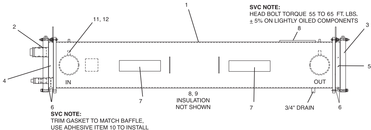
FIG. 1 – EVAPORATOR COMPONENTS
