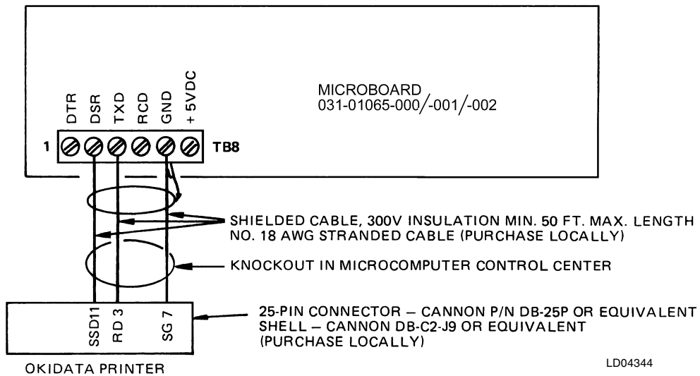
FIG. 11 – PRINTER INTERFACE ADAPTER FOR OKIDATA PRINTER
