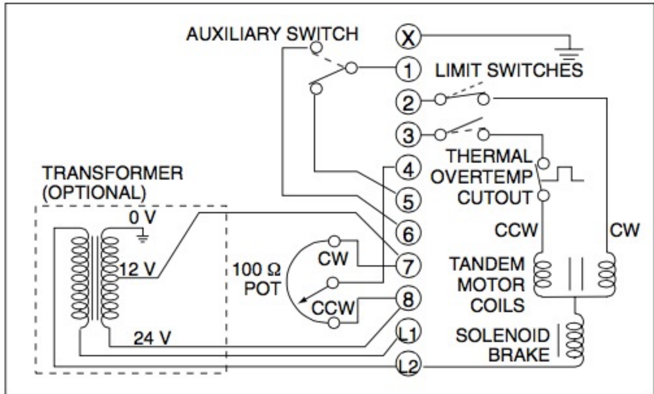
Figure 6. Internal Wiring
