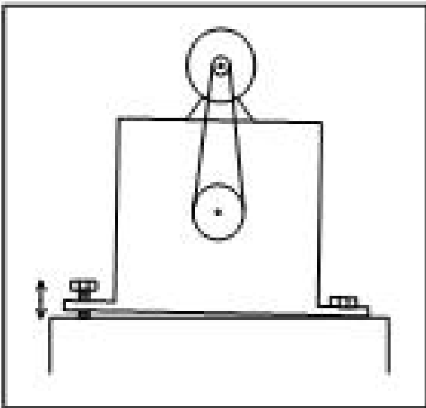
Figure 6: Machine with a loose mounting bolt.
