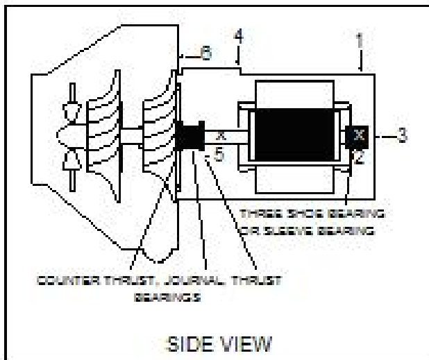
Figure 8: This Carrier 19C chiller requires six measurements points for data collection.
