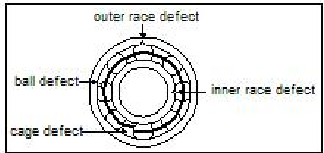
Figure 11: Typical defects on a rolling element bearing.
