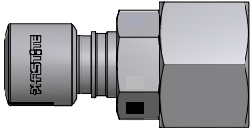
TFS-K Termination Female Straight - BSPT page 24
