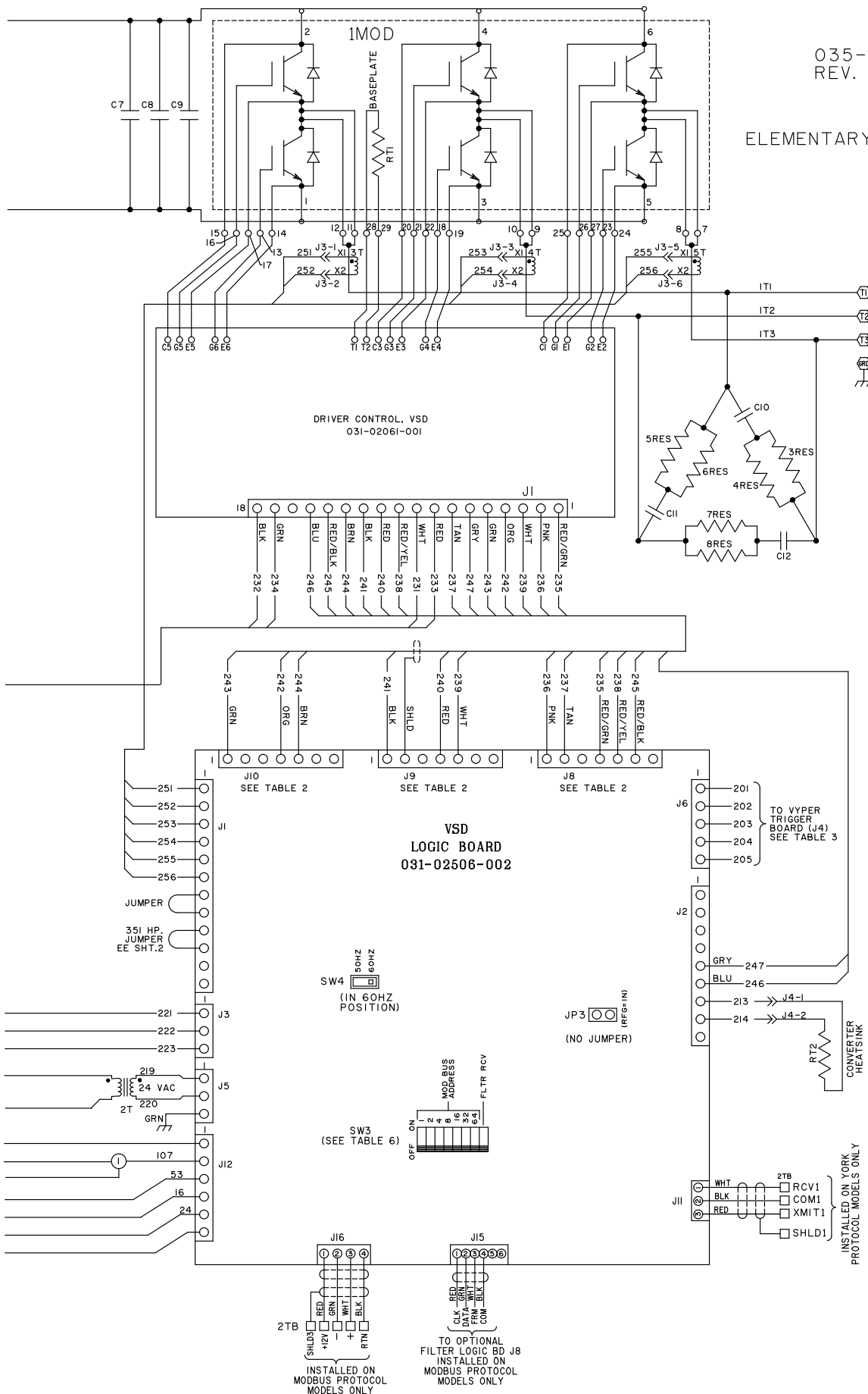
FIG. 1 (CONT'D) - ELEMENTARY WIRING DIAGRAM 292 & 351 HP
