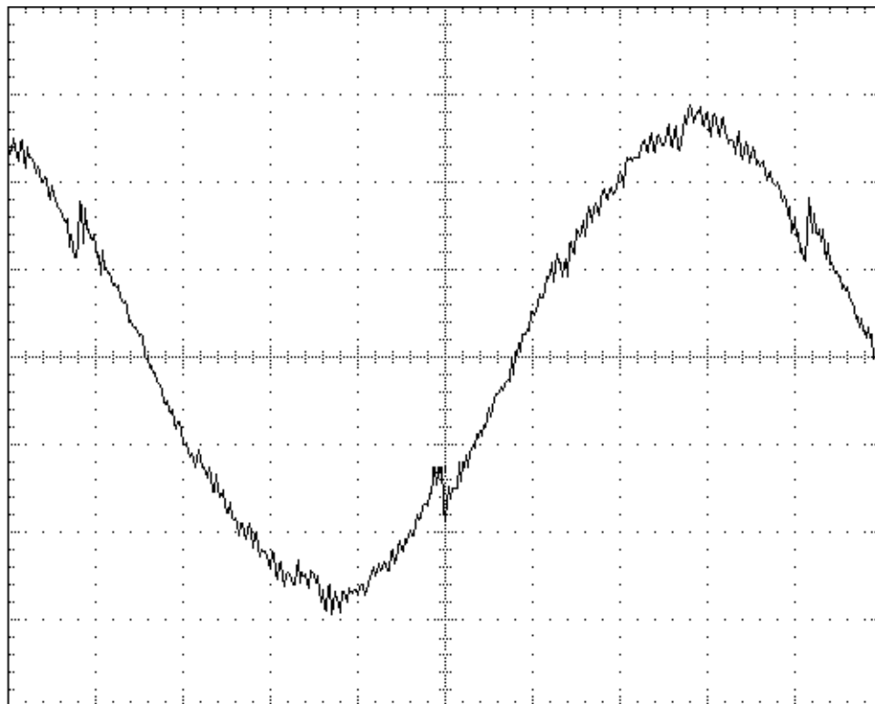
FIG. 7B – VSD INPUT CURRENT WITH FILTER
