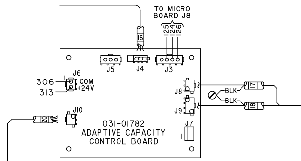
FIG. 12 – ADAPTIVE CAPACITY CONTROL BOARD FOR OPTIVIEW CONTROL CENTER
