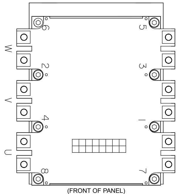
SCREWS TO BE TORQUED IN SEQUENCE - 1, 2, 3, 4, 5, 6, 7, 8 LD07412
