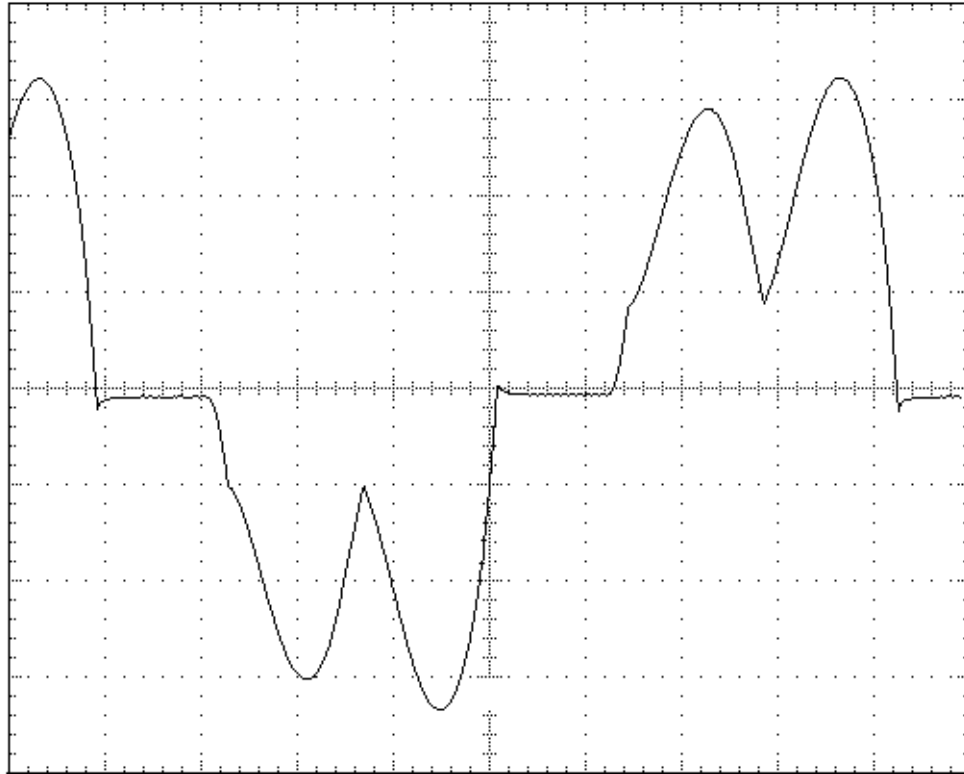
FIG. 7A – VSD INPUT CURRENT WITHOUT FILTER
