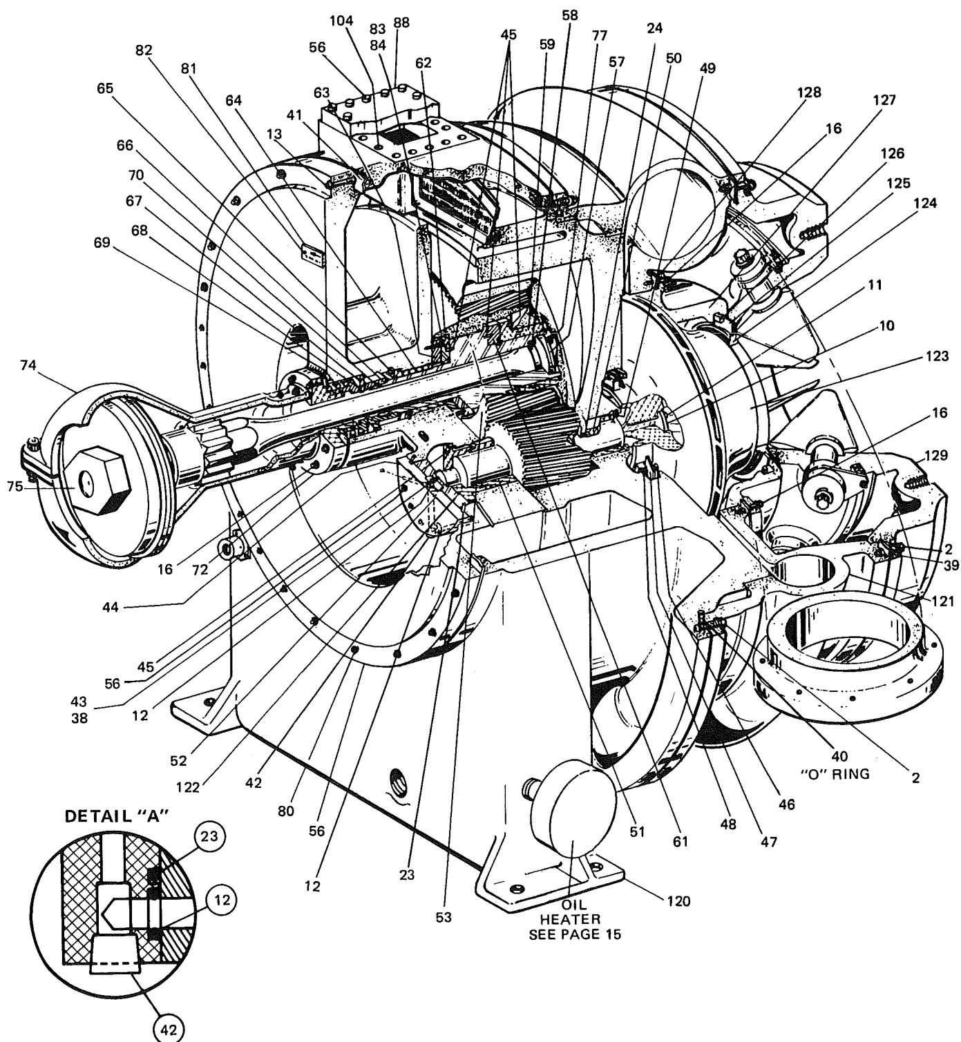
FIG. 2 — MODEL LKC65 & LKC73 COMPRESSORS, PARTS LOCATION
