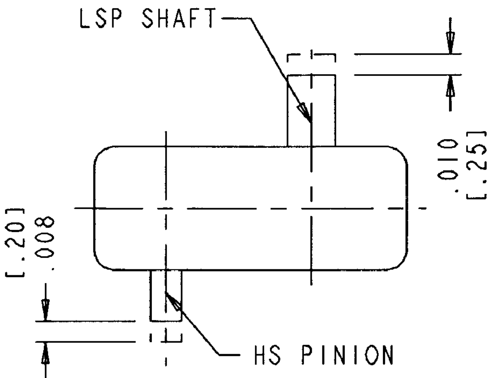
DETAIL - AXIAL THERMAL GROWTH (ALIGNMENT VALUES BASED ON 60° F [33° C] TEMPERATURE RISE ABOVE AMBIENT)
