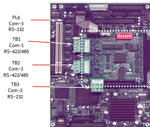
Serial Communications Port Locations
