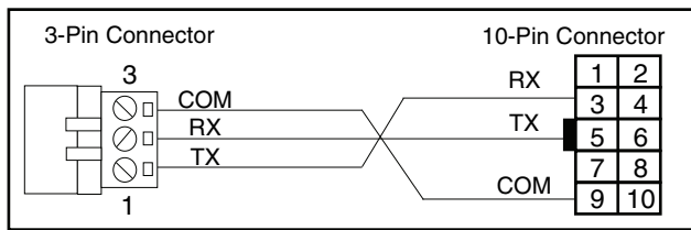
RS-232 Test Harness
