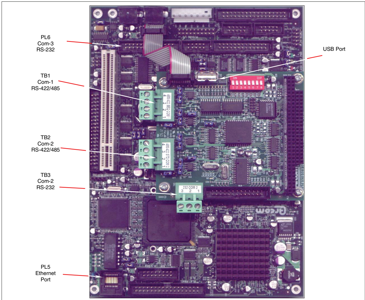
Quantum™ 4 Main and Communications Boards
