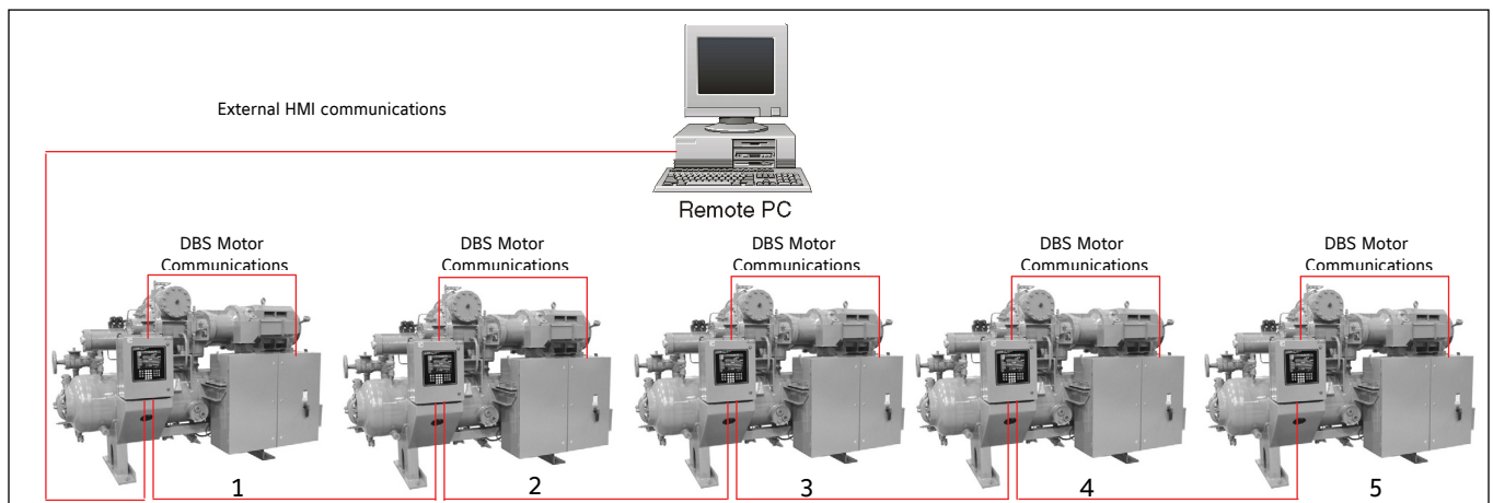
Typical Serial Wiring Scenario including optional DBS Motor Starter
