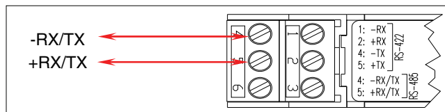
RS-485 Connections
