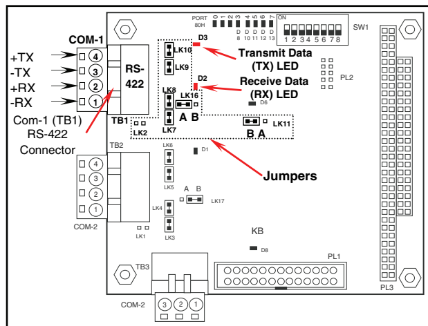
RS-422 Com-1 (TB1) Connector, Jumpers and LED Location
