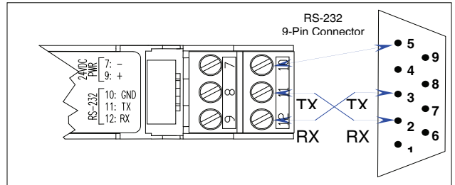
RS-232 Connections
