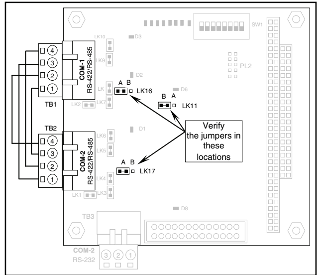
RS-422 Test Configuration
