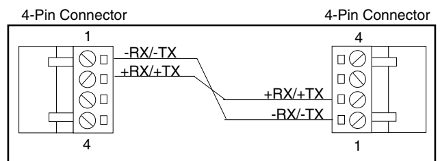
RS-485 Test Harness
