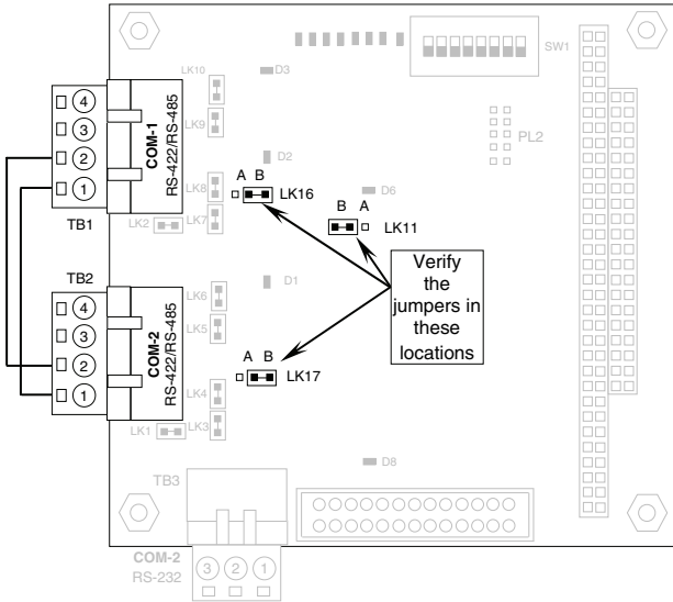
RS-485 Test Configuration
