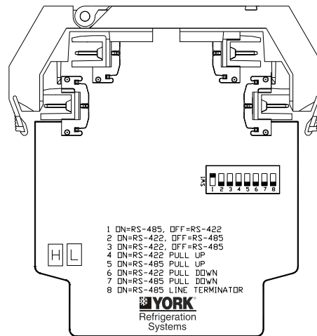
Module circuit board
