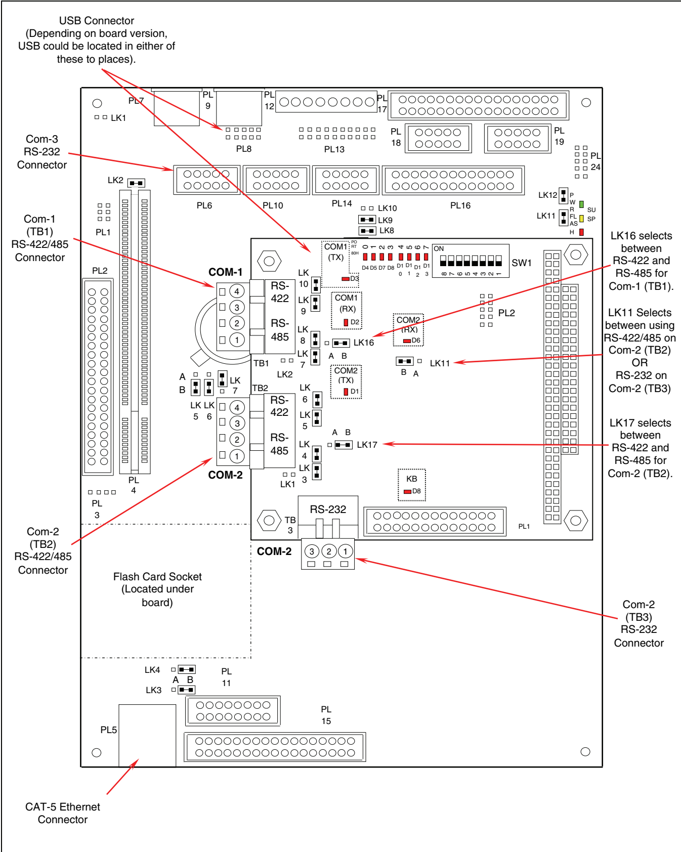
Quantum™ LX Communications Jumpers, connectors and LED locations
