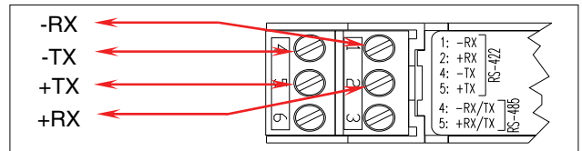
RS-422 Connections
