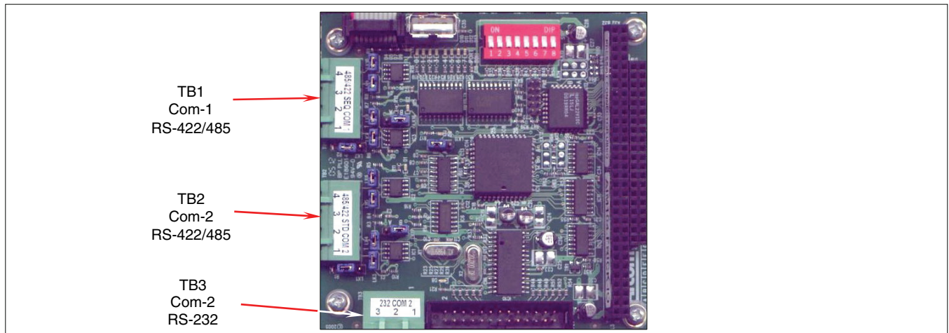
Com-1 and Com-2 Ports on the Daughter Board
