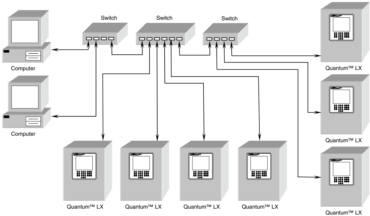
Typical Large Local Quantum™ LX Ethernet Configuration
